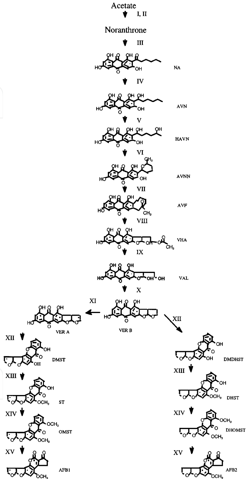
Fig. 1. Biosynthesis of aflatoxins in toxigenic strains of Aspergillus flavus and Aspergillus parasiticus . Adopted from Payne and Brown, 1998. The numbers show the metabolites formed during the biosynthesis.
