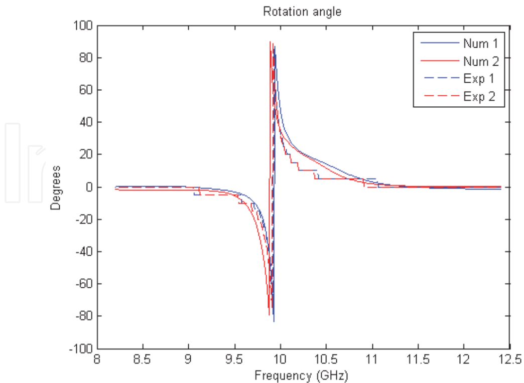
Fig. 13. Rotation of the polarization angle for a plane wave normally incident over a quasi-planar periodic array of right-handed cranks as shown in Figs. 3 and 6: numerical (Num) and experimental (Exp) results. 1 and 2 represent the two possible directions of the propagation wave (incident from front and back side, respectively).
