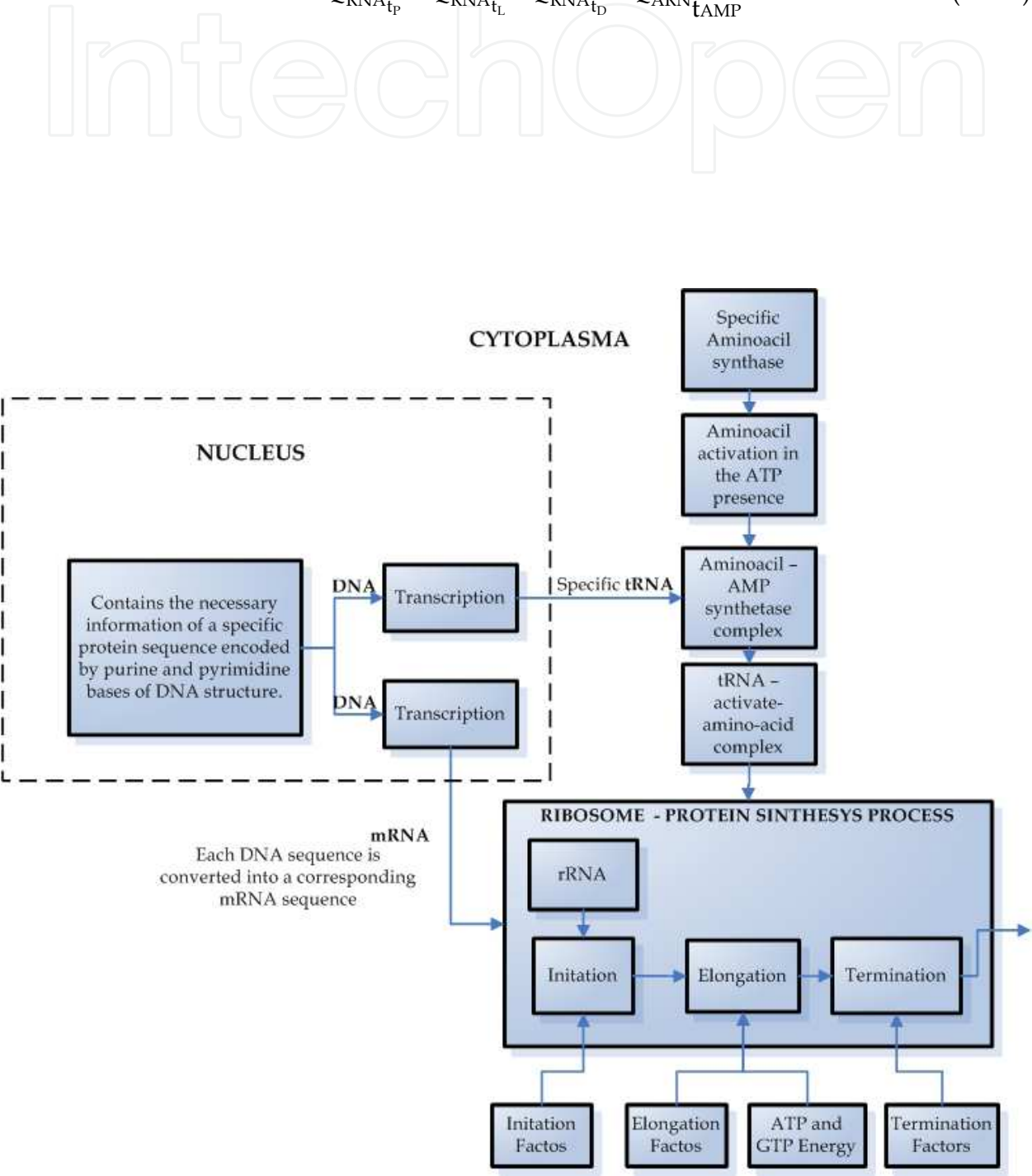
Fig. 4. The multi-compartmental model of protein synthesis process in the neuronal cell
