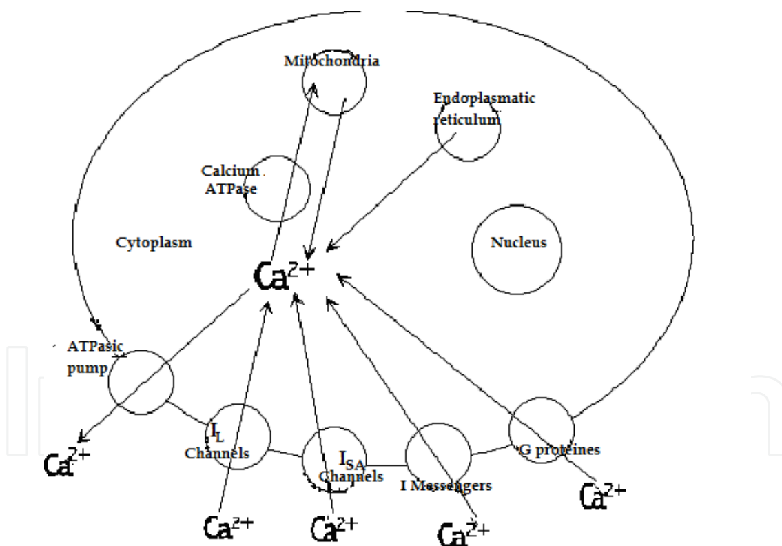
Fig. 6. The states chart for Ca^{2+} inside the neuronal cell in rest state
