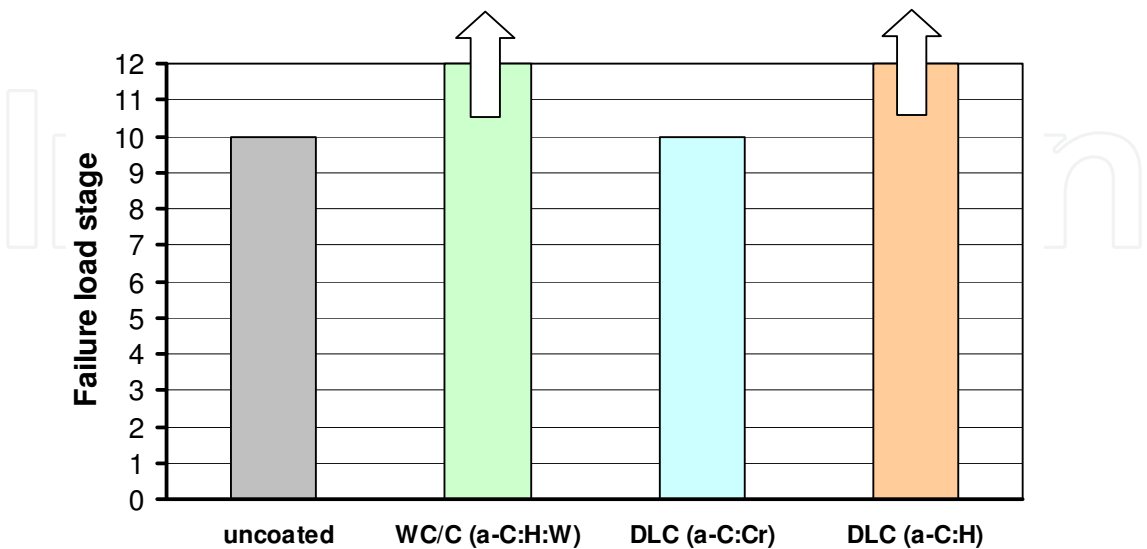
Fig. 13. Failure load stages for uncoated steel gears and for teeth coated with DLC coatings lubricated with eco-oil (A/8.3/90 method)
