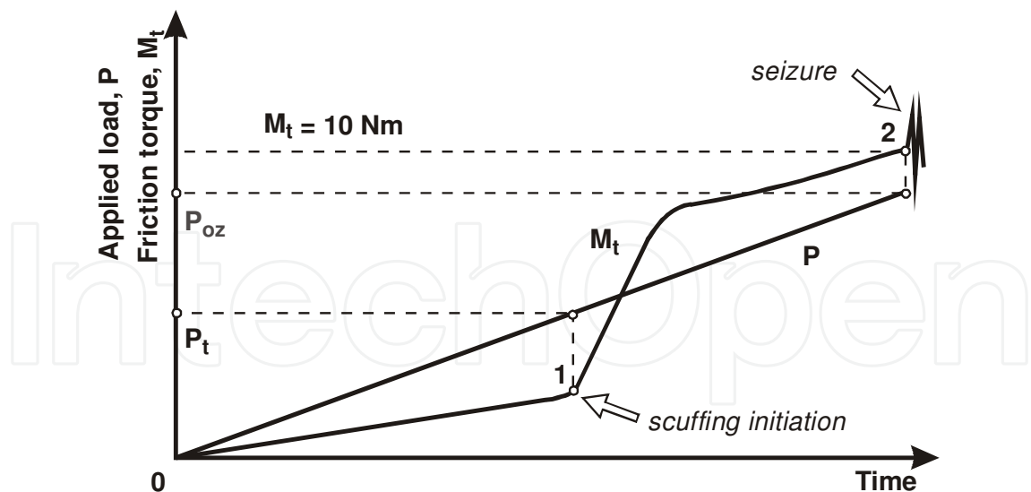
Fig. 5. Simplified friction torque curve ( M_t ) obtained at continuously increasing load ( P ); 1 – scuffing initiation, 1-2 – scuffing propagation, 2 – seizure (exceeding 10 Nm friction torque)
