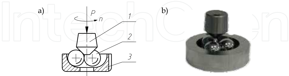
Fig. 8. Cone-three balls tribosystem: a) scheme, b) photograph; 1- cone, 2 - balls, 3 - race
