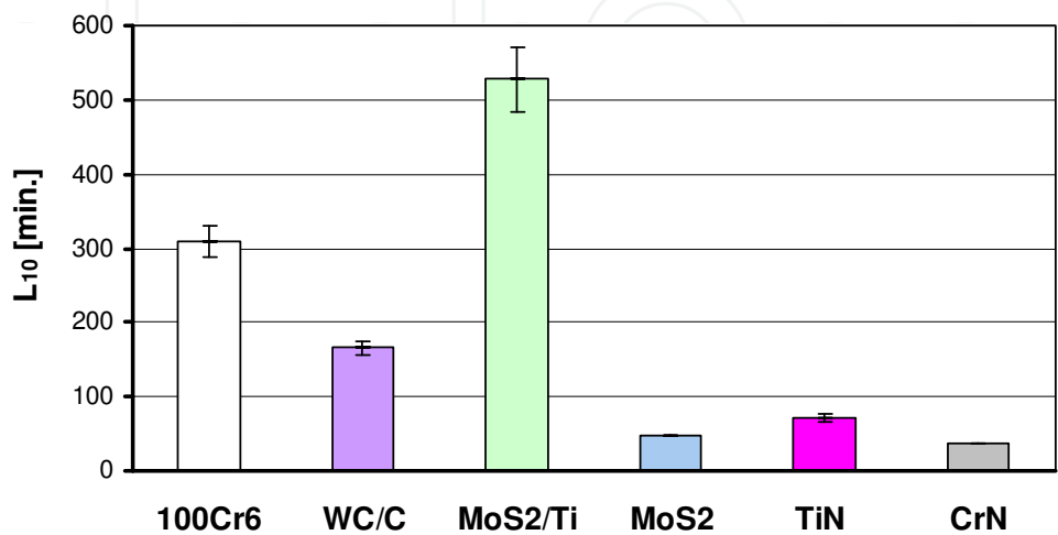
Fig. 9. Results from pitting tests for 100Cr6 steel covered with thin, hard coating
