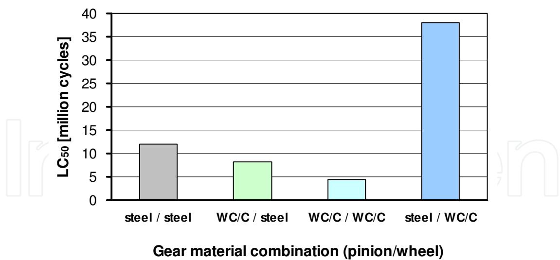
Fig. 16. Fatigue life LC 50 for various pinion/wheel gear material
