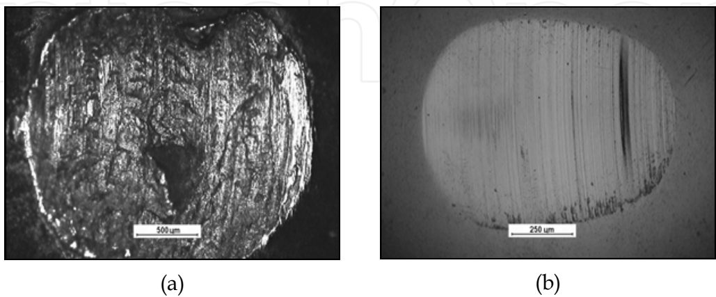
Fig. 7. Wear scars images on lower balls from scuffing tests for: a) steel-steel, b) CrN-CrN (four ball test, mineral base oil without lubricating additives)
