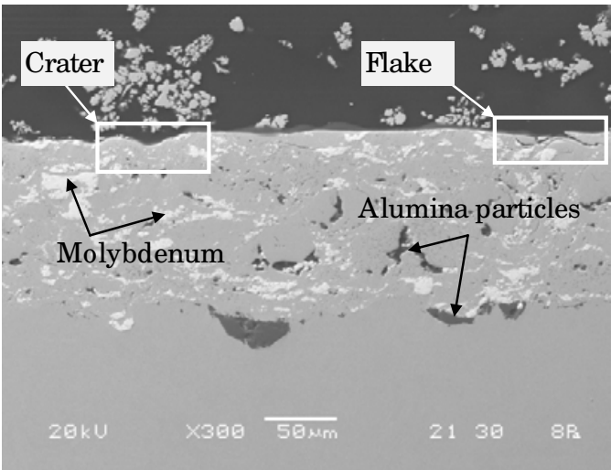
Fig. 3. NiCrBSi + SP+ G coating
