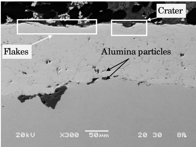
Fig. 4. Al Bronze + SP+ G coating
