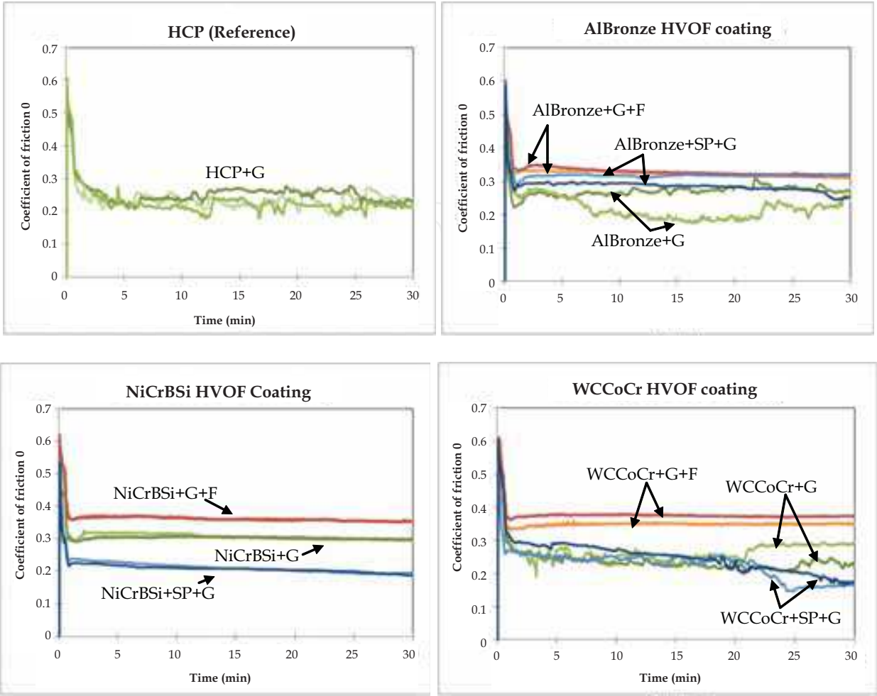
Fig. 6. Friction curves
