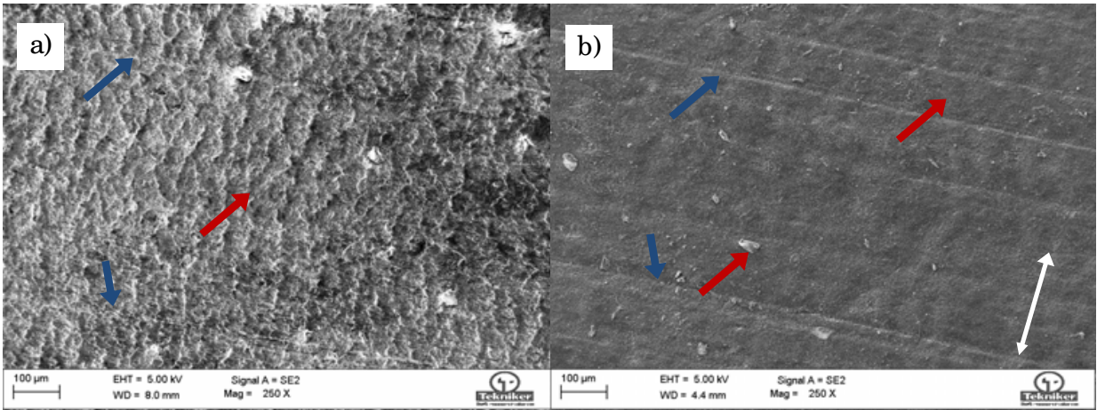
Fig. 8. Not tested area on the NBR elastomeric samples (a) and worn area after tests againts HCP+G reference material (b). White arrow indicates sliding direction. Blue arrows indicate straigh marks from the mould. Red arrows indicate points where X-Ray analysis was done
