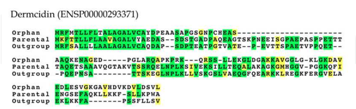
Fig. 2. Alignment of dermcidin (orphan), human lacritin (parental) and cat lacritin (outgroup) proteins. Identical residues are in green, similar residues in yellow.
