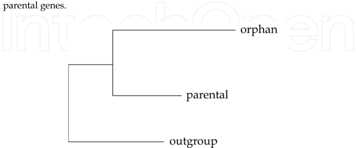
Fig. 1. Tree topology corresponding to gene families containing duplicated orphan genes. The orphan and parental genes are from human, the outgroup gene from a non-primate species.
