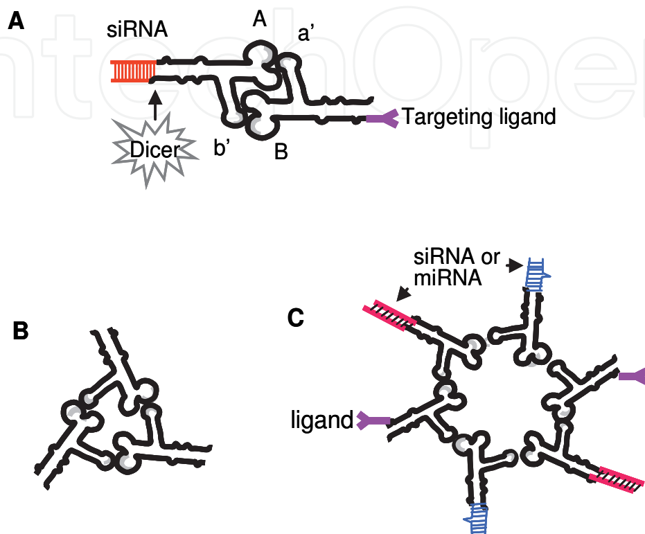
Fig. 3. Structural schematic of packaging RNA (pRNA) multimers as a drug targeted delivery vehicle. (A) pRNA dimer forms through the base-pairing between the loops of an A' b-pRNA-siRNA and a B' a-pRNA-ligand. The shaded areas on the loops indicate the base-pair interactions between the monomers. siRNA is released when intracellular Dicer cleaves the dsRNA, which is indicated by an arrow. (B) pRNA trimers can be stoichiometrically formed by hand-in-hand loop interactions, which contains 1:1:1 of their linked conjugates. (C) hexamers allow for a customizable, combined therapy where multiple drugs may be added to the same complex.
