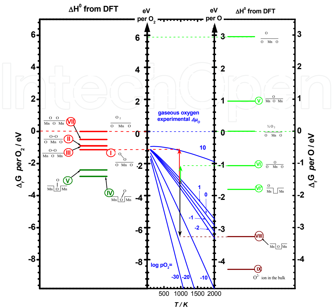
Fig. 6. Spectrum of possible “one-particle” states, where “particles” are O atoms (right panel) and O 2 molecules (left panel). Each level in these panels corresponds to relative energies ( \Delta E_r ) of different molecular and atomic species occurring during oxygen incorporation reaction on the MnO 2 [001]-terminated surface of LaMnO 3 , cf. Table 5. The axes on the left and right give the energy \Delta E_r relative to resting O 2 molecule away from the surface (on the left) or an atom in such O 2 molecule (on the right). In the ground state of the crystal all lattice sites in crystal bulk (states X) and I surface (states VIII) are occupied (red levels) and the rest of the “one-particle” states vacant. The numbers at levels correspond to the numbers assigned to respective states in Table 5. The highest level on the right panel corresponds to a free (not in a molecule) O atom away from the crystal. The central panel shows the experimental T - and p_{O_2} -dependence of the Gibbs energy of gaseous O 2 (Table 1 and Eq.(50)), its energy scale refers to an O 2 molecule on the left and to an O atom in an O 2 molecule on the right. The labels m on the lines represent the pressure: p_{O_2}=10^m atm. The arrows indicate various Gibbs reaction energies due to moving of a “particle” between crystal and gas: red = formation of adsorbed superoxide O 2 - on defect-free surface; green = formation of adsorbed O- atop Mn on defect-free surface; black = incorporation of oxygen into a surface oxygen vacancy.
