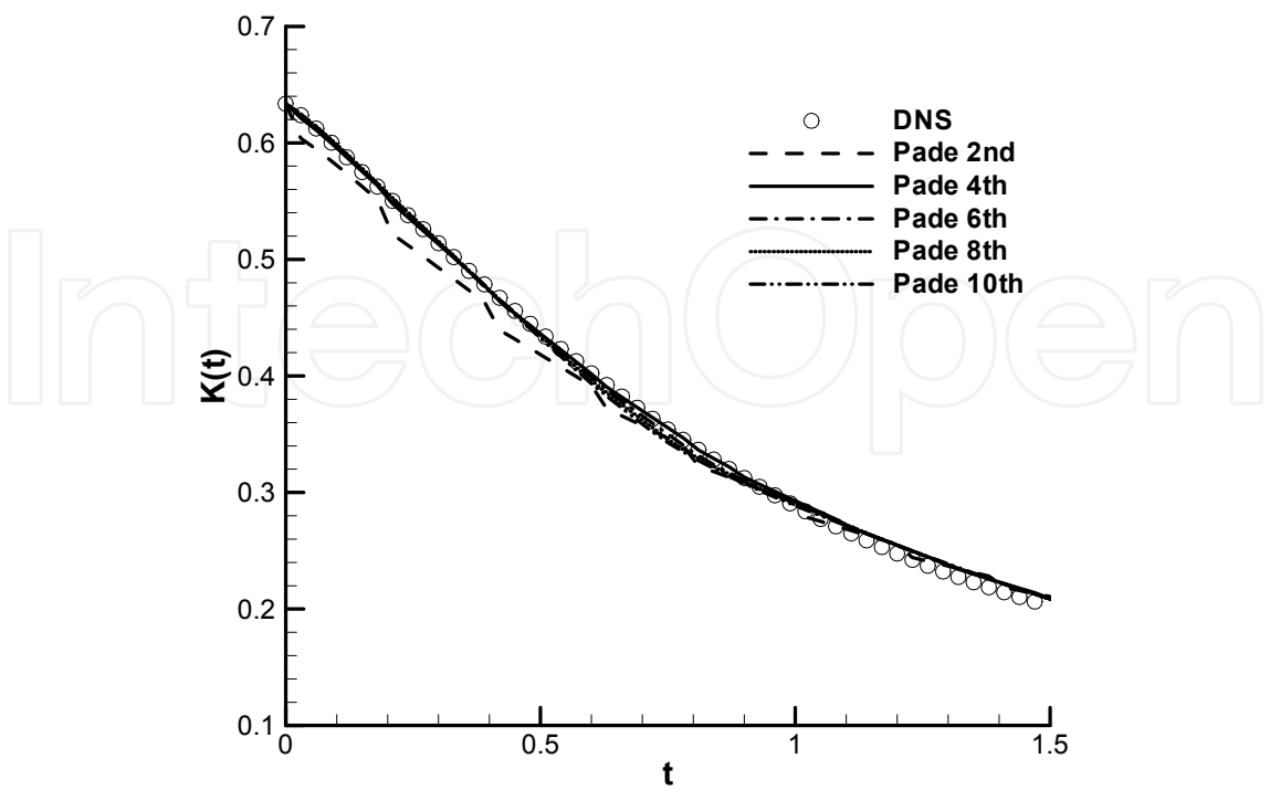
Fig. 4.12. The decay of the total kinetic energy for the Padé filters.
