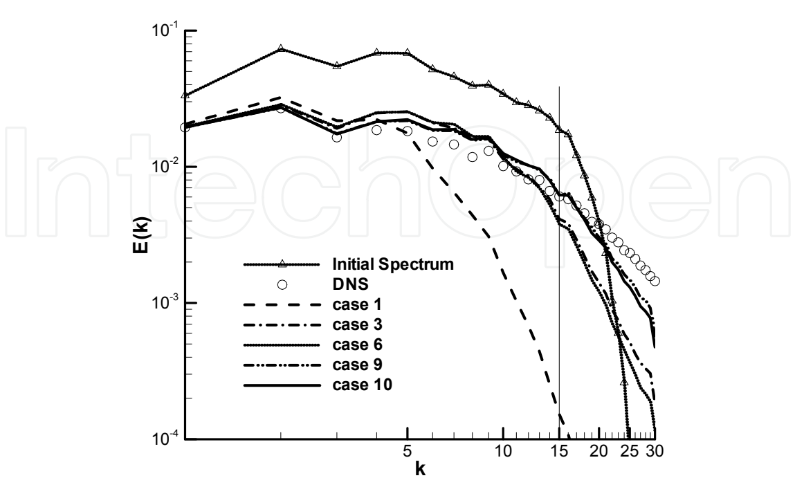
Fig. 4.8. Energy spectrum at final time for the V-filters.
