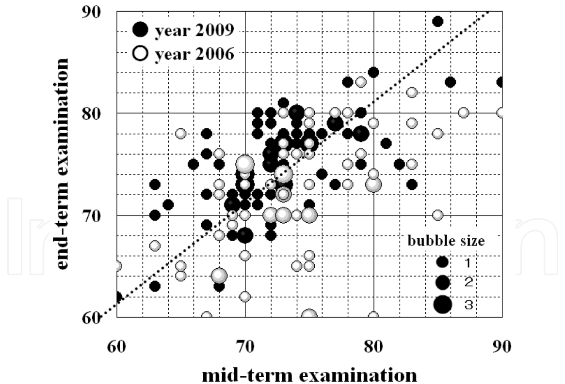
Fig. 3. distribution of s_m and s_f . The bubble size shows the number of person who got the score pair. Through the experience, we show the change of the students' skill between mid-term examination and the end-term examination ((Nakahira et al., 2010a;b)). To examine how
