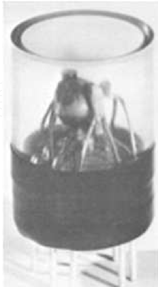
Fig. 2. The first radioisotope thermoelectric generator (RTG).
