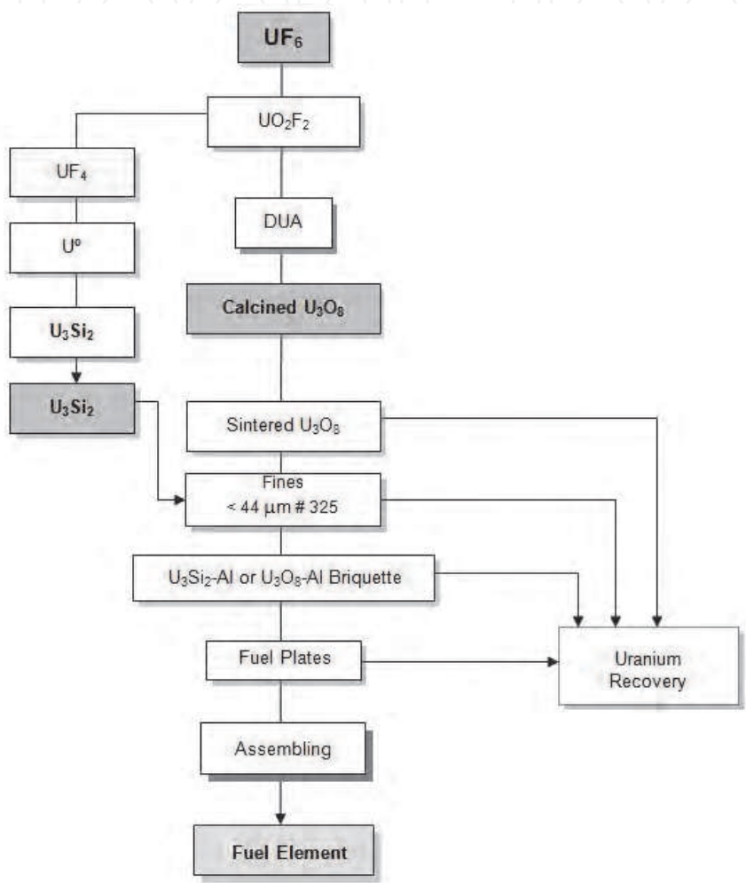
Fig. 10. Fabrication process of silicide fuel elements.
