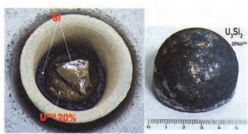
Assembling of U 3 Si 2 crucible load
