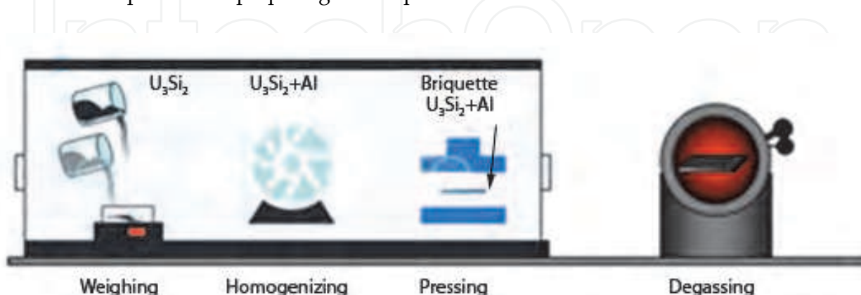
Fig. 11. Process for briquettes preparation and degassing.
