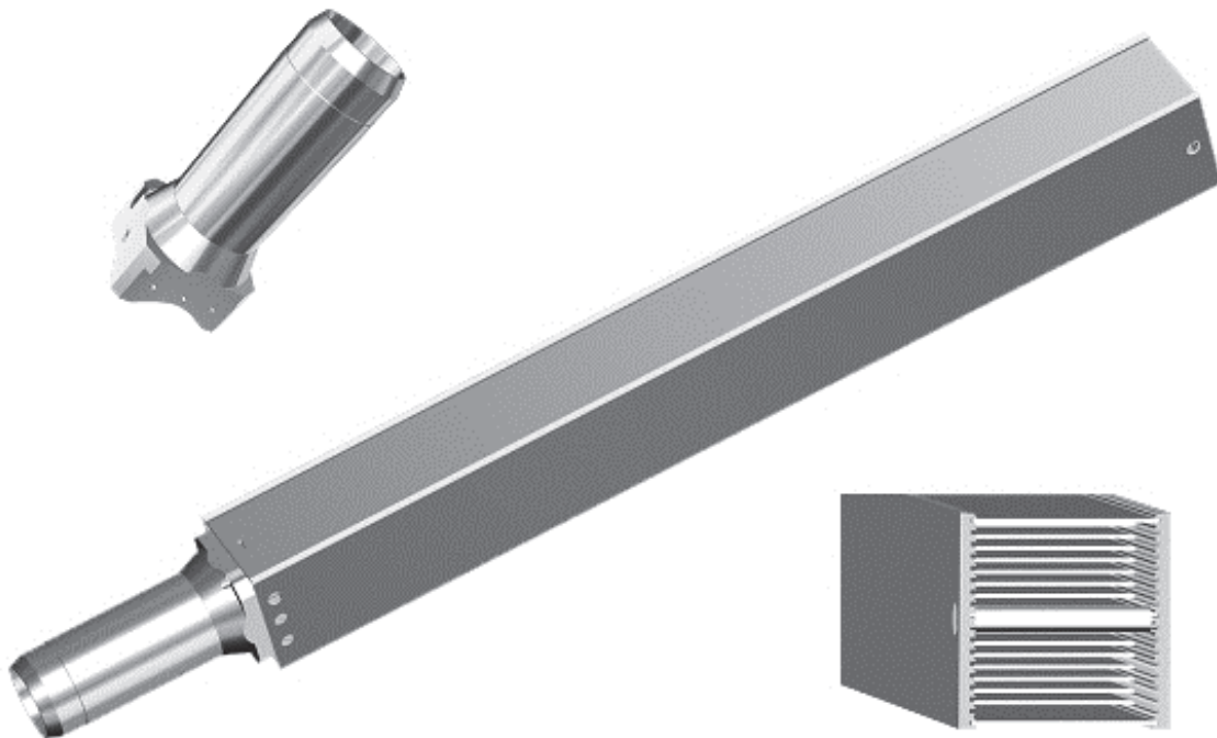
Fig. 16. Schematic illustration of the fuel element produced at IPEN.
