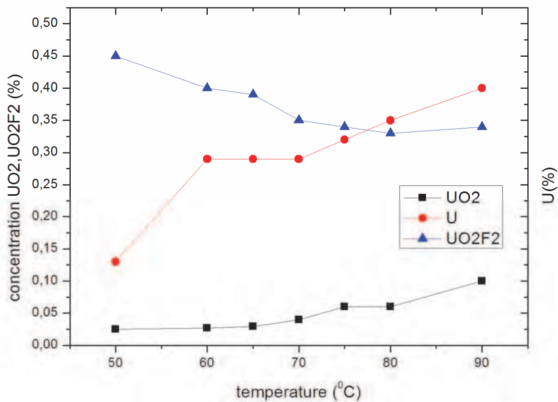
Fig. 4. Influence of the temperature as a function of the contents of UO 2 F 2 and UO 2 in UF 4
