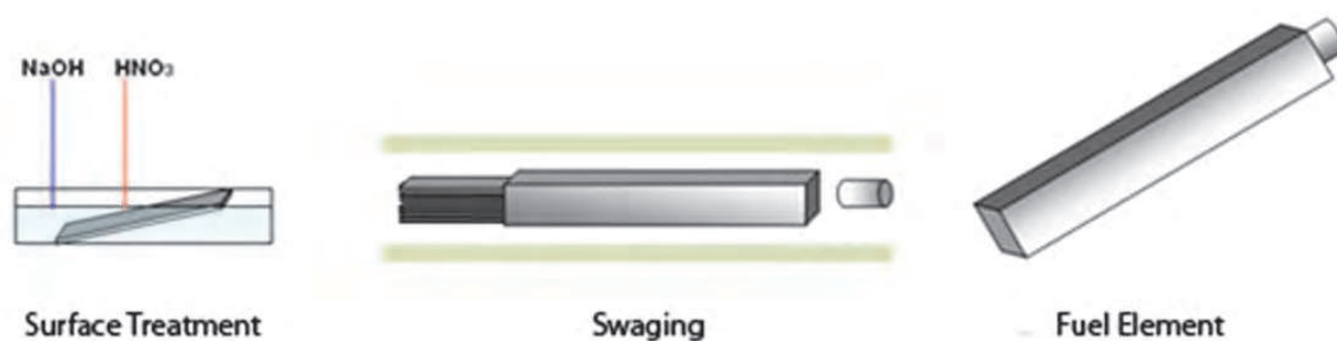
Fig. 15. The process of assembling the fuel elements.
