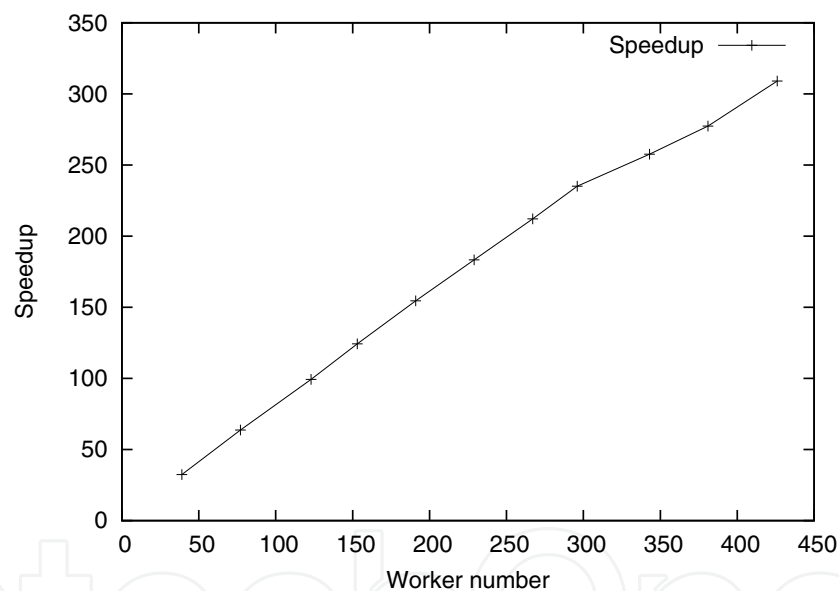
Fig. 3. Speedup factor
