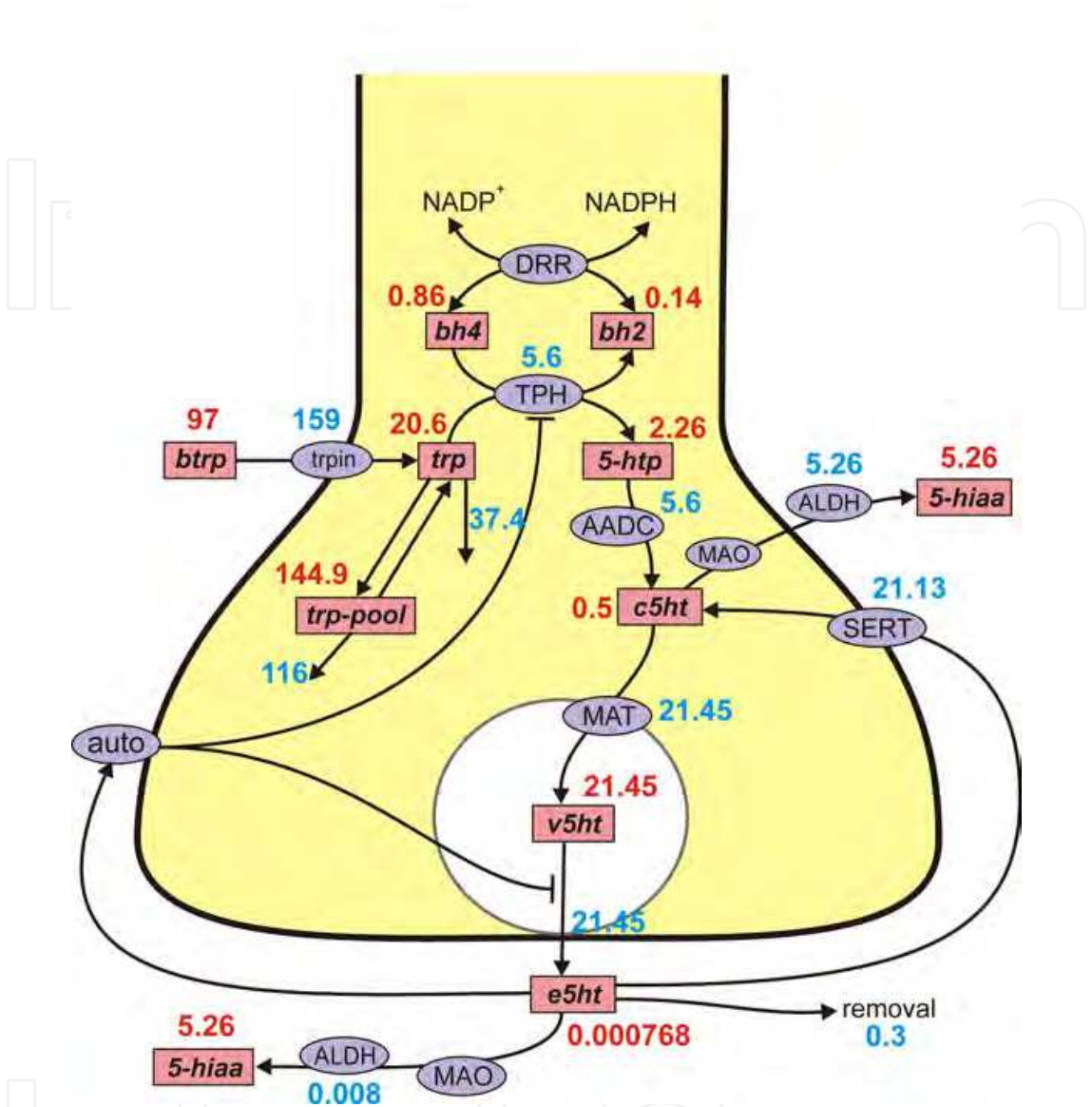
Fig. 1. Steady state concentrations and fluxes in the 5-HT terminal model. The figure shows the reactions in the model. The pink rectangular boxes indicate substrates and blue ellipses contain the acronyms of enzymes or transporters; steady state values in the model are indicated. Concentrations (red) have units of \mu\text{M} and rates (blue) have units of \mu\text{M}/\text{hr} . Full names of the substrates are: bh2, dihydrobiopterin; bh4, tetrahydrobiopterin; trp, tryptophan; btrp, serum tryptophan; 5htp, 5-hydroxytryptophan; c5ht, cytosolic 5-HT; v5ht, vesicular 5-HT; e5ht; extracellular 5-HT; 5-hiaa, 5-hydroxyindoleacetic acid; trp-pool , the tryptophan pool. Names of enzymes and transporters are: Trpin, neutral amino acid transporter; DRR, dihydrobiopterin reductase; TPH, tryptophan hydroxylase; AADC, aromatic amino acid decarboxylase; MAT, vesicular monoamine transporter; SERT, 5-HT reuptake transporter; auto, 5-HT autoreceptors; MAO, monoamine oxidase; ALDH, aldehyde dehydrogenase. Removal means uptake by capillaries or glial cells or diffusion out of the system.
