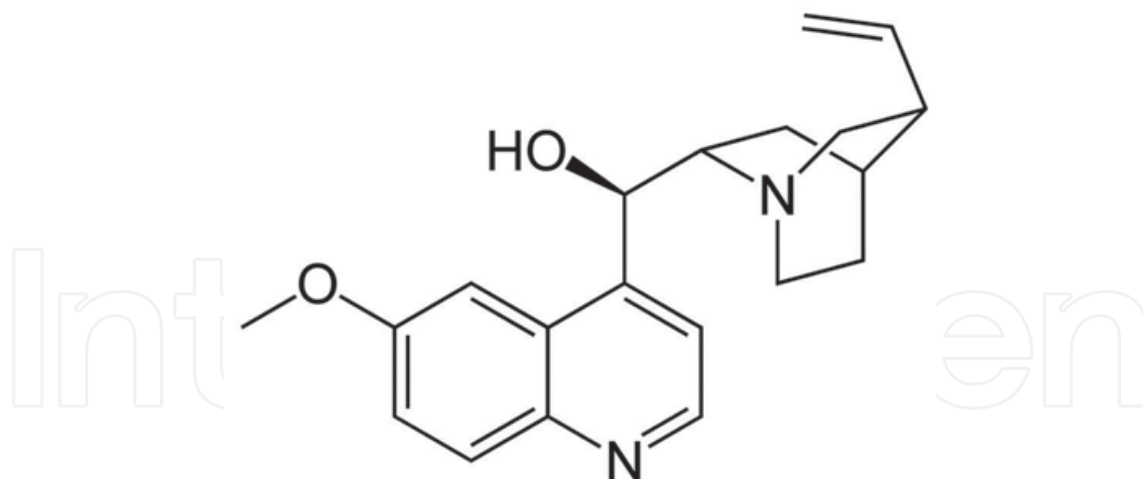
Fig. 5. Structure of quinidine
