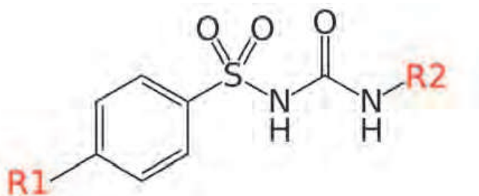
Fig. 2. Structure of the sulfonylureas
