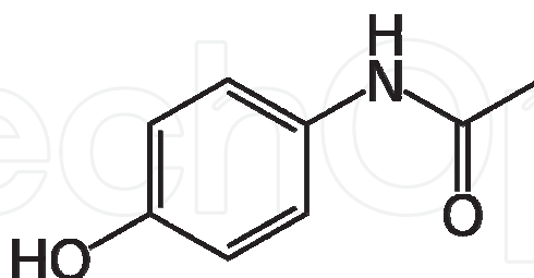
Fig. 3. Structure of the paracetamol (acetaminophen)
