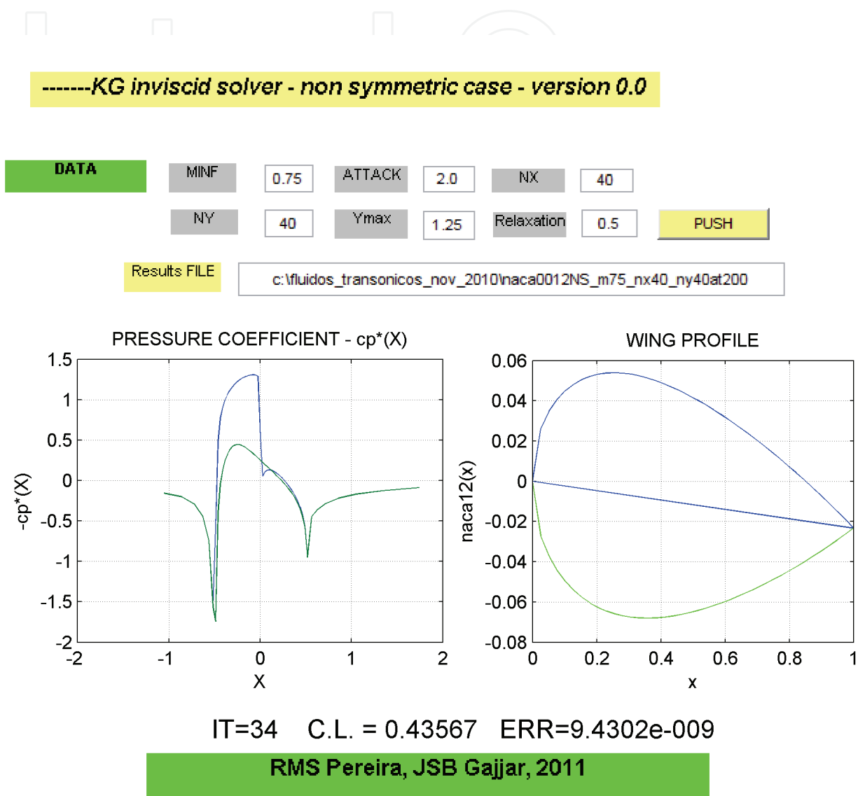
Fig. 8. Example of results for KG code for Transonic flows where M_{inf} = 0.75; \alpha = 2.0; Nx = 40, Ny = 40, relaxation = 0.5 .
