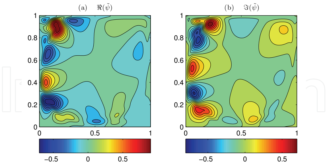
Fig. 3. Eigenfunctions of the streamfunction for lid-driven cavity at a critical Reynolds number of Re = 8026.7 and aspect ratio A = 1 .
