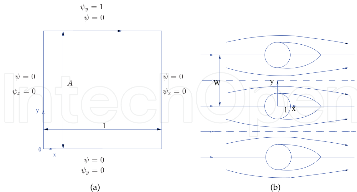
Fig. 2. Sketch of (a) the lid-driven cavity with boundary conditions, and (b) flow past a row of circular cylinders.
