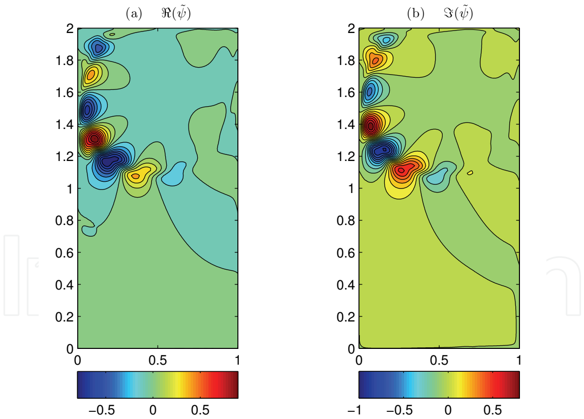
Fig. 4. Eigenfunctions of the streamfunction for lid-driven cavity at a critical Reynolds number of Re = 5861 and aspect ratio A = 2 .
