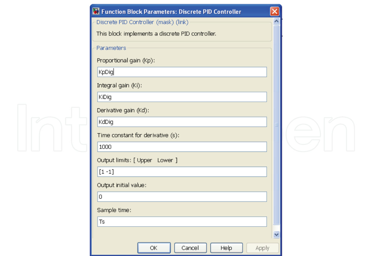
Fig. 7. Configuration Window Discrete PID
