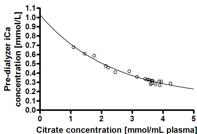
Fig. 2. Pre-dialyzer ionized calcium (iCa) concentration plotted against plasma citrate concentration.
