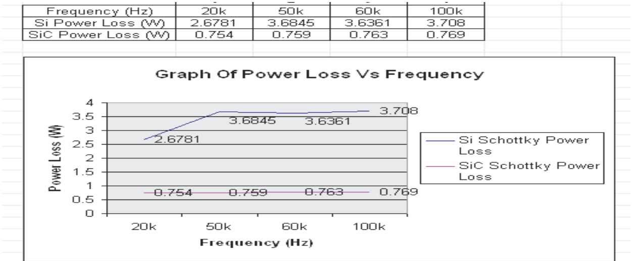
Fig. 21. Graph of Power Loss vs Frequency of Silicon Schottky and Silicon Carbide Schottky Diode
