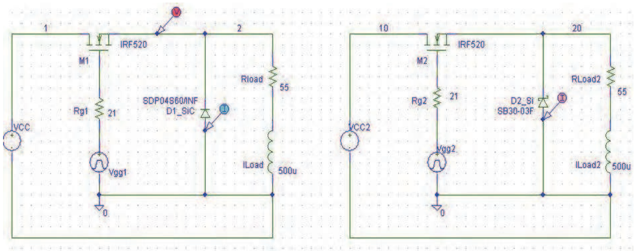
Fig. 5. Inductive Load Chopper Circuit
