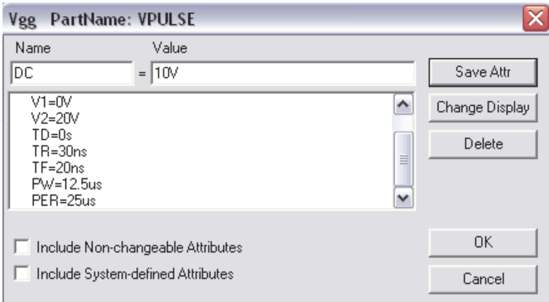
Fig. 6. V_{pulse} Setting
