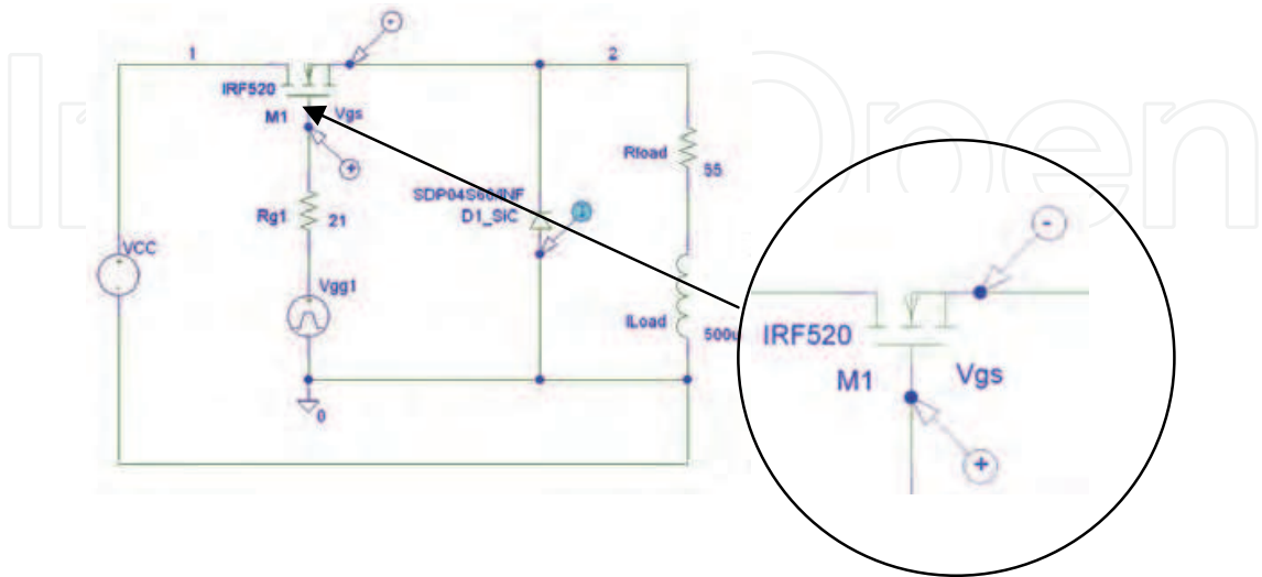
Fig. 8. Finding V_{gs} of Silicon Schottky and Silicon Carbide Schottky diode using voltage differential probe.
