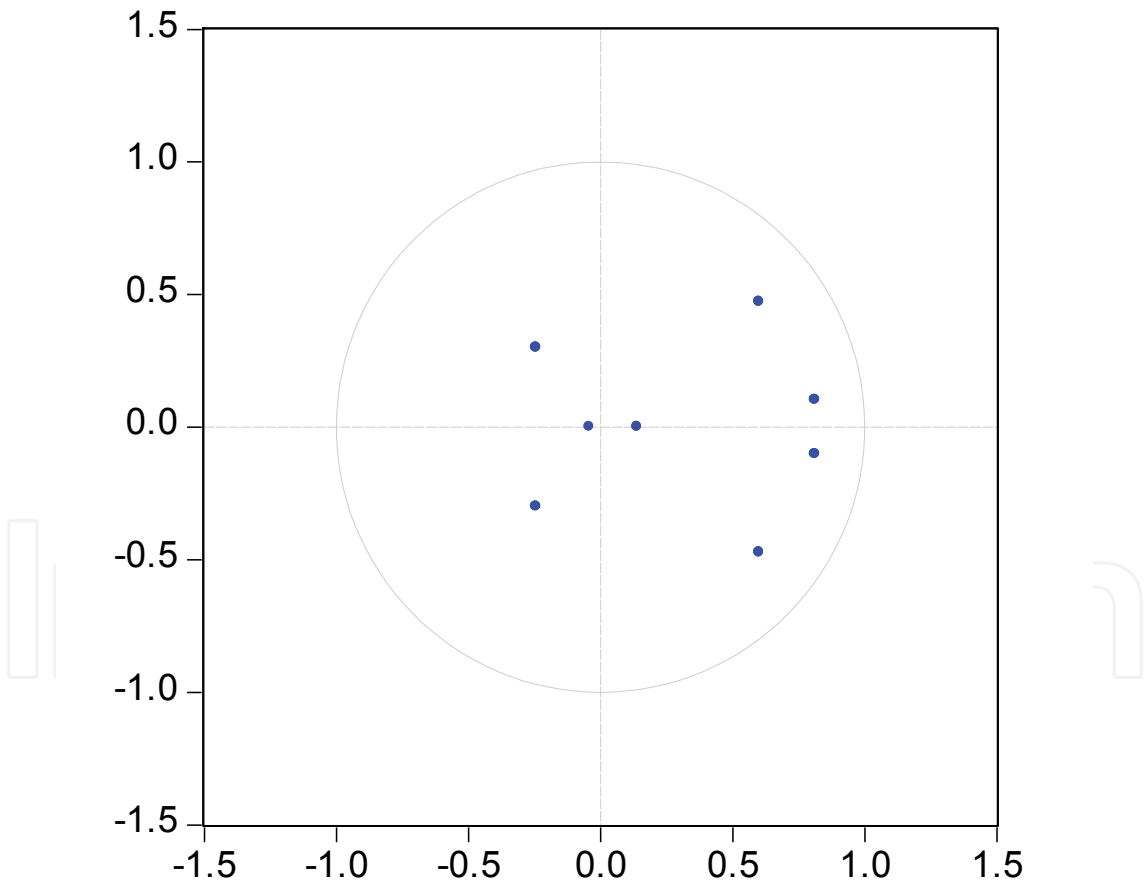
Inverse Roots of AR Characteristic Polynomial
