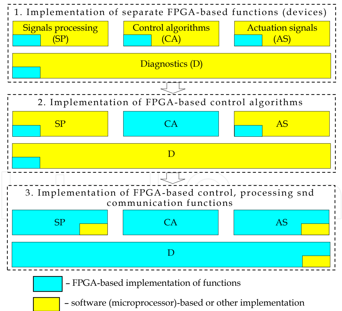
Fig. 1. Application of FPGA technology in the NPP I&Cs produced by RPC Radiy
