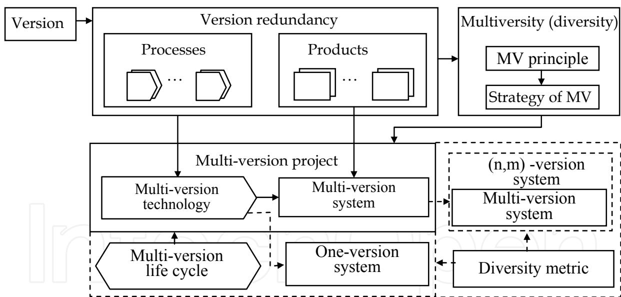
Fig. 3. Taxonomy scheme of multi-version computing
