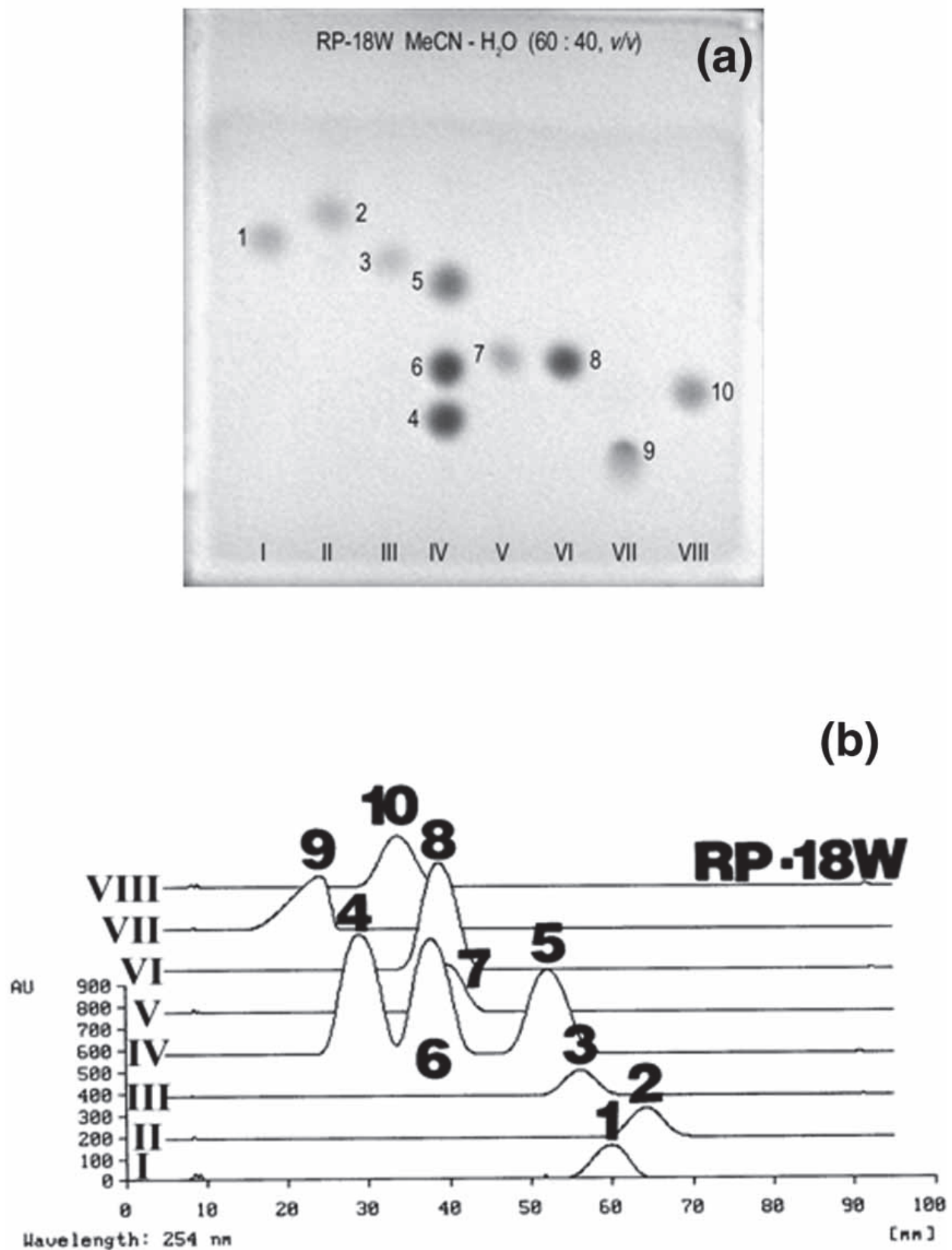
Fig. 4. Videoscan (a) and densitogram (b) of the RP-18W plate, which shows separation of eight fractions of mixture of 10 pesticides (5 \mu L of each fraction) by RP system: acetonitrile-water (60 : 40, v/v) (From Tuzimski, 2005a. With permission.).
