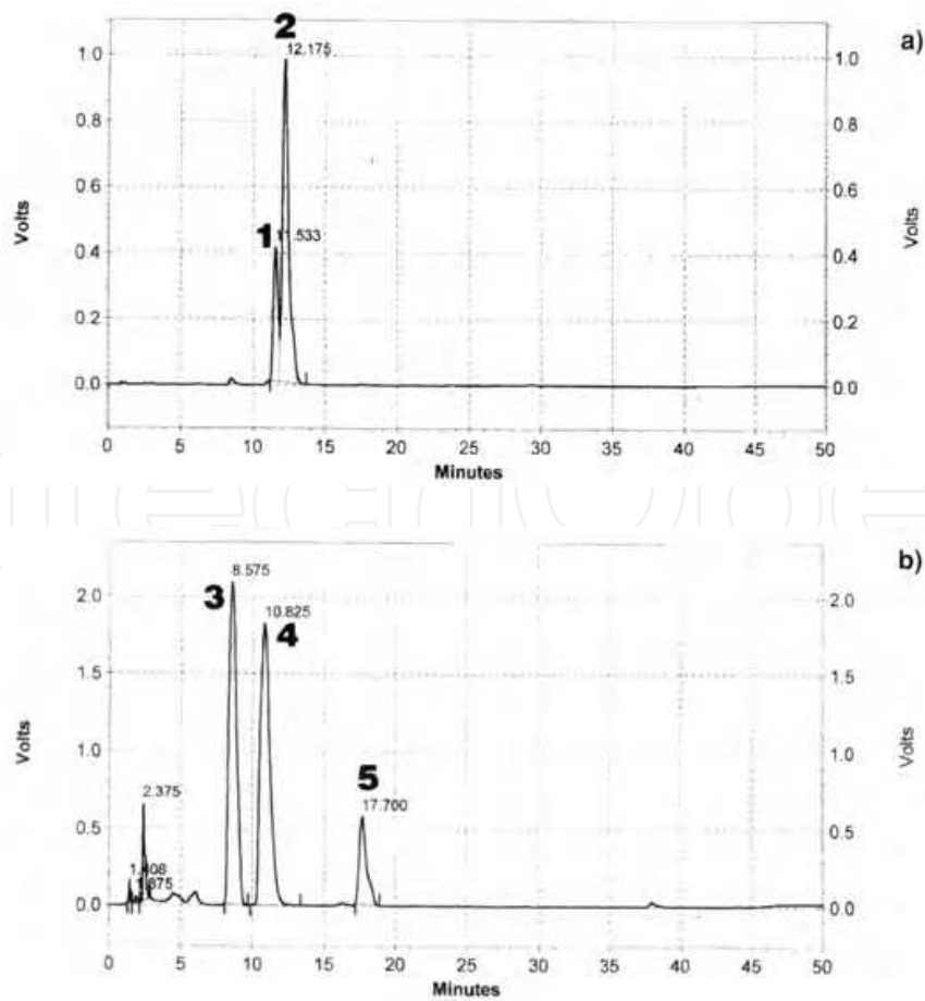
Fig. 10. HPLC separation of the ten-component pesticide mixture on a 150 mm × 4.6 mm, dp = 5\text{ }\mu\text{m} , Supelcosil LC-18 column (Supelco) by use of a methanol-water gradient (50 to 85% methanol from 0–50 min). The flow rate was 1.0 mL min -1 , detection was at 254 nm, and the temperature was 22 ± 1°C. (From Tuzimski, 2005b. With permission.).
