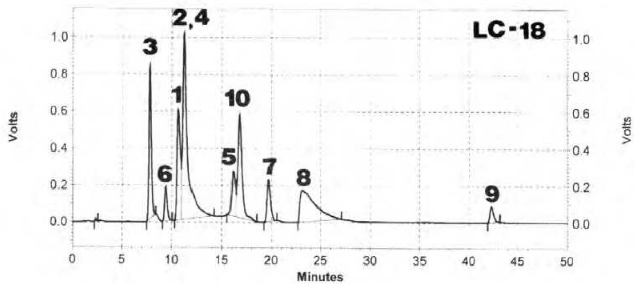
Fig. 10. HPLC separation of the ten-component pesticide mixture on a 150 mm × 4.6 mm, dp = 5\text{ }\mu\text{m} , Supelcosil LC-18 column (Supelco) by use of a methanol-water gradient (50 to 85% methanol from 0–50 min). The flow rate was 1.0 mL min -1 , detection was at 254 nm, and the temperature was 22 ± 1°C. (From Tuzimski, 2005b. With permission.).
