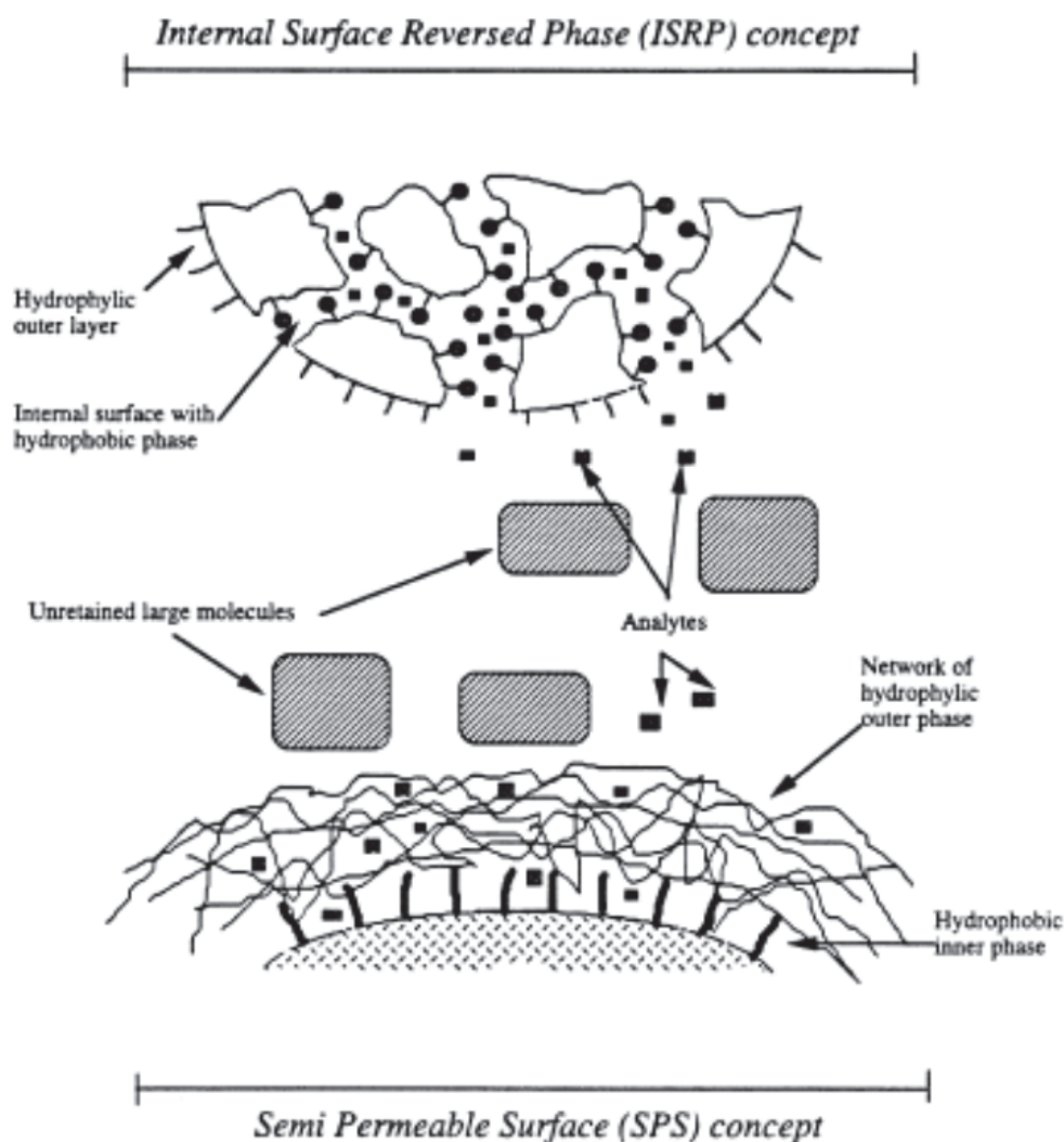
Fig. 5. Schematic representation of the principle of restricted access materials (Poole, 2003).
