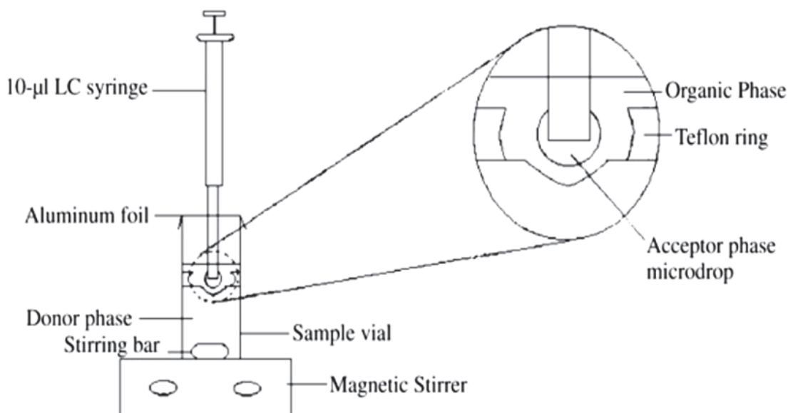
Fig. 2. Schematic representation of dynamic single drop microextraction (DSDME) (Lambropoulou, 2007).
