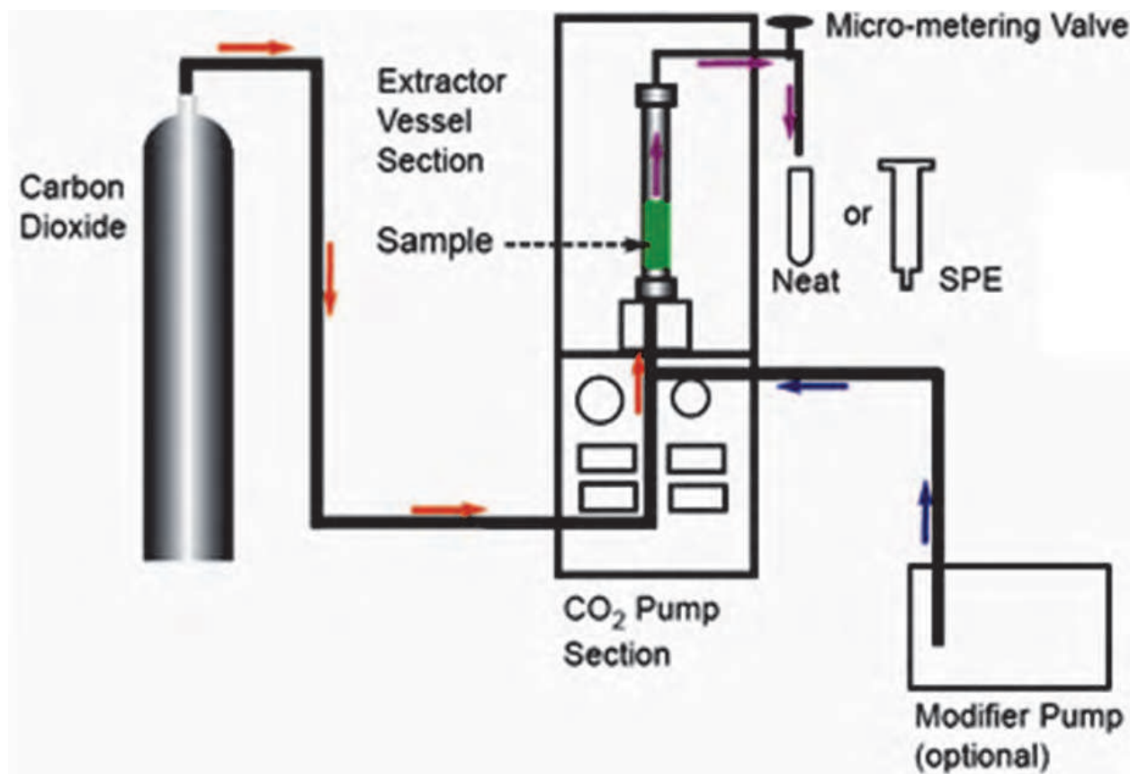
Fig. 8. Diagram of a Spe-ed™ Prime SFE by Applied Separations Inc. (2008)
