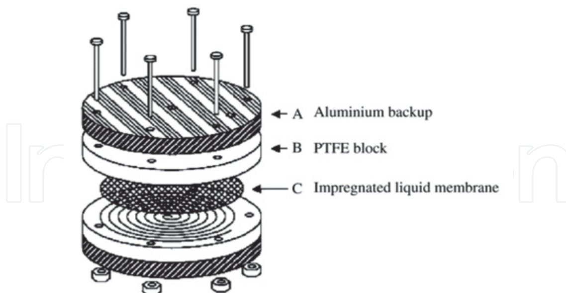
Fig. 4. Schematic diagram of a supported liquid membrane extraction (SLME).
