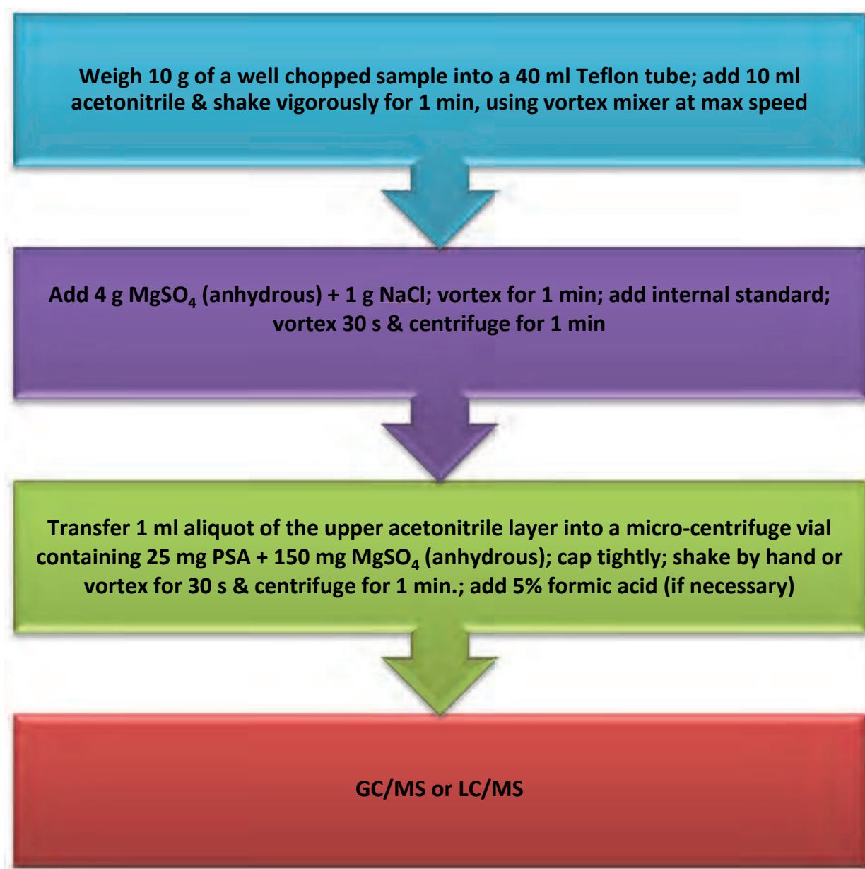
Scheme 1. The main steps in the QuEChERS protocol.
