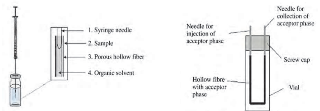
Fig. 3. Schematic representation of rod and U-shaped porous hollow fiber membranes.
