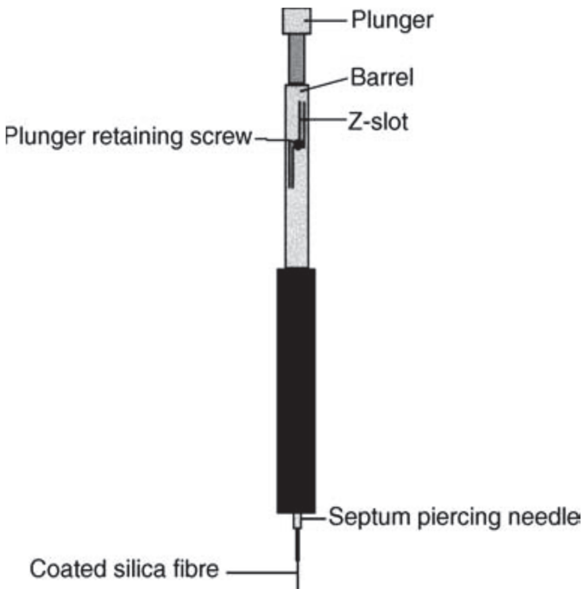
Fig. 6. Schematic diagram of a SPME device (King et al., 2003).
