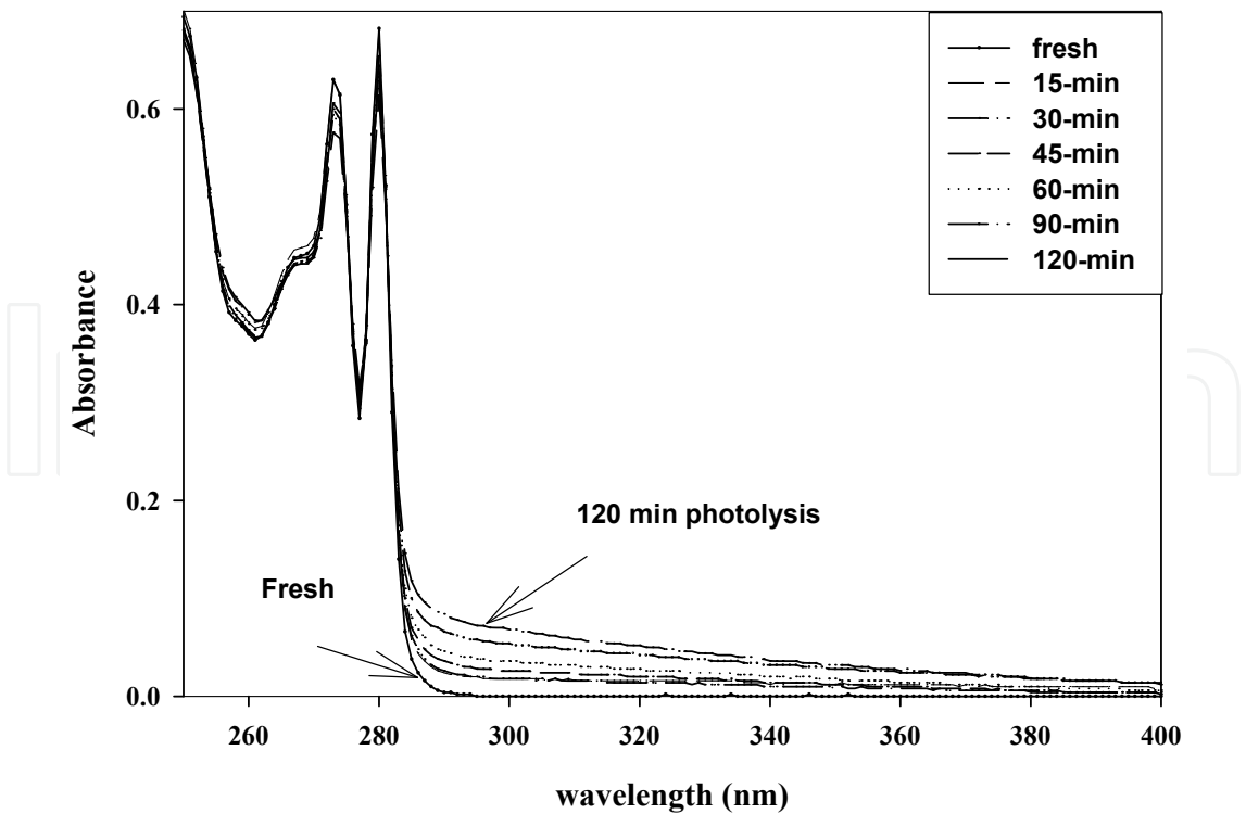
Fig. 5. UV absorption spectra of fresh and photolyzed samples of 1 \times 10^{-4} M solutions of benzimidazole in acetonitrile solvent.
