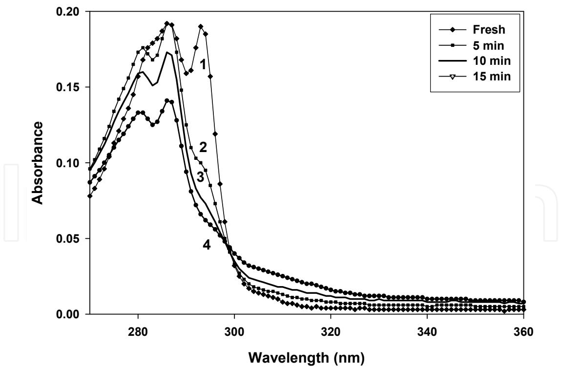
Fig. 8. UV absorption spectra of fresh and photolyzed samples of 0.5\times10^{-4}\text{M} solutions of carbendazim in acetonitrile solvent, (1) fresh, (2) 5 min, (3) 10 min, (4) 15 min photolysis periods.
