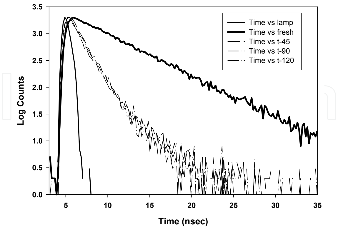
Fig. 7. Fluorescence decay time of fresh and photolyzed samples of 1\times10^{-4}\text{M} solutions of benzimidazole in acetonitrile solvent excited at 280 nm.
