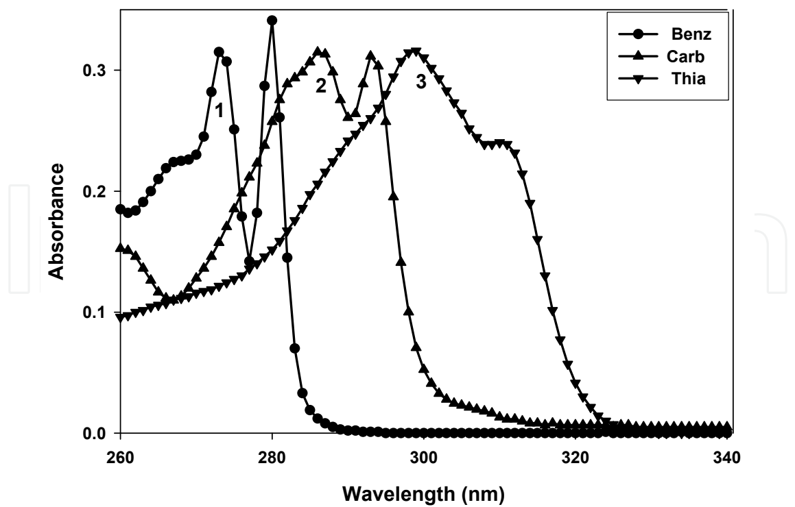
Fig. 2. UV absorption spectra of fresh samples of 1 \times 10^{-4} M solutions (1) benzimidazole, (2) carbendazime, (3) thiabendazole in acetonitrile solvent.
