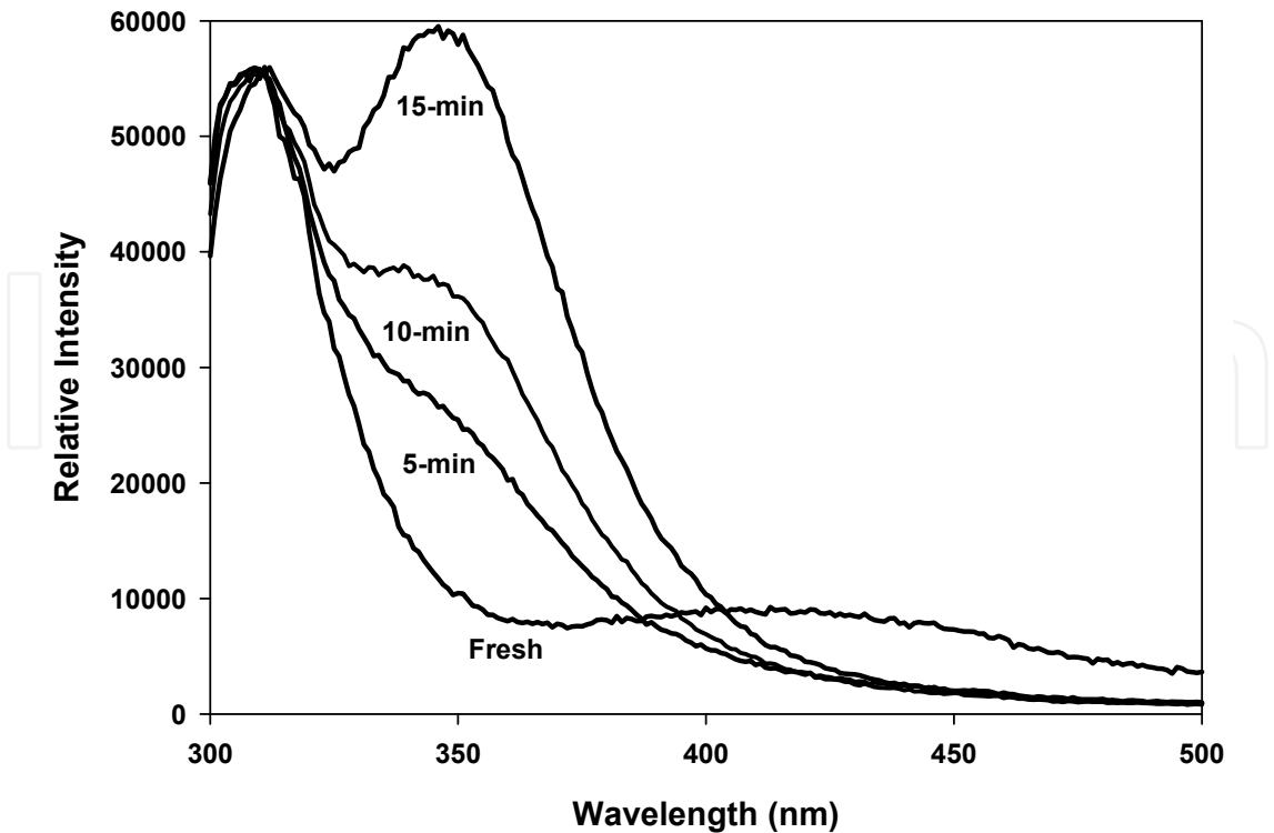
Fig. 9. Normalized fluorescence spectra of fresh and photolyzed samples of 0.5 \times 10^{-4} M solutions of carbendazim in acetonitrile solvent excited at 300 nm.
