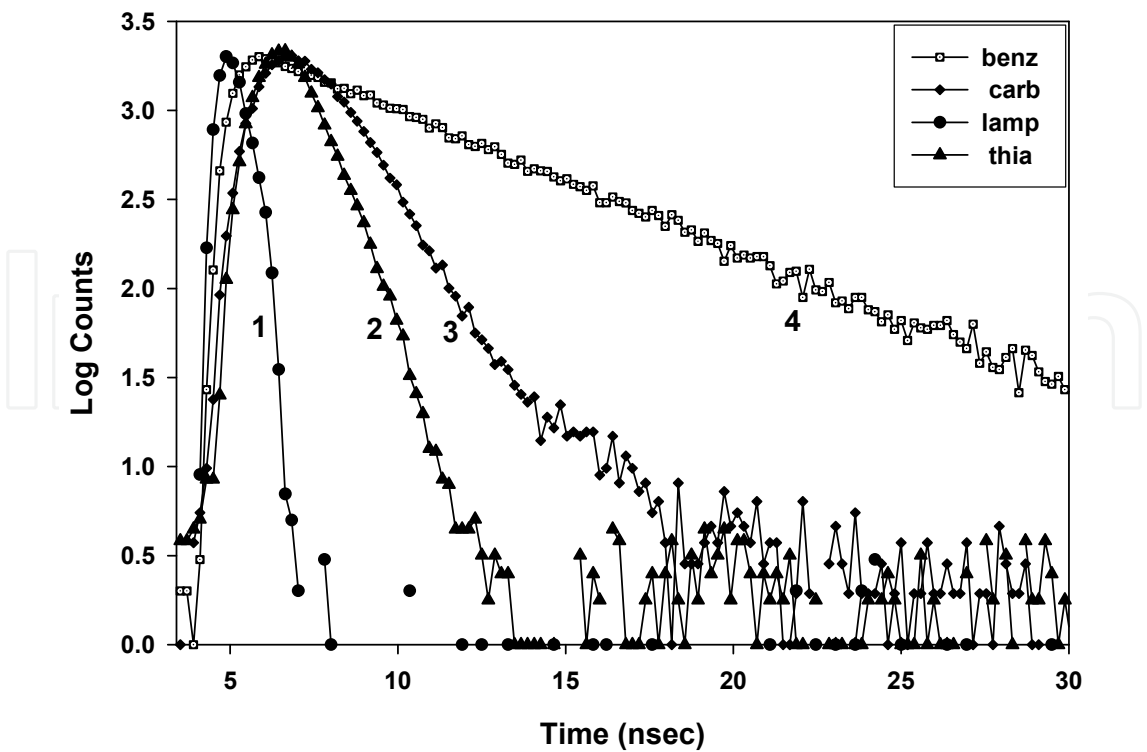
Fig. 4. Decay time curves for a fresh samples of \approx 10^{-4} M solutions, (1) lamp pulse decay, (2) thiabendazole, (3) carbendazime, (4) benzimidazole in acetonitrile solvent. Excitation and fluorescence bands correspond to those obtained from the absorption and emission maxima.
