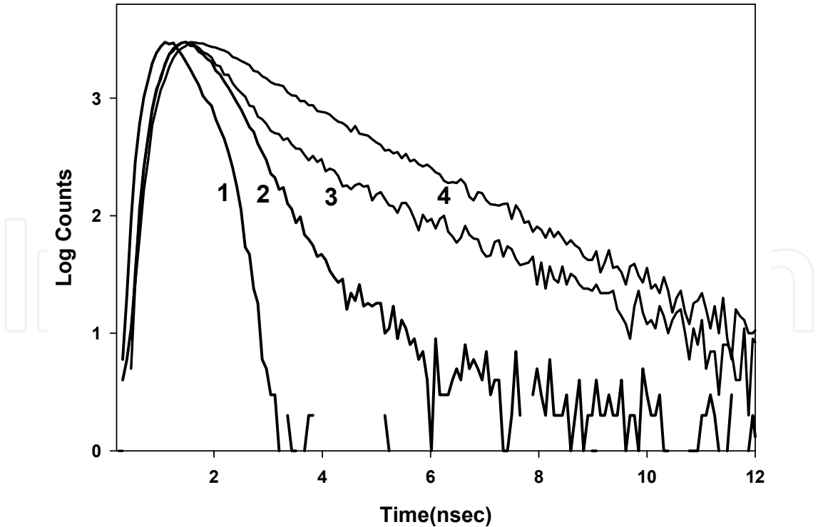
Fig. 10. Fluorescence decay time of fresh and photolyzed samples of 0.5 \times 10^{-4} M solutions of carbendazim in acetonitrile solvent excited at 300 nm. (1) lamp, (2) Fresh, (3) 10 min, (4) 20 min photolysis time.
