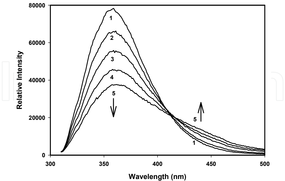
Fig. 12. Fluorescence spectra of fresh and photolyzed samples of 1.5 \times 10^{-4} \text{M} solutions of thiabendazole in acetonitrile solvent excited at 300 nm. (1) fresh, 2 5 min, (3) 10 min, (4) 15 min, (5) 20 min photolysis periods
