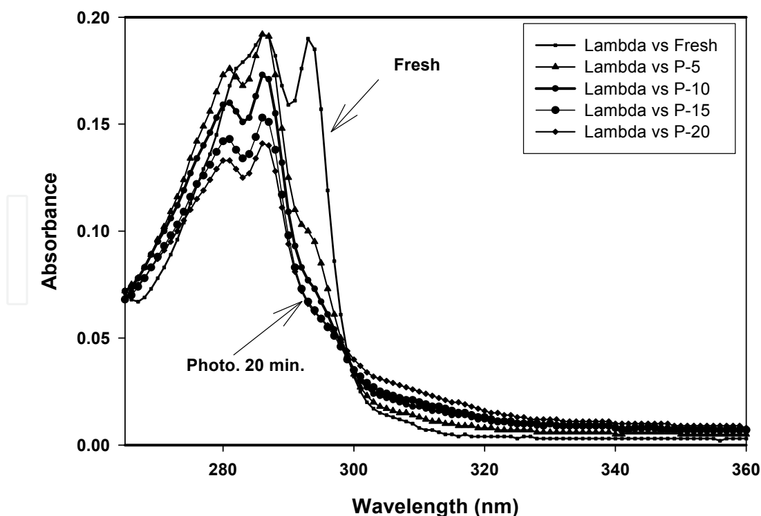
Fig. 11. UV absorption spectra of fresh and photolyzed samples of 1.5 \times 10^{-4} M solutions of thiabendazole in acetonitrile solvent.
