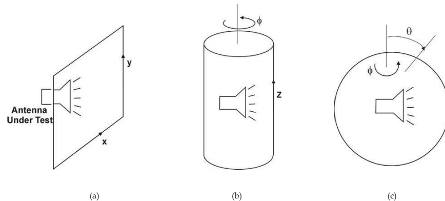
Fig. 2. Canonical near-field scan configurations: (a) planar, (b) cylindrical, (c) spherical.
