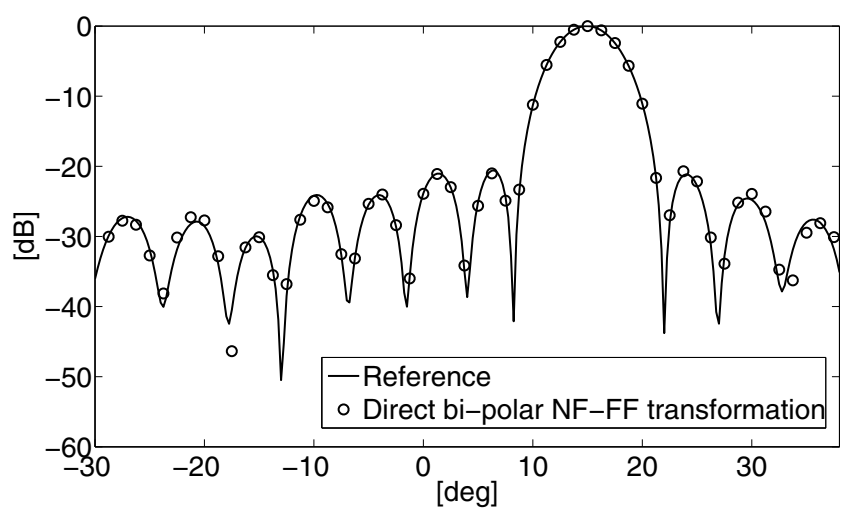
Fig. 11. Co-polarized H-plane pattern for a 21x21 dipole array with Taylor illumination.
