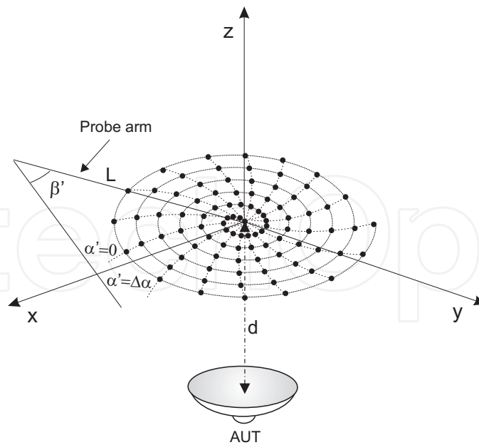
Fig. 8. Planar spiral near-field scanning.
