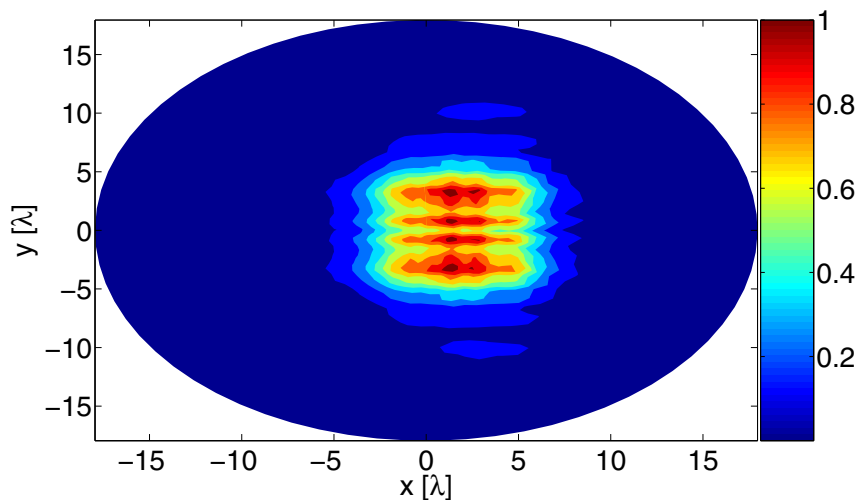
Fig. 10. Normalized bi-polar near-field amplitude for a 21x21 dipole array with Taylor illumination.
