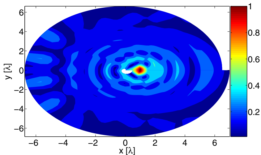
Fig. 12. Normalized bi-polar near-field amplitude for a 21x21 dipole array with Taylor illumination.
