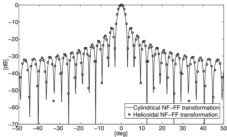
Fig. 4. Far-field amplitude ( E_\theta component) for linear array of z-oriented 37 elementary Huyghens sources: comparison between cylindrical and helicoidal NF-FF transformations.
