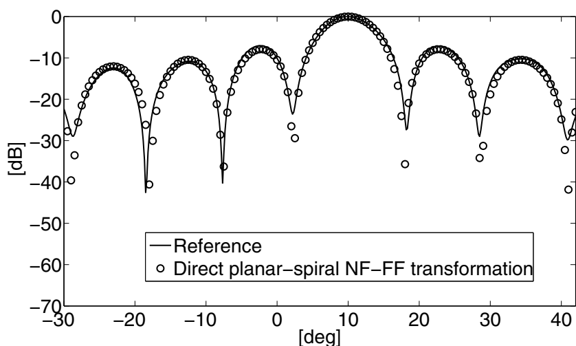
Fig. 13. Co-polarized H-plane pattern for a 21x21 dipole array with Taylor illumination.
