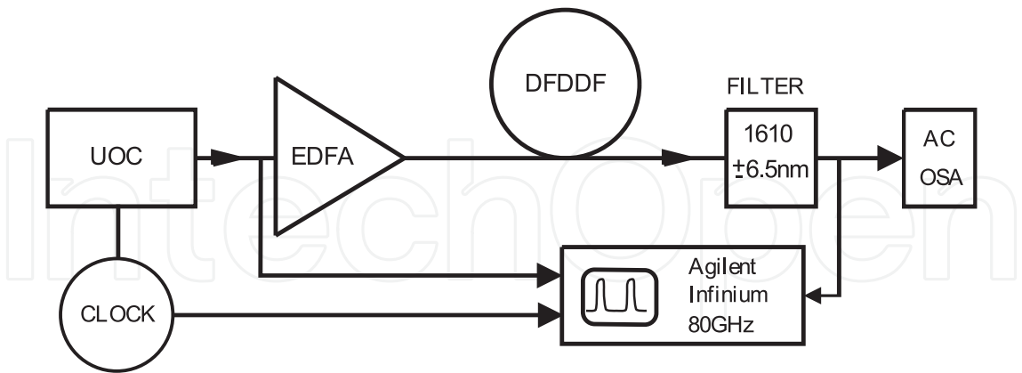
Fig. 13. Experimental setup: Pritel UOC, picosecond pulse source; EDFA, Er-doped fiber amplifier; DFDDF, 42 m length of dispersion flattened dispersion decreasing fiber; AC, autocorrelator “Femtochrome”; OSA, optical spectrum analyzer ‘Ando AQ6317’; “Agilent Infinium”, sampling scope with 80 GHz bandwidth; “FILTER”, WDM filter
