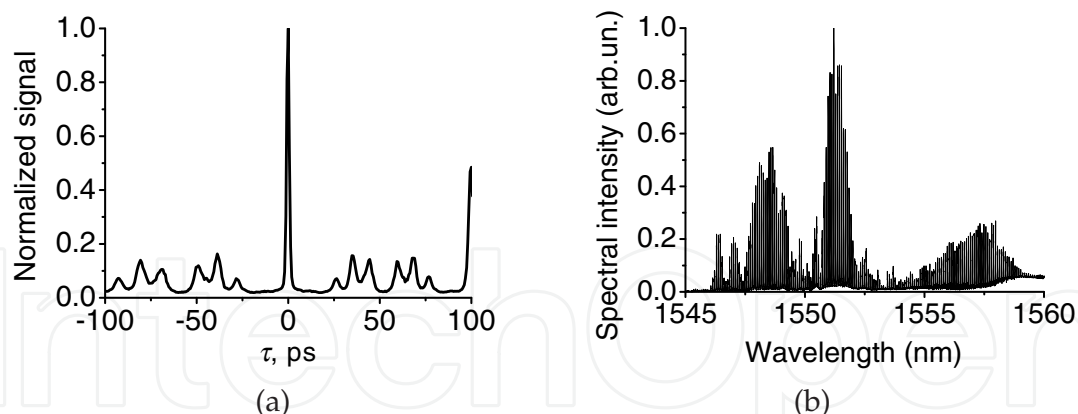
Fig. 9. High power pulse transmission through DOF. (a) Autocorrelation trace. (b) pulse train spectrum. Width of initial pulse is T_{FWHM} = 2.05 ps, The input average power is P = 258.9 mW. The phase of modulation is \varphi = 0 .
