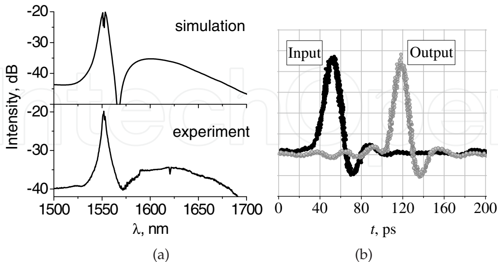
Fig. 15. Output of the DFDDF fiber. (a) Optical spectra obtained by simulation (top) and experimentally (bottom); (b) Sampling scope trace of the pulse at DFDDF input (black color) and output signal of 1610 nm filter (gray color). Input pulse energy is 140 nJ. Pulse repetition rate is 5.37 GHz.
