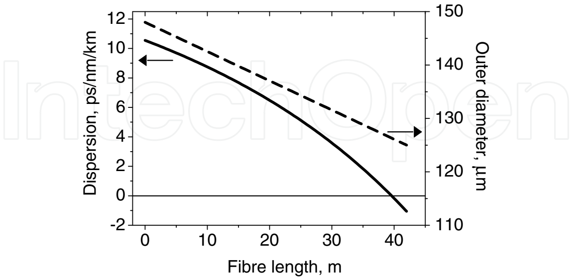
Fig. 14. Dispersion (solid curve) and outer diameter (dashed curve) of DFDDF versus fiber length.
