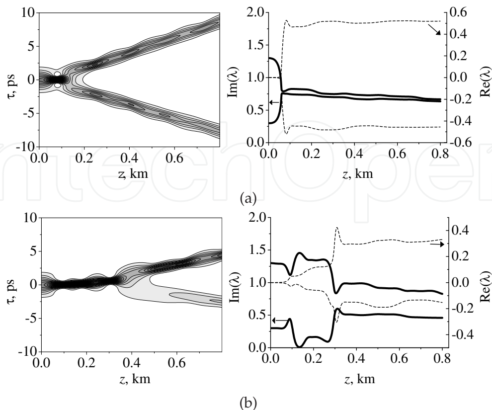
Fig. 10. Numerical simulation of the pulse evolution in DOF. Width of initial pulse is T_{\text{FWHM}} = 2.05 ps, The pulse has soliton order N = 1.8 . (a) \varphi = \pi . (b) \varphi = 0 .
