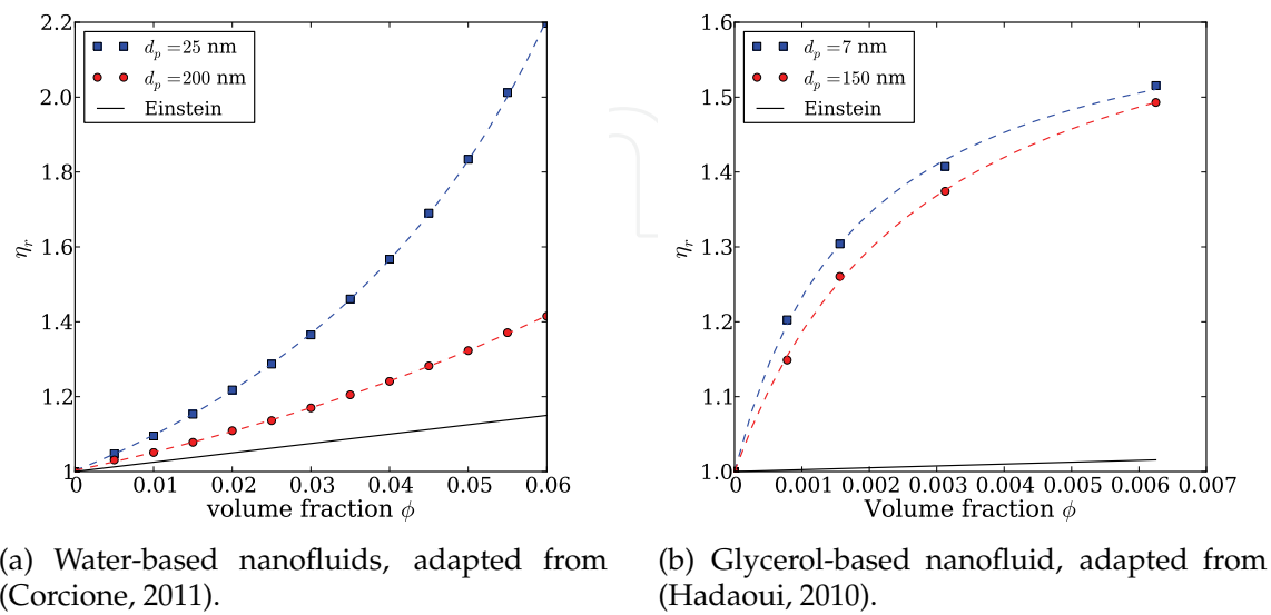
Fig. 11. Evolution of viscosity as a function of \phi and NPs diameter d_p .
