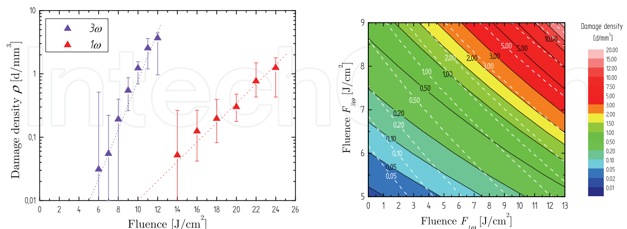
Fig. 8. (a) Damage density versus fluence in the mono-wavelength case: for 1\omega and 3\omega . (b) Evolution of the LID densities (expressed in \text{dam./mm}^3 ) as a function of F_{3\omega} and F_{1\omega} . The color levels stand for the experimental damage densities. Modeling results are represented in white dash contour lines for \delta = 3 . Modeling results are discussed in Sec. 3.2.3.
