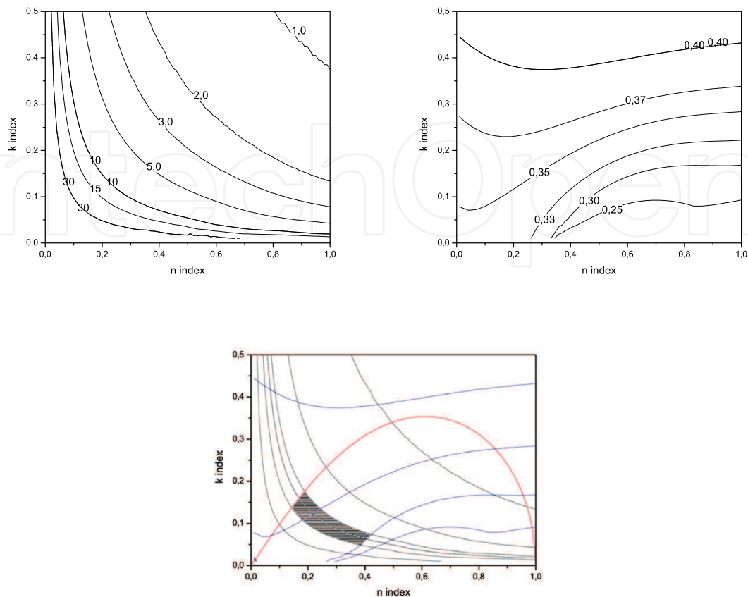
Fig. 2. (top left) Critical fluence F_c in J.cm^{-2} as a function of n and k for \tau = 3 ns . (top right) Scaling law exponent x as a function of n and k for \tau \in [1. ns; 10. ns] . (bottom) Intersection of (a) and (b), the highlighted area delimits the region satisfying experimental data.
