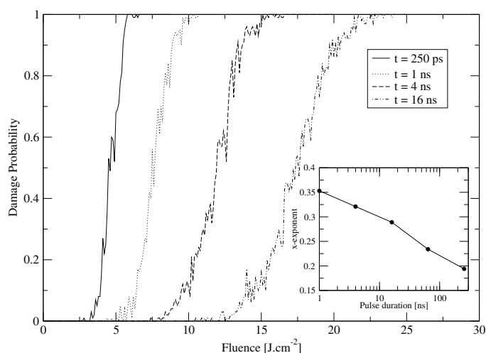
Fig. 4. Evolution of the damage probability as a function of fluence within the 1D model. Four pulse durations are considered : \tau = 250\text{ps} , 1\text{ns} , 4\text{ns} and 16\text{ns} . Parameters are n_{ADNS} = 100 and N = 10000 . 200 drawings have been performed for each fluence. Sub-figure displays the scaling law exponent as a function of the pulse duration (see text).
