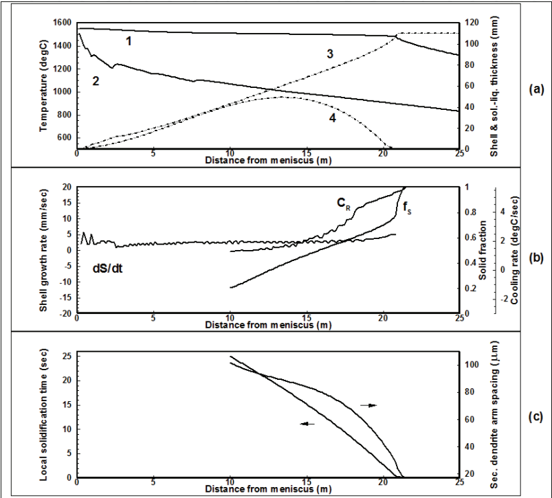
Fig. 8. Results with respect to distance from the meniscus: In part (a), lines (1) and (2) illustrate the centreline and surface temperatures of a 220 × 1500 mm x mm Stomana slab; lines (3) and (4) depict the shell thickness and the distance between the solidus and liquidus temperatures; in part (b), the solid fraction f_s , the local cooling-rate C_R , and the rate of shell growth dS/dt are presented; in part (c), the local solidification time and secondary dendrite arm spacing are depicted, as well. Casting conditions: %C = 0.185; casting speed: 0.80 m/min; SPH: 40 K; solidus temperature = 1479°C; (all temperatures in the graph are in °C)
