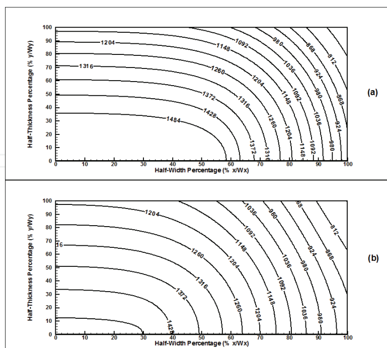
Fig. 16. Temperature distribution in sections of a 130 x 390 mm x mm Sovel slab, at 7.3 m for part (a) and 9.5 m from the meniscus, respectively. %C = 0.165; casting speed: 1.1 m/min; SPH: 40 K; solidus temperature = 1484°C; (all temperatures in the graph are in °C)
