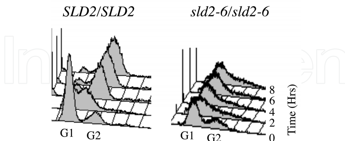
Fig. 1. Flow cytometry profiles of SLD2/SLD2 and sld2-6/sld2-6 mutant cells that have been induced to initiate meiotic differentiation at the non-permissive temperature of 36°C. The sld2-6 mutant arrests in G1-phase – early S-phase and does not complete S-phase. The sld2-6 temperature sensitive allele was provided by Dr. H. Araki and was introduced into the S. cerevisiae SK1 genetic background by gene replacement.
