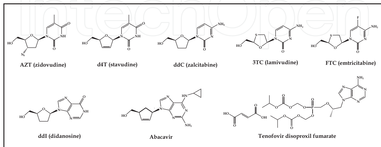
Fig. 6. Chemical structures of approved NRTIs: \beta -D-(+)-3'-azido-3'-deoxythymidine (zidovudine, AZT), \beta -D-(+)-2',3'-dideoxy-2',3'-dideoxythymidine (stavudine, d4T), \beta -D-(+)-2',3'-dideoxyinosine (didanosine, ddI), \beta -D-(+)-2',3'-dideoxycytidine (zalcitabine, ddC), \beta -L-(-)-2',3'-dideoxy-3'-thiacytidine, (lamivudine, 3TC), (-)-(1S,4R)-4-[2-amino-6-(cyclopropylamino)-9H-purin-9-yl]-2-cyclopentene-1-methanol (abacavir), \beta -L-(-)-2',3'-dideoxy-5-fluoro-3'-thiacytidine (emtricitabine, FTC), and R-9-(2-phosphonomethoxy-propyl)adenine disoproxil fumarate (tenofovir disoproxil fumarate).
