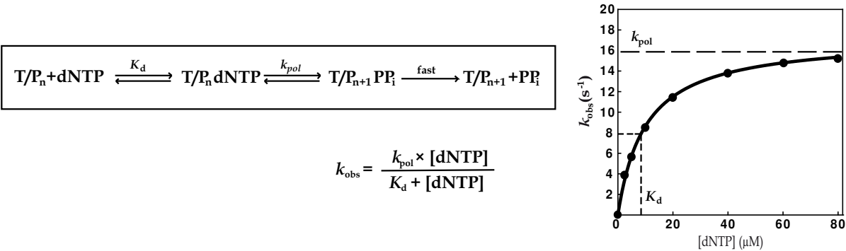
Fig. 5. Nucleotide incorporation reaction and example of the determination of kinetic parameters k_{pol} and K_d under pre-steady-state conditions. \text{T/P}_n represents the template-primer with n being the nucleotide length, and \text{T/P}_{n+1} represents the same template-primer after the incorporation of one nucleotide. \text{PP}_i stands for pyrophosphate.
