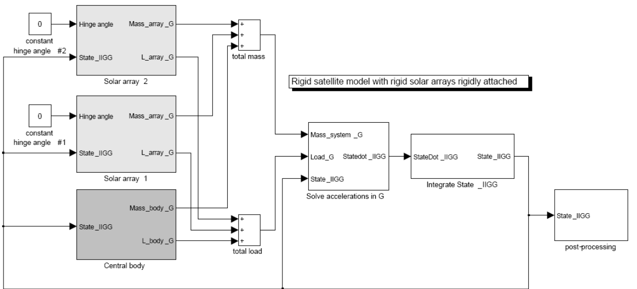
Fig. 6. Top-level architecture of a single-satellite simulator.
