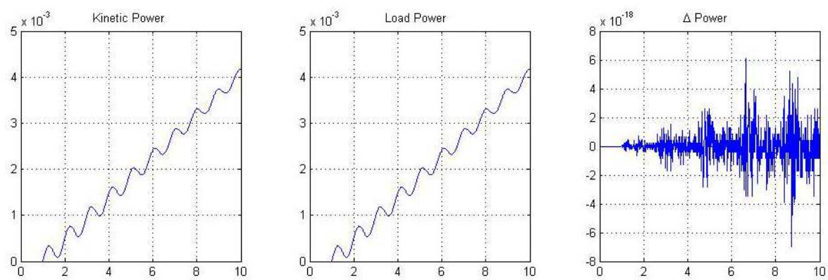
Fig. 12. Time history of the power conservation laws
