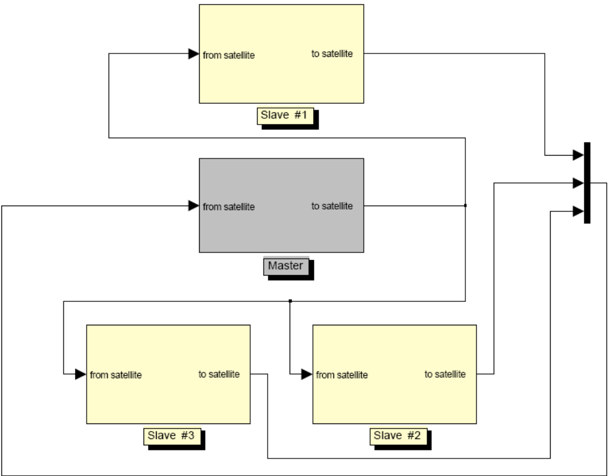
Fig. 9. Formation-flying simulator for four satellites.
