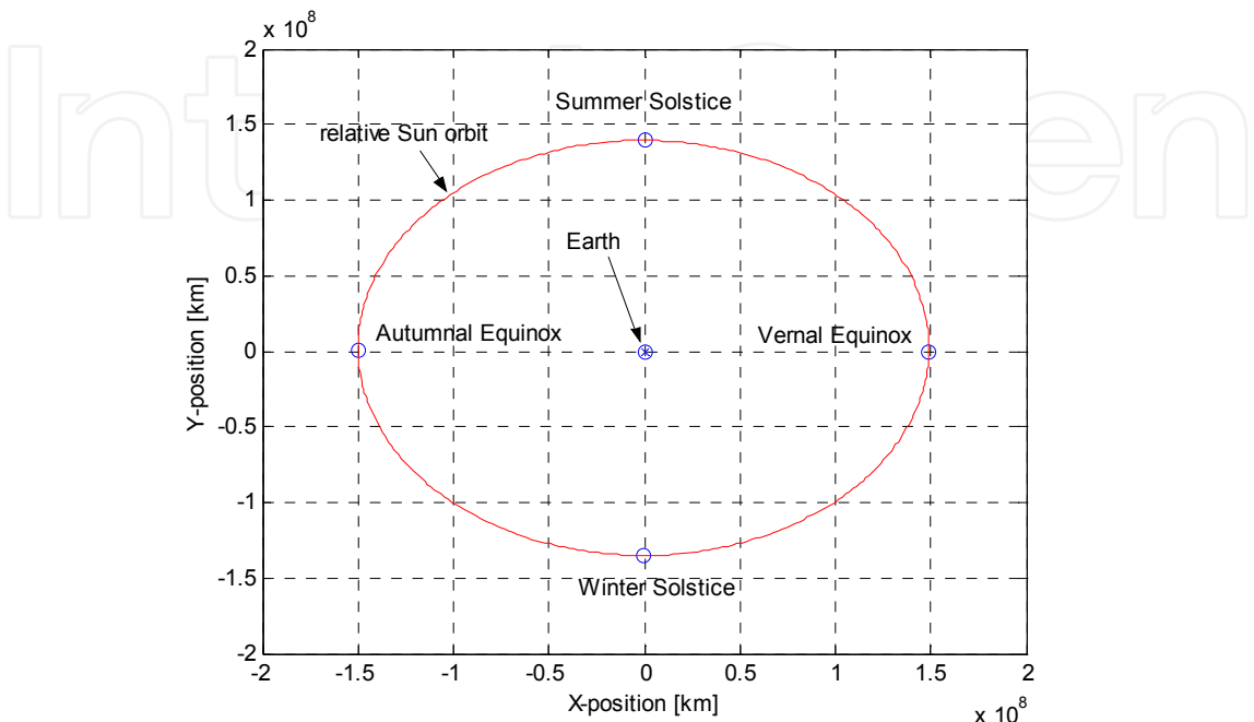
Fig. 4. Relative in-plane orbit of the Sun around the Earth. The Equinoxes appear at y = 0 , whereas the Solstices appear at x = 0 .
