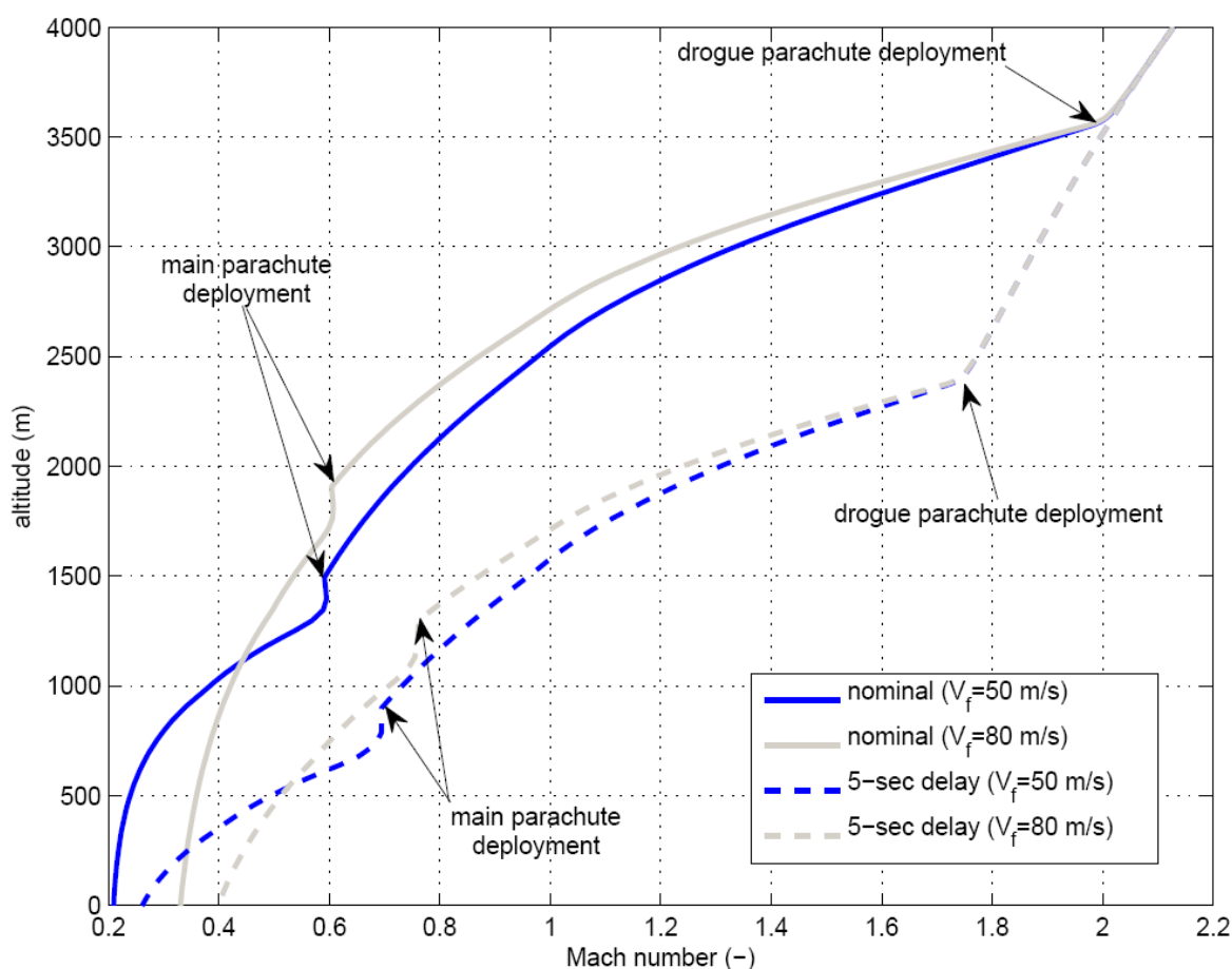
Fig. 16. Altitude-Mach number profile for different parachute-deployment timings.
