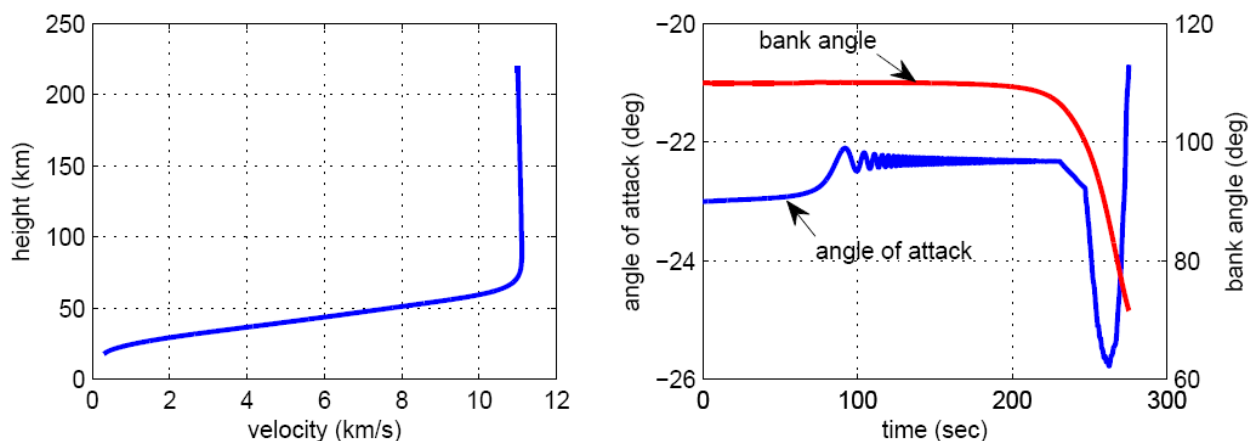
Fig. 15. Altitude-velocity profile (left) and attitude angles versus time (right).
