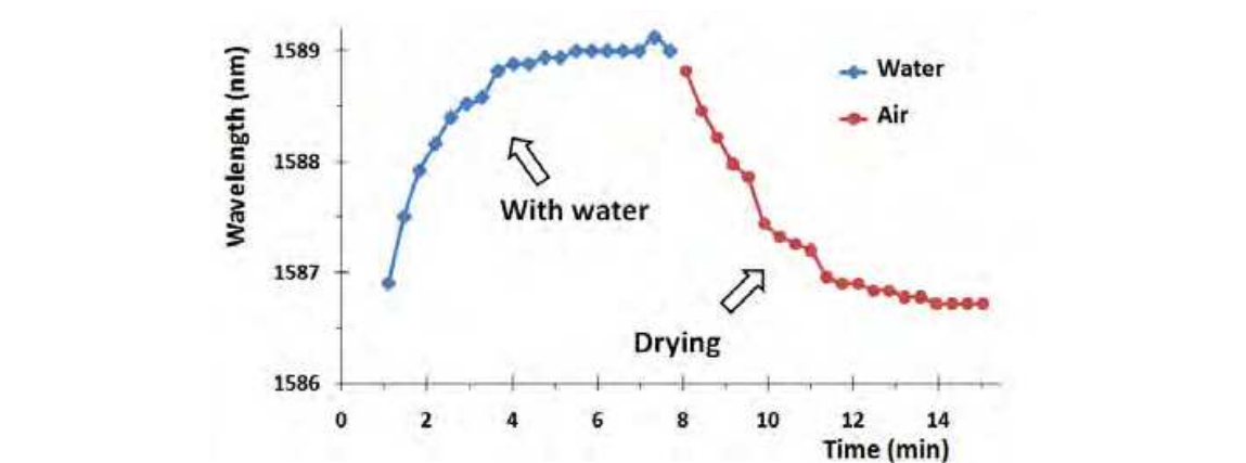
Fig. 27. Central wavelength of Bragg grating within the cavity during the stabilization period when the cavity is filled with water and then subject to a drying process.
