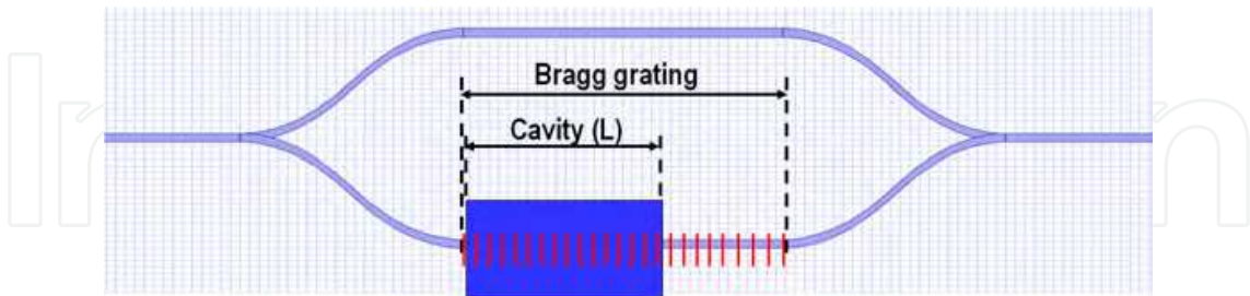
Fig. 19. Schematic of the refractive index sensor. The shaded zone represents the cavity with length L where the refractive index change will take place.
