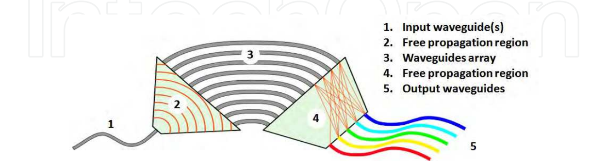
Fig. 30. Schematic representation of an M \times N arrayed waveguide grating. When the propagating beam, coming from an input waveguide, enters the free propagation region (FPR) it is no longer laterally confined. At the end of this section, the beam is coupled into the waveguides array, propagating through each of them to the second FPR. The length
