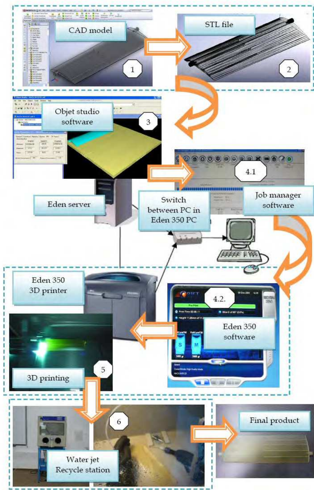
Fig. 9. EDEN 350 flow chart
