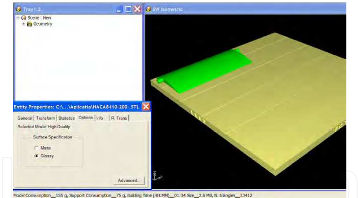
Fig. 14. The orientation of the 3D model on the EDEN350 build tray: 0°, glossy mode Results regarding this case study are presented in the table 1.
