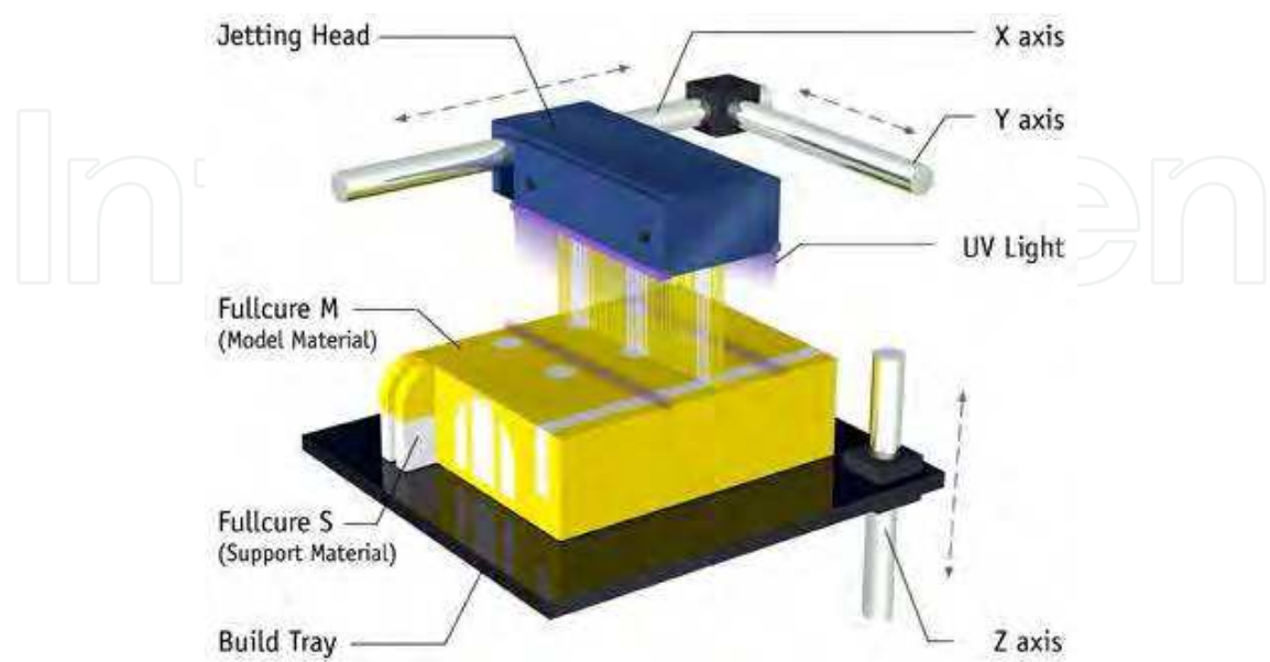
Fig. 4. “Polymer jetting” printing (photo courtesy of Objet) (Objet Geometries Ltd., 2010)
