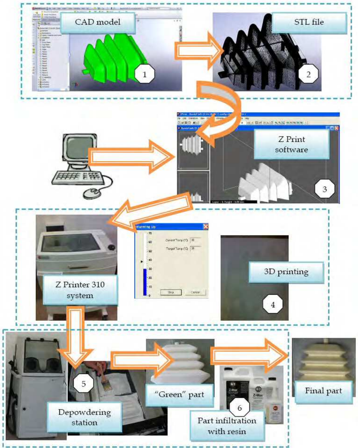
Fig. 7. ZPrint flow chart Generally, the 3D printing process consists in the following main steps: pre-processing, processing and post-processing. The ZPrint flow chart is shown in fig. 7. In the pre-processing stage a 3D file is imported into the ZPrint software (STL, PLY or VRML file), scale it (if necessary), orientate the part and simulate the manufacturing process
