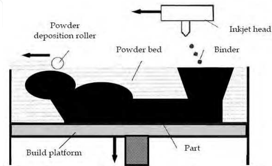
Fig. 5. "Inkjet" printing
