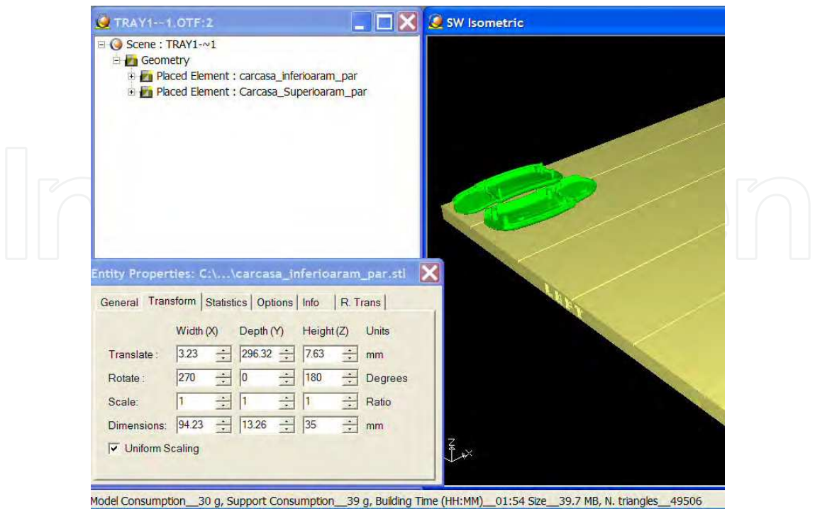
Fig. 20. Positioning of parts along Y axis, “XY-00” rule satisfied (polyjet technology)
