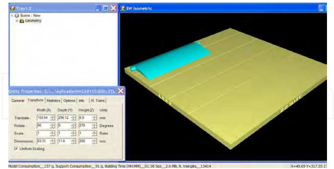
Fig. 13. The orientation of the 3D model on the EDEN350 build tray: 0° (the biggest dimension along X)
