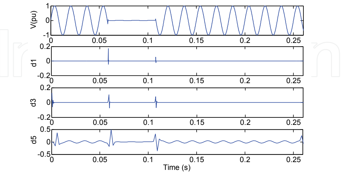
Fig. 3. The voltage interruption signal and detail coefficients: first decomposed level ( d_1 ), third decomposed level ( d_3 ), and fifth decomposed level ( d_5 )
