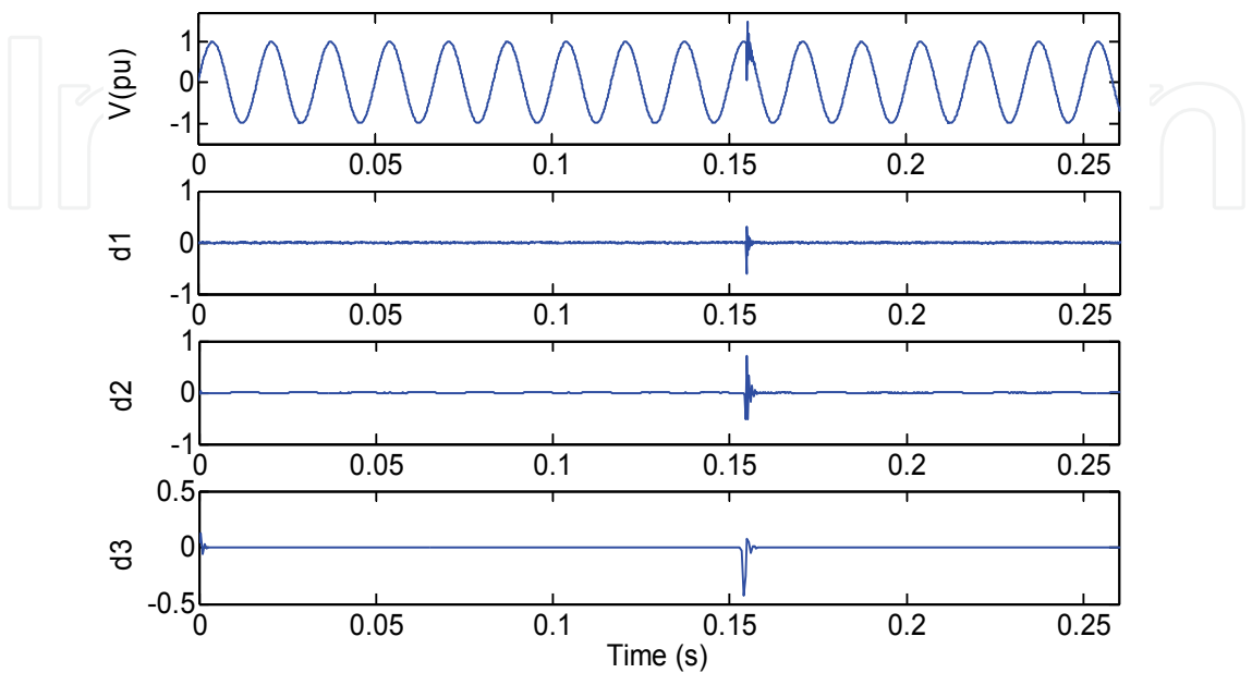
Fig. 4. The capacitor switching signal and detail coefficients: first decomposed level (d1), second decomposed level (d2), and third decomposed level (d3)
