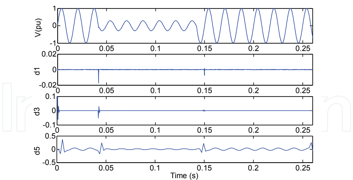
Fig. 5. The voltage sag and detail coefficients: first decomposed level (d1), third decomposed level (d3), and fifth decomposed level (d5)
