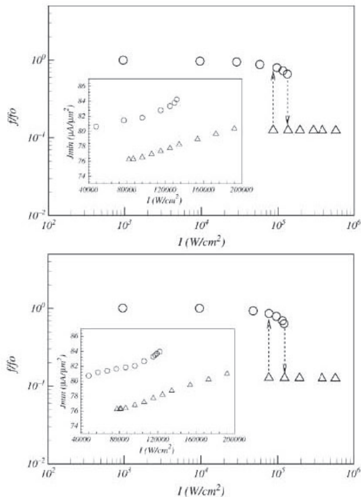
Fig. 5. The upper portion: the nonlinear electro-optic characteristic when exclusion of the II effect. The corresponding J_{min} - I hysteric curve is shown in the inset. The lower portion: the same illustrations as in the upper portion but inclusion of the II effect.
