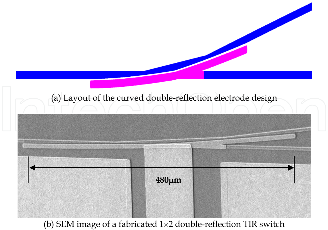
Fig. 14. 1x2 TIR optical switch with curved double-reflection electrode.
