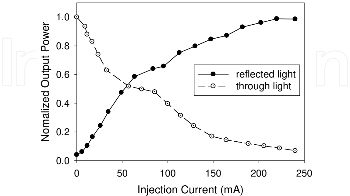
Fig. 13. Measured switching characteristics of a fabricated 2x2 double-reflection TIR optical switch.
