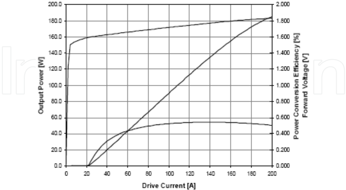
Fig. 4. PIV-PCE characteristic of a 50% filling factor 808 nm bar on micro channel cooler at 25 °C water temperature from the Oclaro Company.
