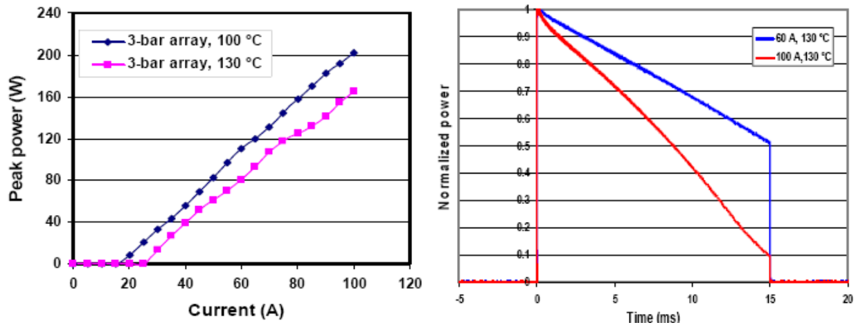
Fig. 2. High temperature performance of 3-bar array (left) and its pulse shape at 130 °C (right).
