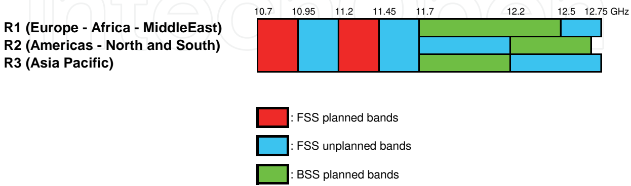
Fig. 5. Ku band allocation for SATCOM downlink.
