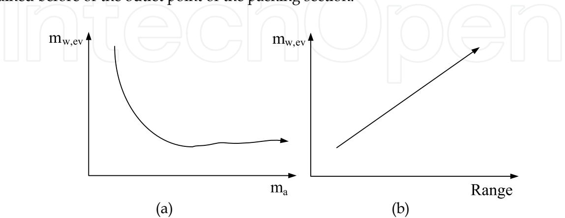
Fig. 6. Evaporate profile respect to air flow rate and range
