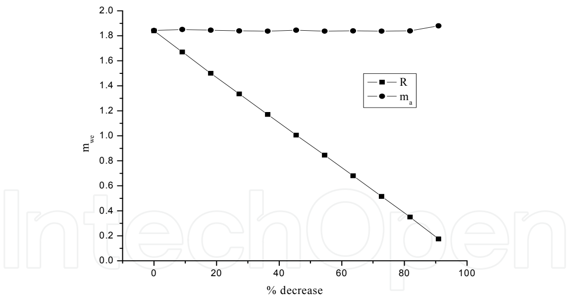
Fig. 7. Sensitivity analysis of the evaporate rate with respect to air flowrate and range
