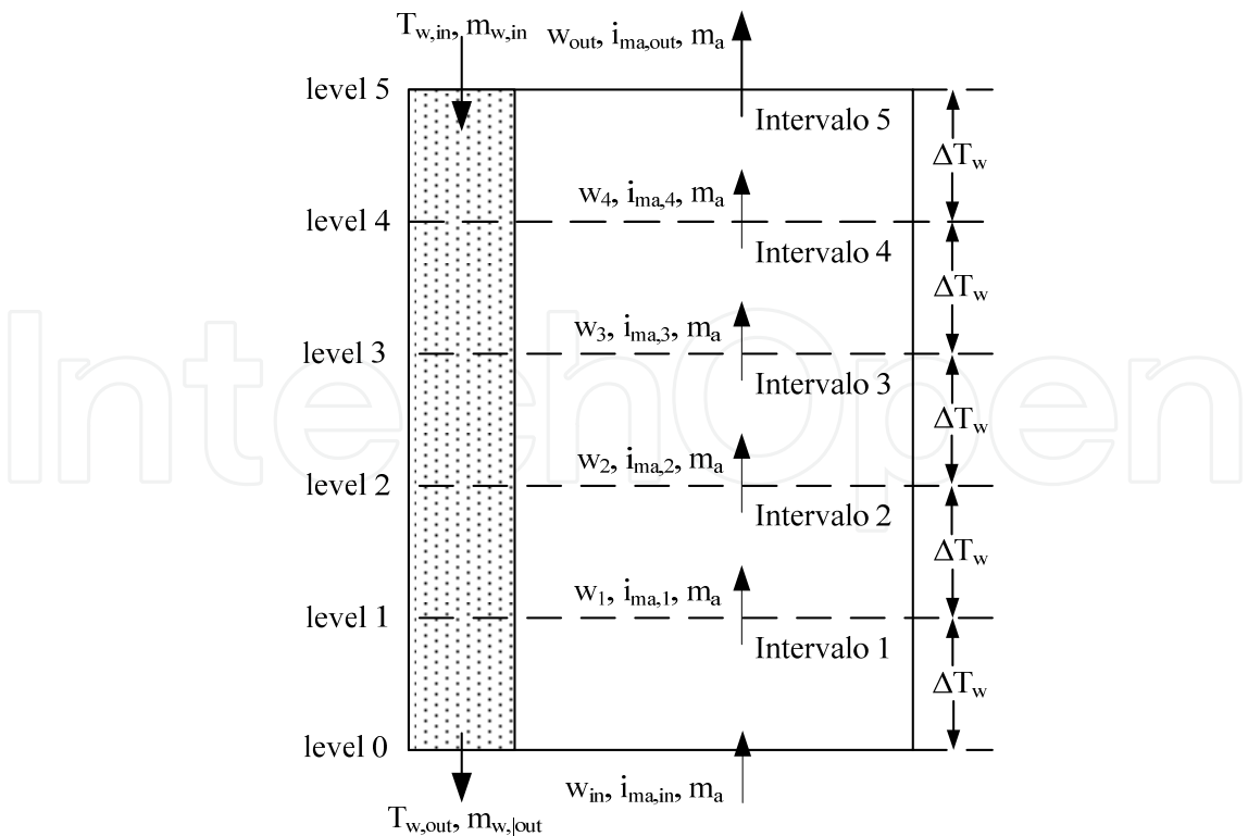
Fig. 4. Graphical representation of the Runge-Kutta method
