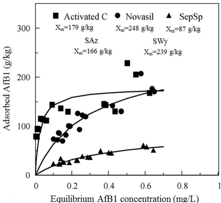
Fig. 2. Aflatoxin B1 adsorption to activated carbon, Novasil, SepSp, SWy, and SAz from water fitted to Langmuir model with monolayer adsorption capacities ( X_m ) calculated from Langmuir fit parameters.
