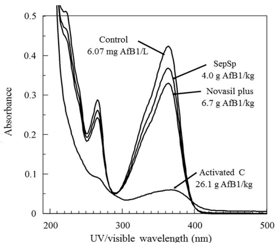
Fig. 4. Spectra of aqueous Control, Novasil plus, SepSp, and activated carbon samples (2 mg) after adsorption of aflatoxin B1 and extraction with 60% methanol. Maximum absorbance of aflatoxin B1 is at 360 nm. The amounts of aflatoxin adsorbed were calculated from the sample weights and absorbance differences from the control.
