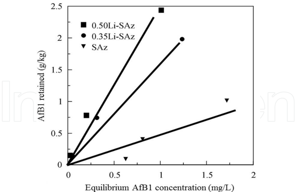
Fig. 8. Aflatoxin B1 retention from aqueous corn meal by natural (SAz) and reduced-charge SAz samples after 60% methanol extraction. Layer charge decreases in the order SAz > 0.35Li-SAz > 0.50Li-SAz.
