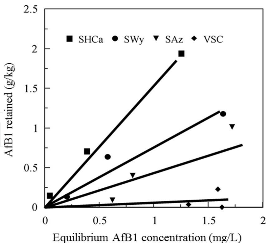
Fig. 7. Aflatoxin B1 retention from aqueous corn meal by natural clay samples after 60% methanol extraction with layer charge decreasing in the order VSC > SAz > SWy > SHCa.
