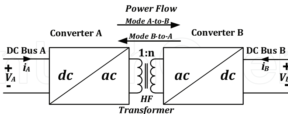
Fig. 5. Basic structure of an IBDC
