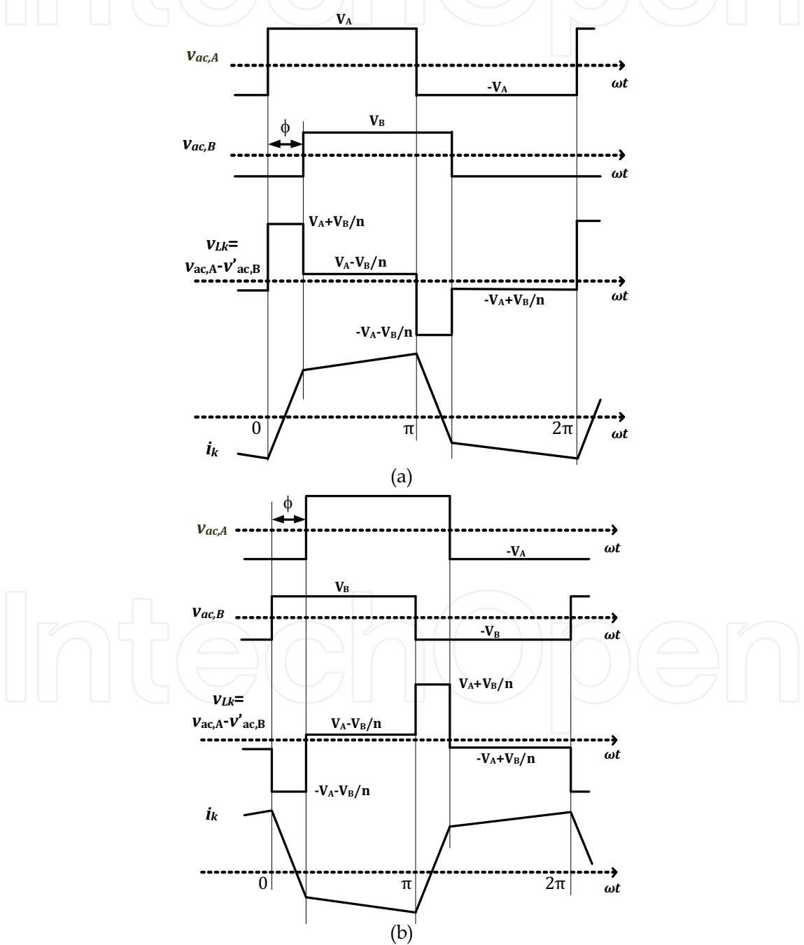
Fig. 7. Operating waveforms of Configuration 1. (a) A-to-B mode and (b) B-to-A mode
