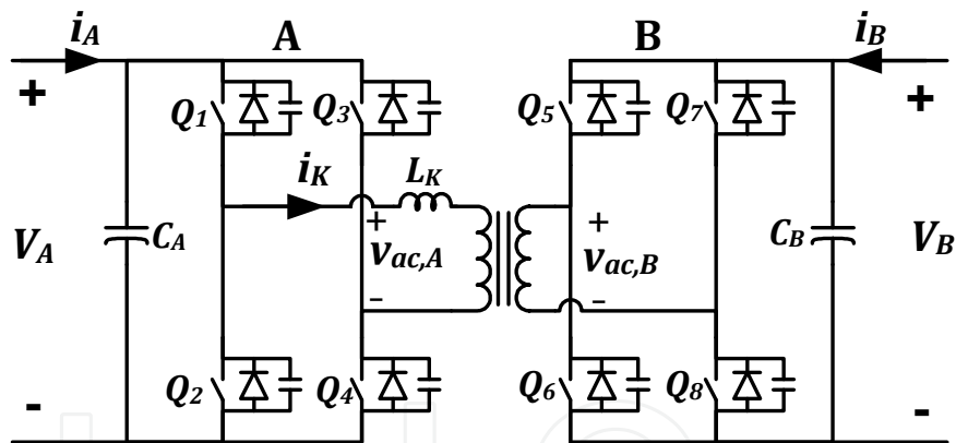
Fig. 6. Circuit diagram of Configuration 1.
