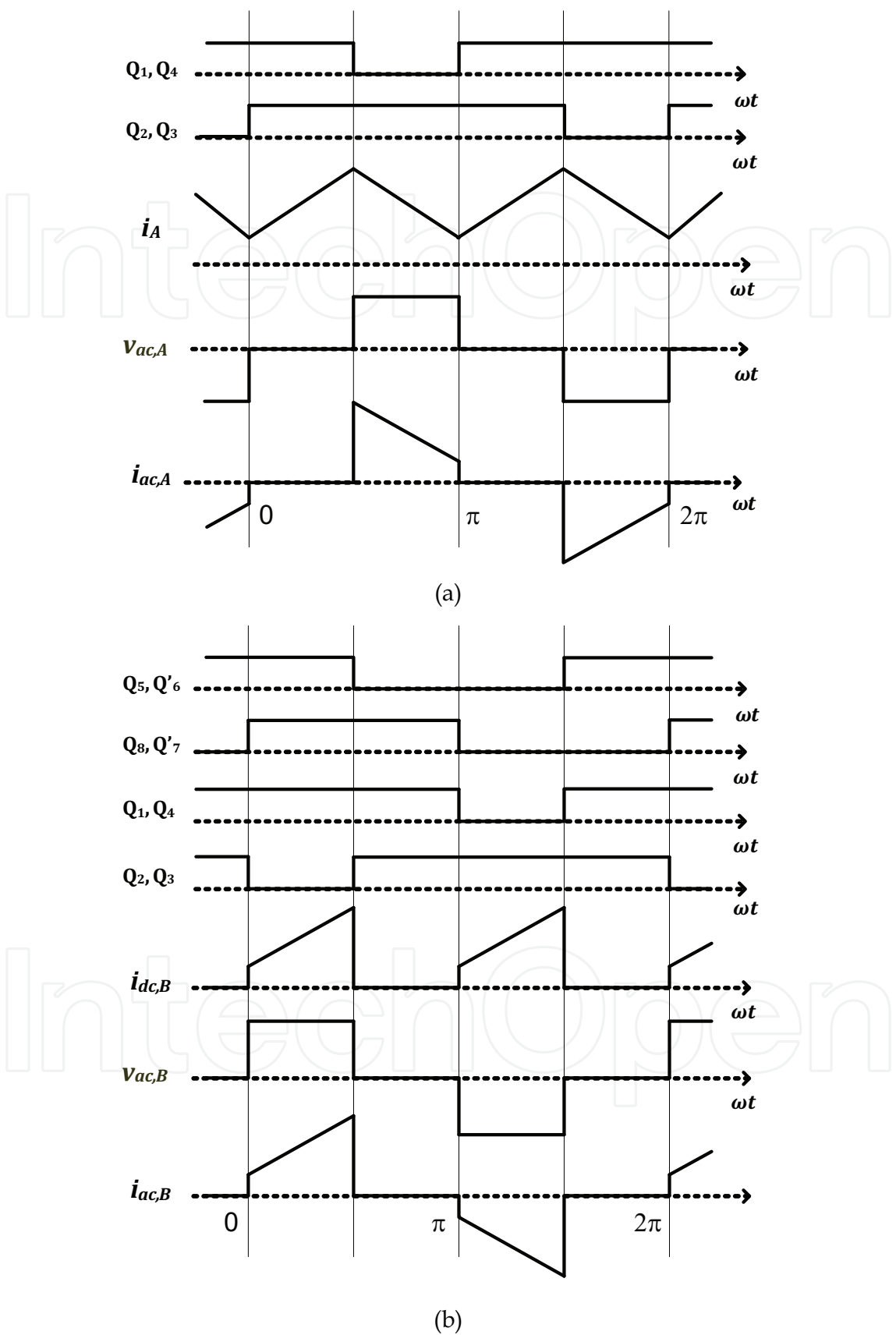
Fig. 9. Operating waveforms of Configuration 2. (a) A-to-B mode and (b) B-to-A mode
