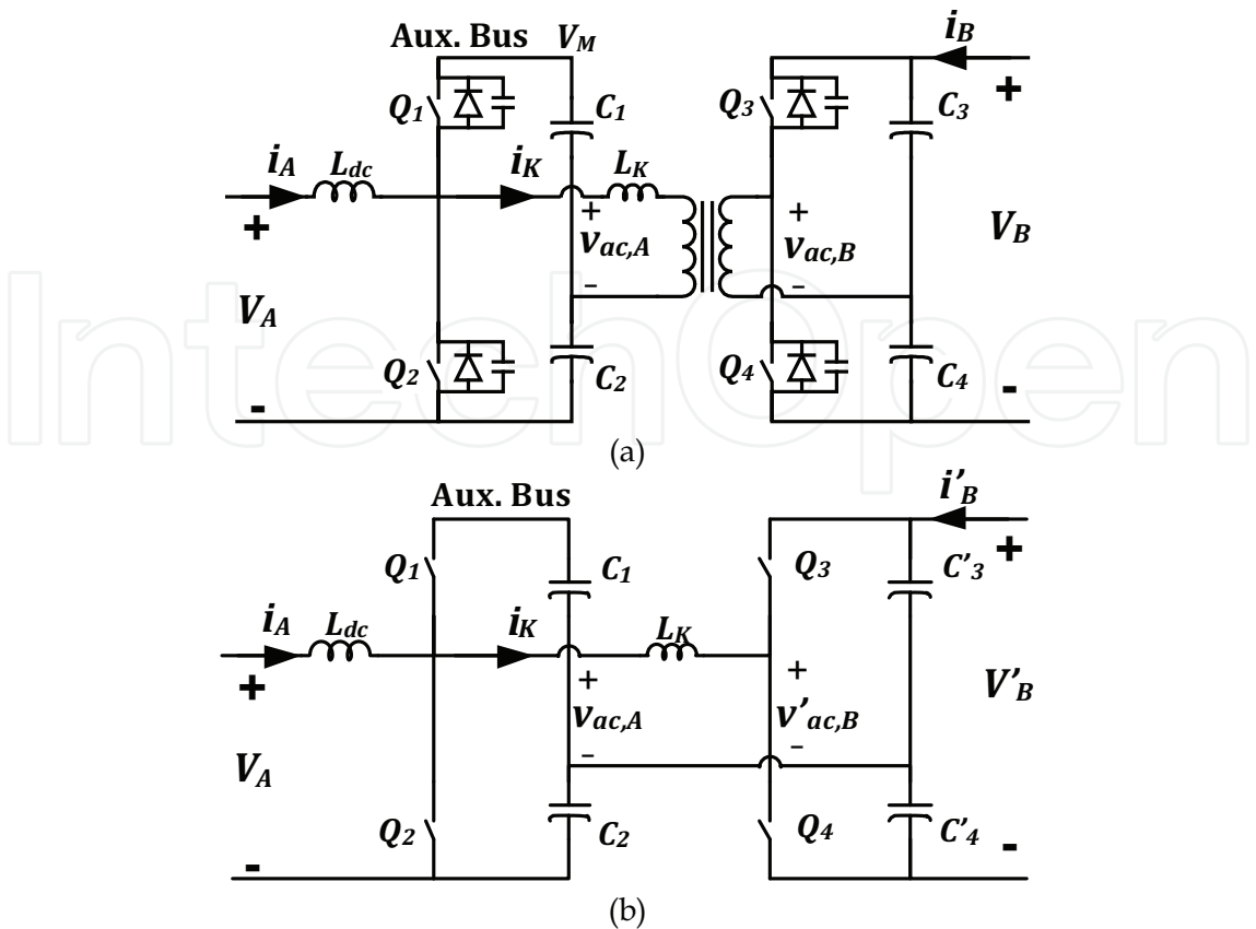
Fig. 10. (a) Circuit diagram of Configuration 3 and (b) idealized model.
