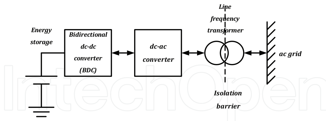
Fig. 12. Basic structure of an energy storage device connected to an ac grid through a line-frequency transformer.
