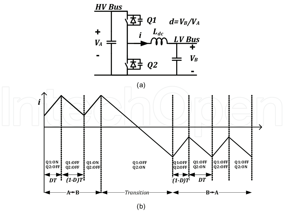
Fig. 2. (a) Basic NBDC and (b) operating waveforms.
