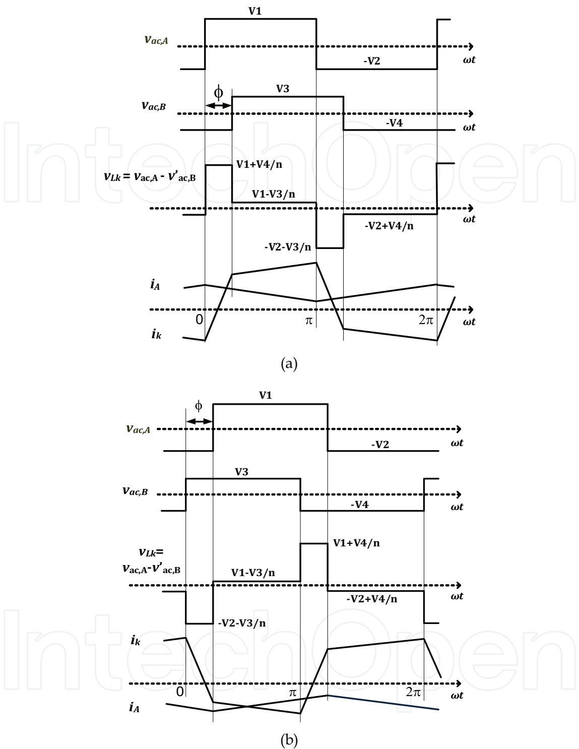
Fig. 11. Operating waveforms of Configuration 3. (a) A-to-B mode and (b) B-to-A mod
