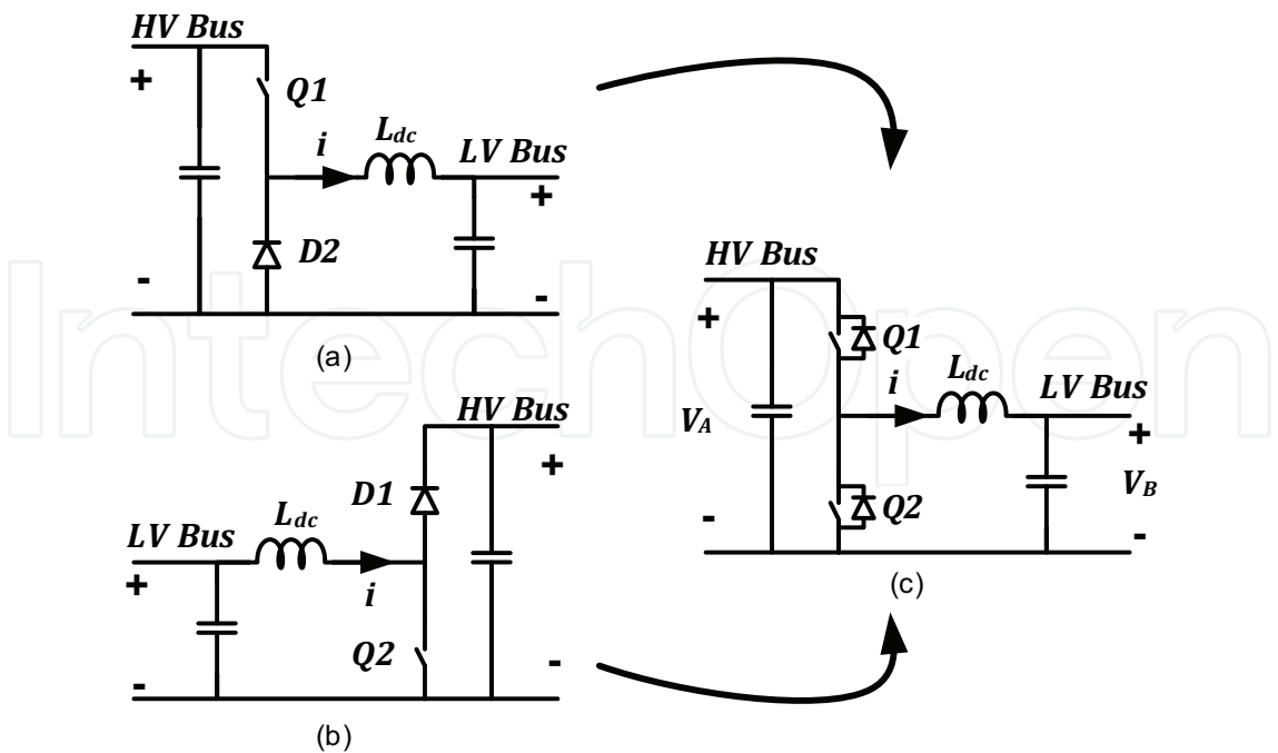
Fig. 1. (a) Elementary unidirectional buck converter, (b) elementary unidirectional boost converter and (c) transformation to bidirectional converter by substituting diodes with a controllable switch.
