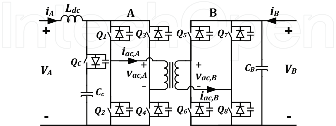
Fig. 8. Circuit diagram of Configuration 2.
