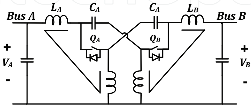
Fig. 4. A different structure for NBDC
