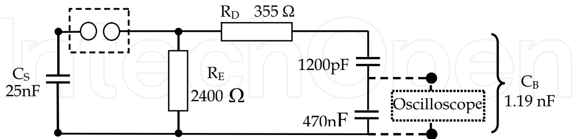
Fig. 14. Circuit diagram for stage 1 testing
