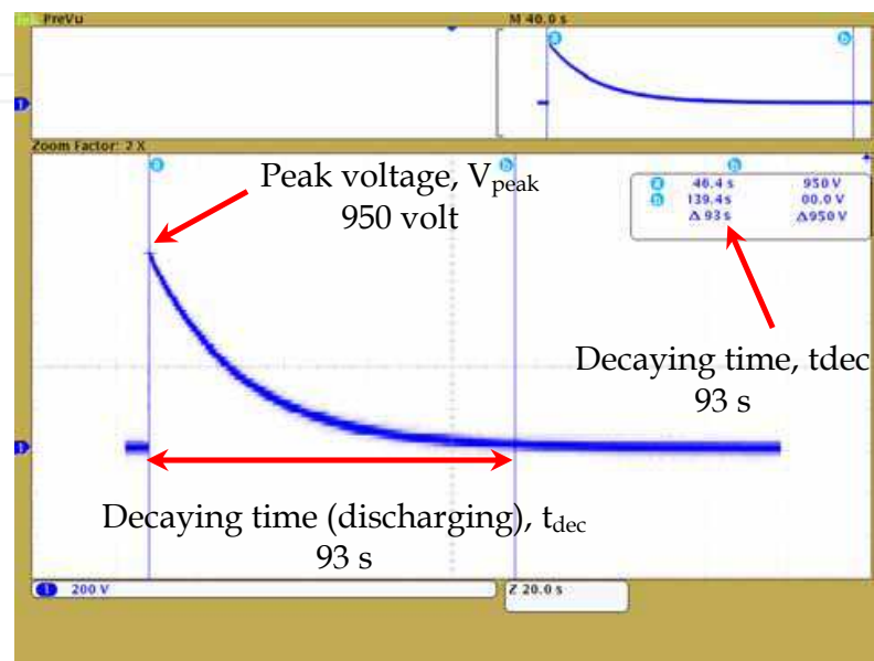
Fig. 19. Decaying time for one unit sample capacitor 0.22 \mu F
