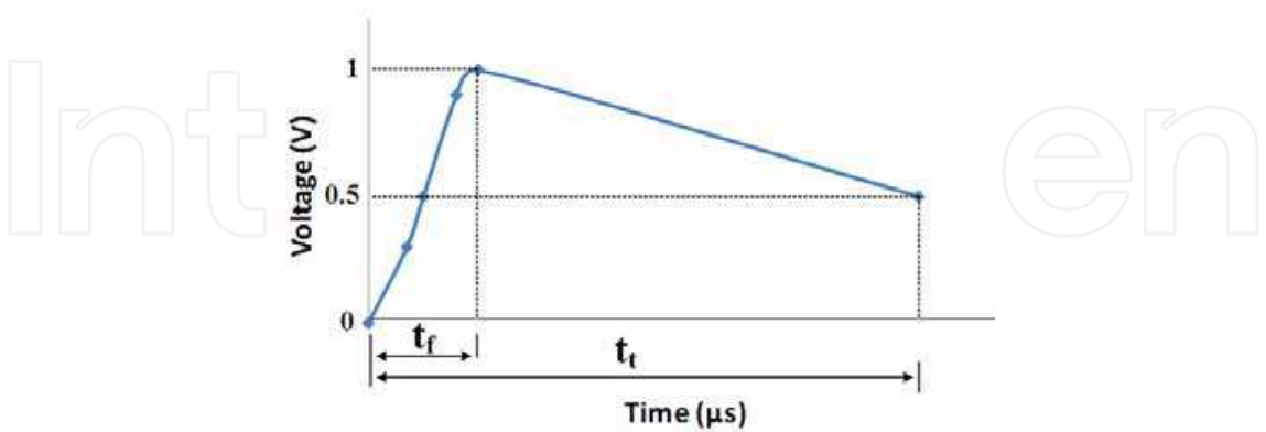
Fig. 2. Standardized impulse voltage wave shape
