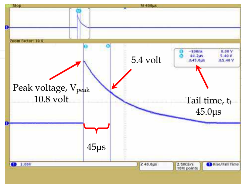
Fig. 16. Tail time t_t of the experimental impulse voltage wave shape
