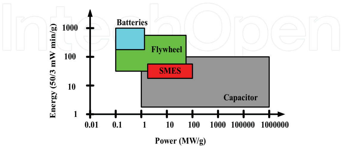
Fig. 3. Specific power versus specific energy ranges
