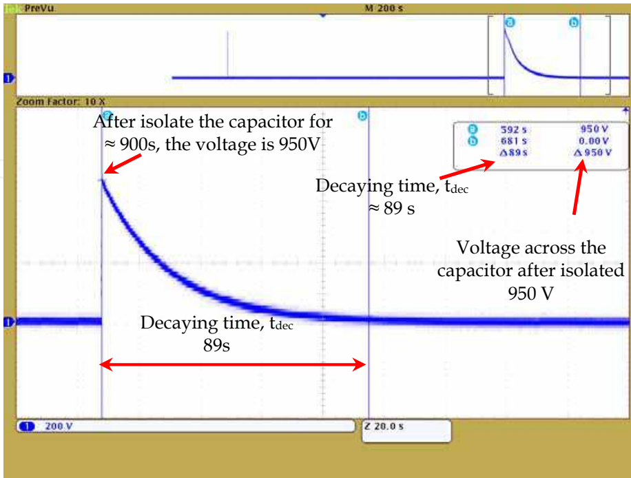
Fig. 25. Voltage waveform of the sample capacitor after isolating period.
