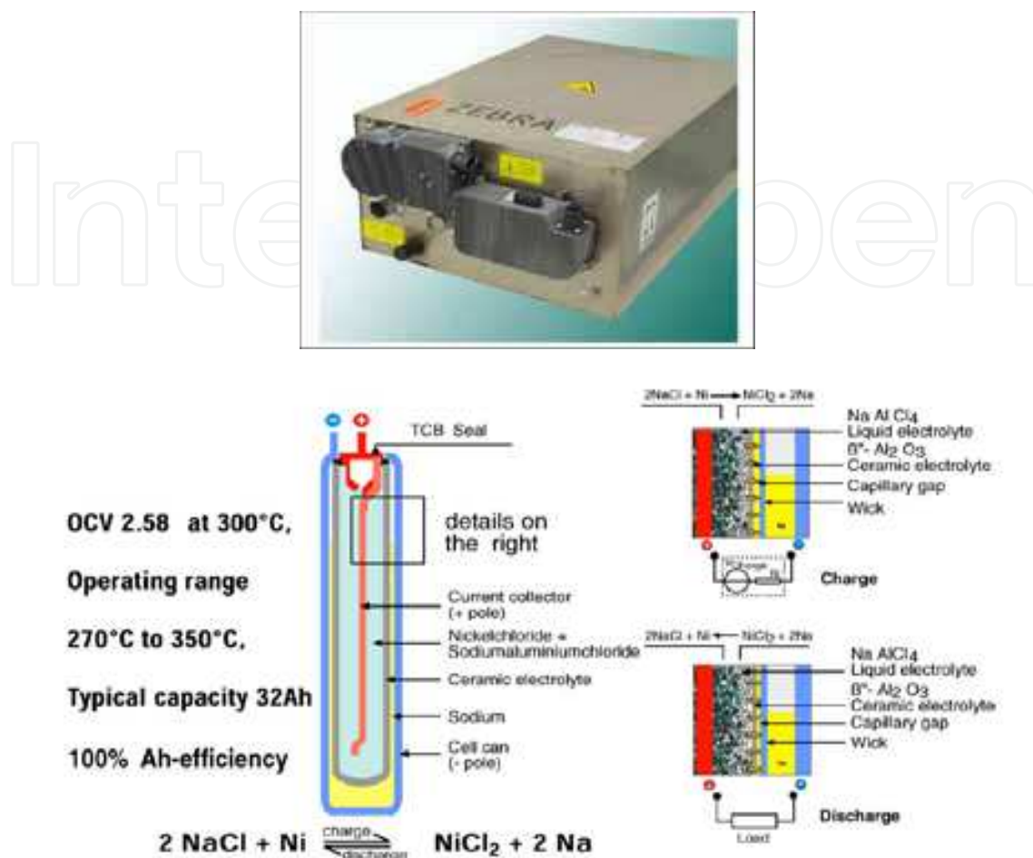
Fig. 5. Zebra battery
