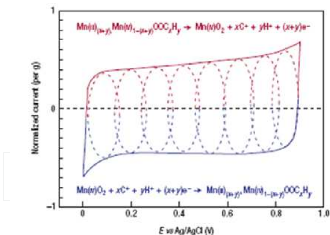
Fig. 10. Voltammogram of a \text{MnO}_2 electrode in neutral aqueous electrolyte
