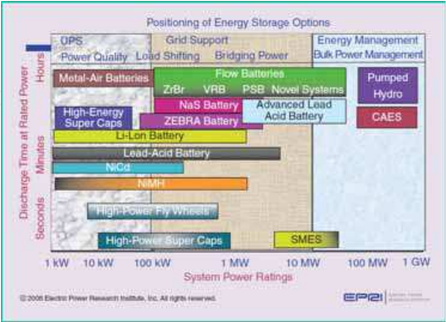
Fig. 1. The state of the art of storage technologies (source: EPRI)
