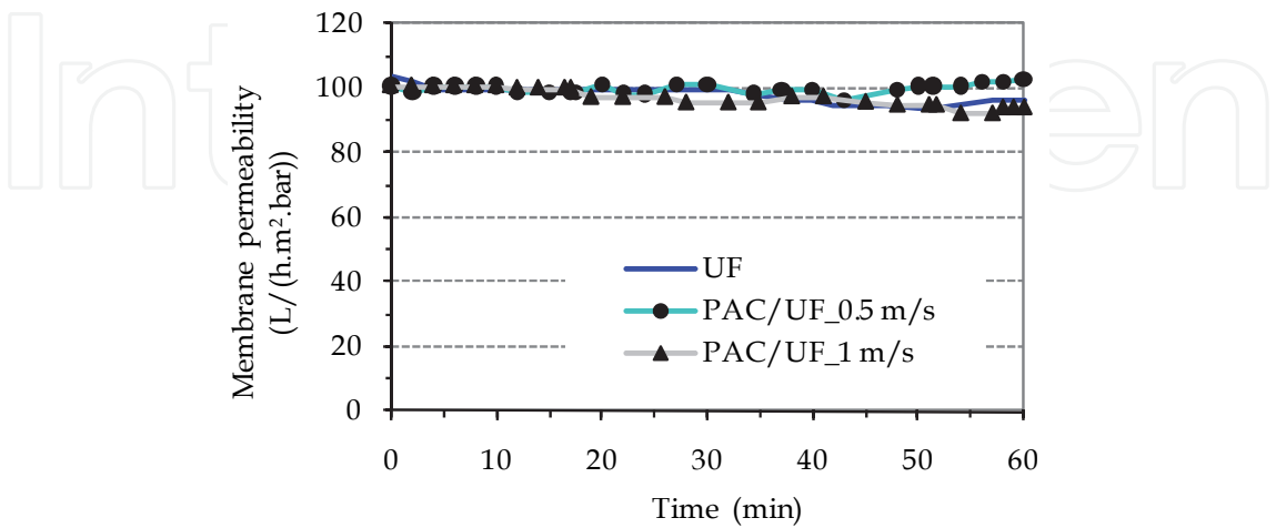
Fig. 6. Membrane permeability during UF and PAC/UF time-depending fouling runs at two cross-flow velocities (UF: no PAC addition; PAC/UF: 5 mg/L PAC).
