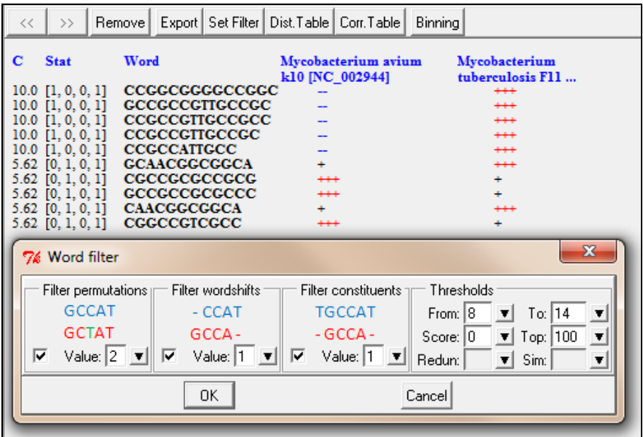
Fig. 6. The top 10 most diverse words which separate M. tuberculosis from M. avium . The filter was set to reduce the redundancy of the selected words. Next, the distance values D between an unknown sequence and the taxonomic units were calculated as follows:
