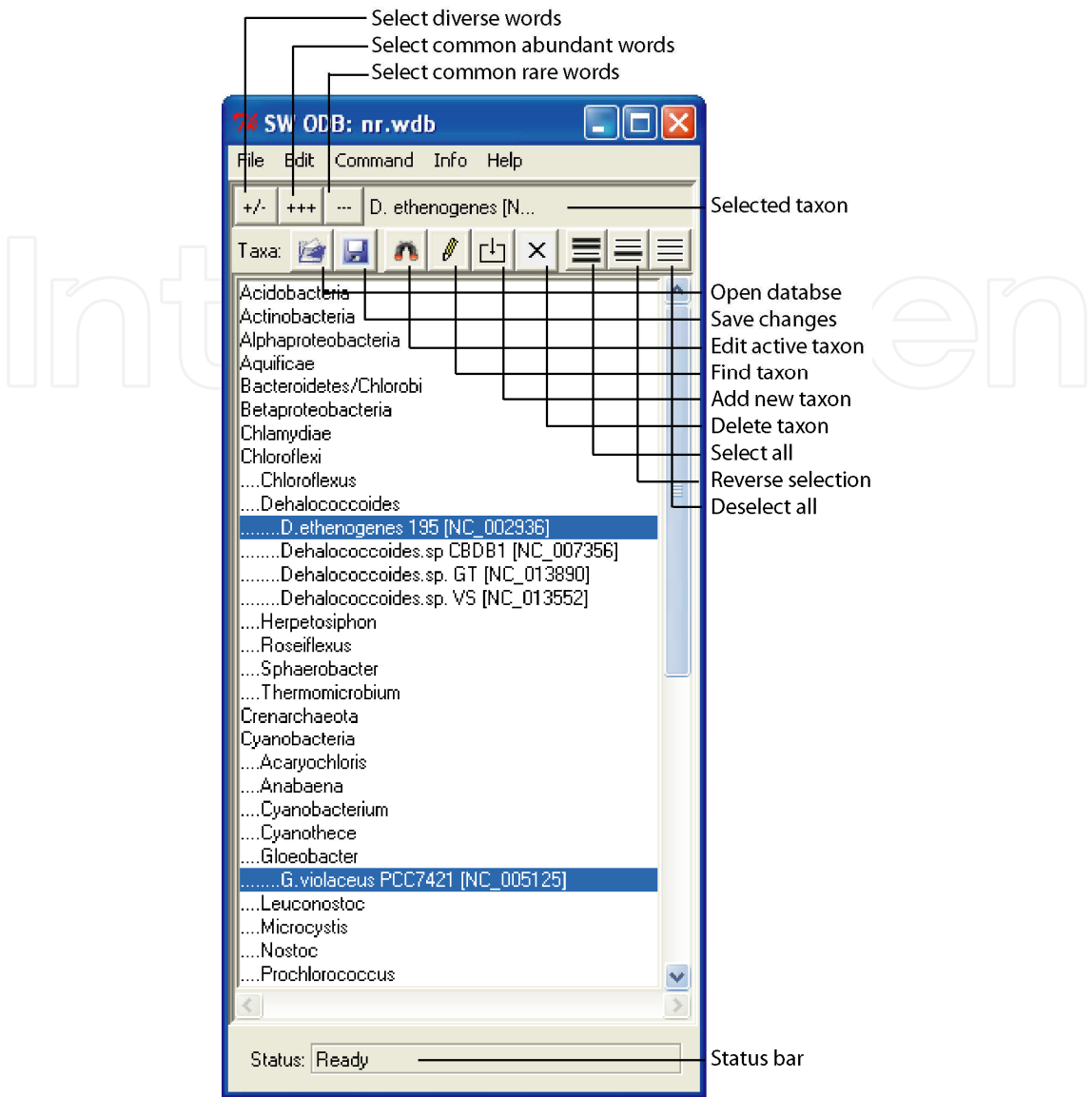
Fig. 5. The main window of OligoDBViewer.
