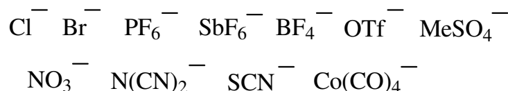
Fig. 2. Different anions that configure the ionic liquids.
