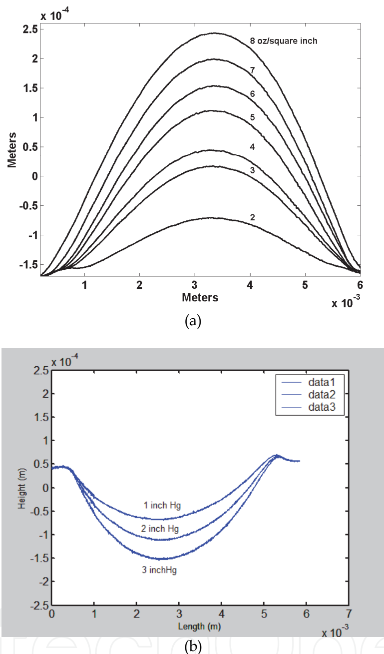
Fig. 12. Cell membranes reliefs measured with a surface analyzer. Parameter is the pressure. In (a) positive pressure was applied. In (b) negative pressure (vacuum) was applied.
