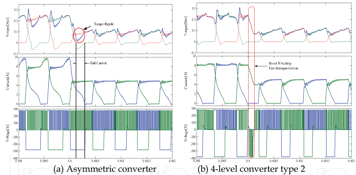
Fig. 25. Compared simulation results with reference variation.
