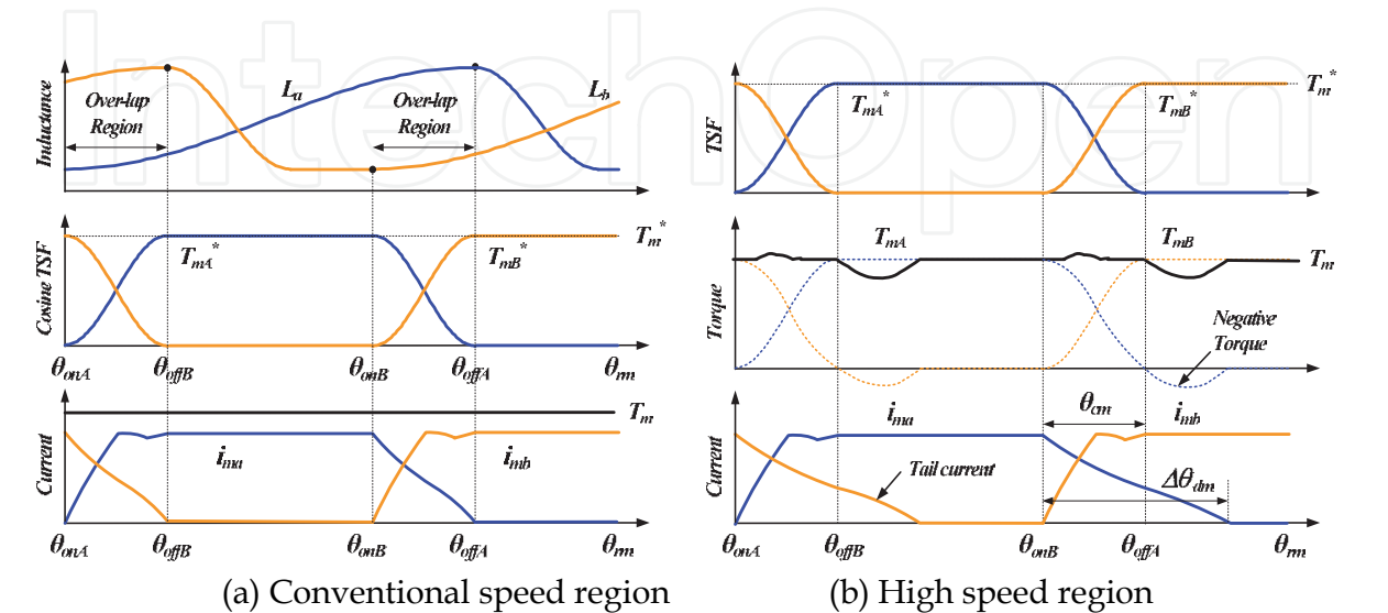
Fig. 26. Torque and current in TSF according to the speed.
