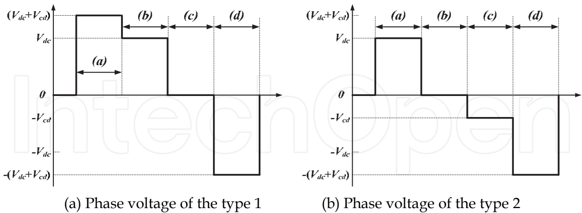
Fig. 21. Phase voltage of the 4-level converter. Fig. 22 shows current waveform of the 4-level converter type 1 and asymmetric one at 10,000[rpm] from experiment in a 12/8 SRM. As shown in Fig. 22, excitation current of the 4-level converter can support fast build-up and commutation of phase current when compared with a conventional asymmetric converter. Another approach using 4-level converter is DITC method. In the torque control, the additional control mode is very effective.
