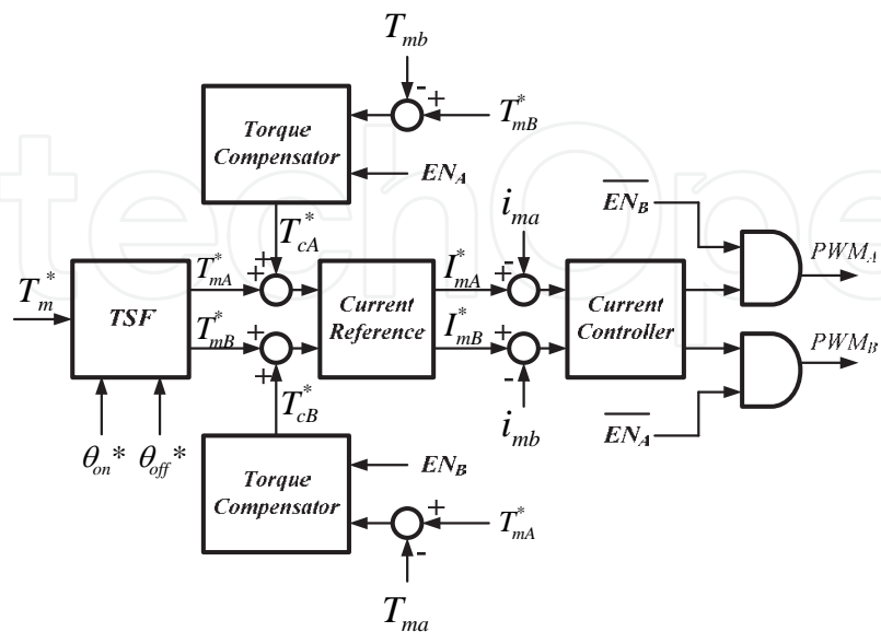
(b) Control block diagram
