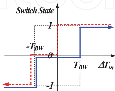
(b) Switching rule without PWM
