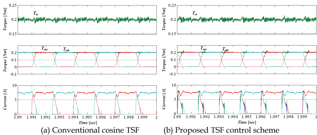
(a) Conventional cosine TSF (b) Proposed TSF control scheme Fig. 29. Compared simulation result at 10,000[rpm].
