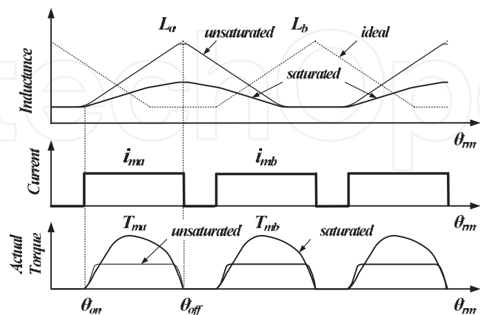
Fig. 8. Non-linear torque from the saturation effect.
