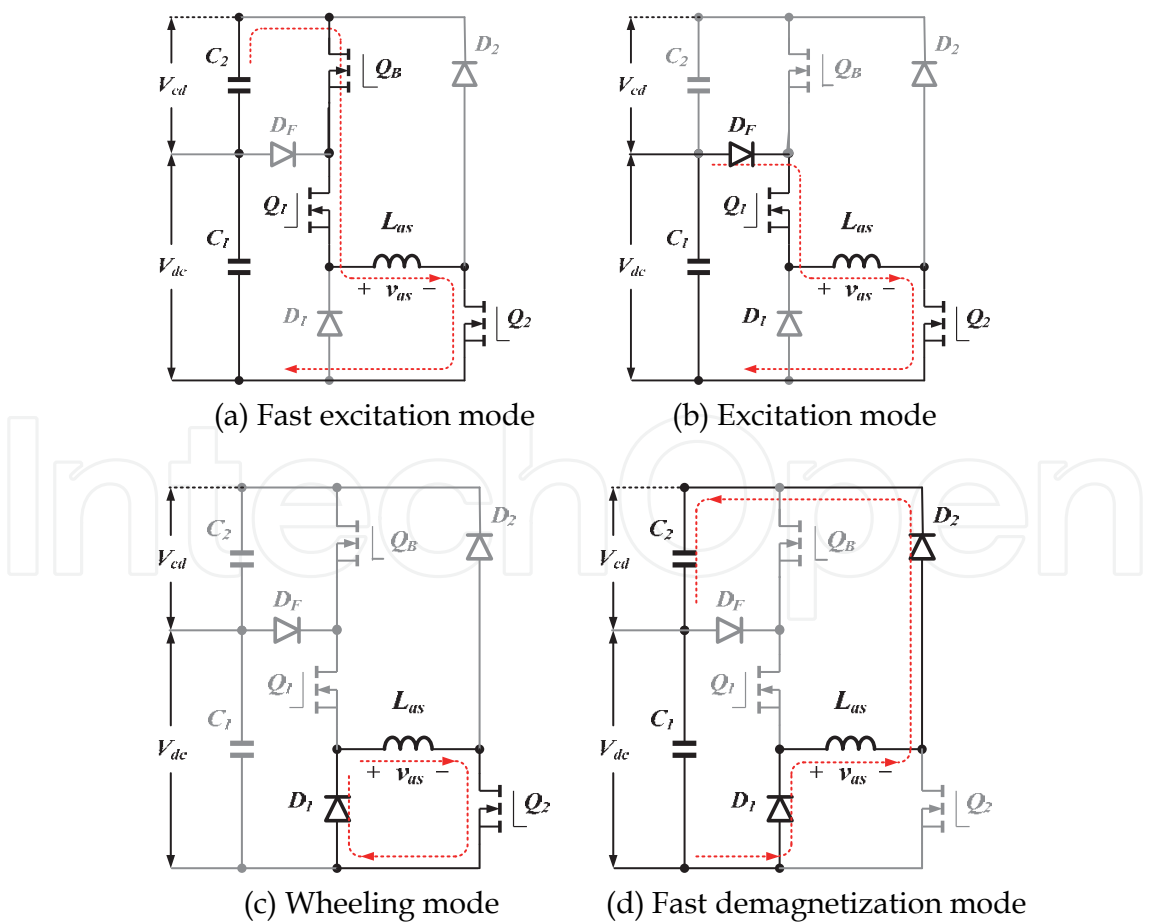
Fig. 19. Operating modes of the 4-level converter (type 1).
