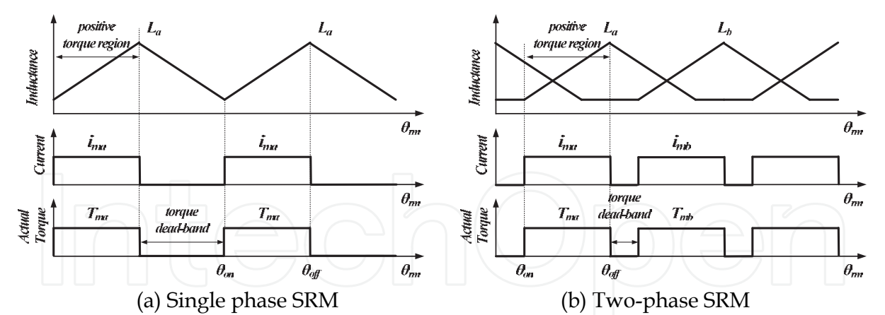
Fig. 6. Inductance, current and output torque of single and two-phase SRMs.
