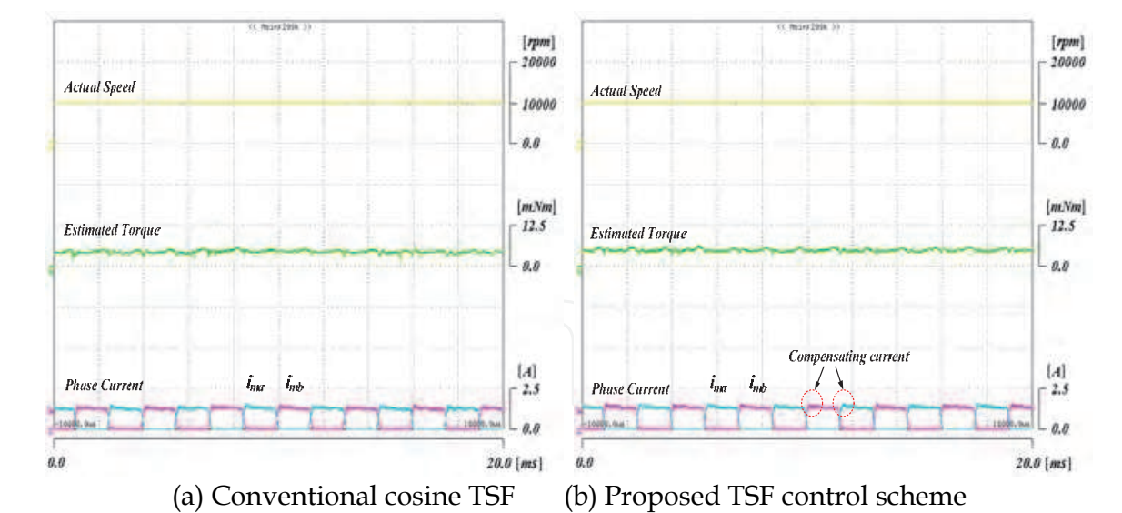
Fig. 31. Compared experimental results (At 10,000[rpm]).
