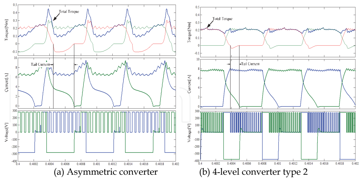
Fig. 24. Compared simulation results(30,000[rpm]).
