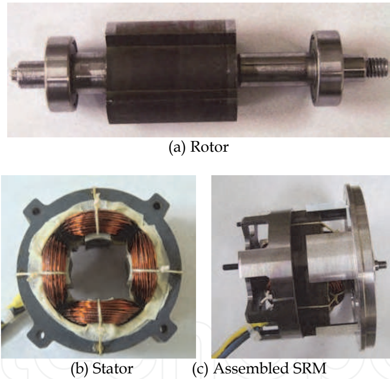
Fig. 23. Proto-type high speed 4/2 SRM.
