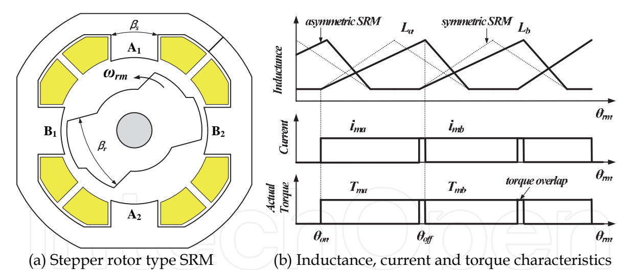
Fig. 7. Uni-directional 4/2 SRM with torque overlap.
