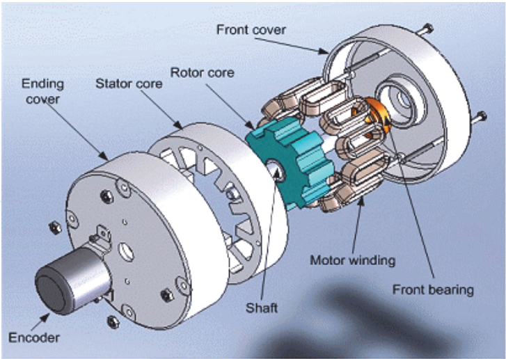
Fig. 4. The construction of SRM.
