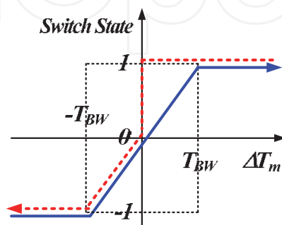
(c) Switching rule with PWM
