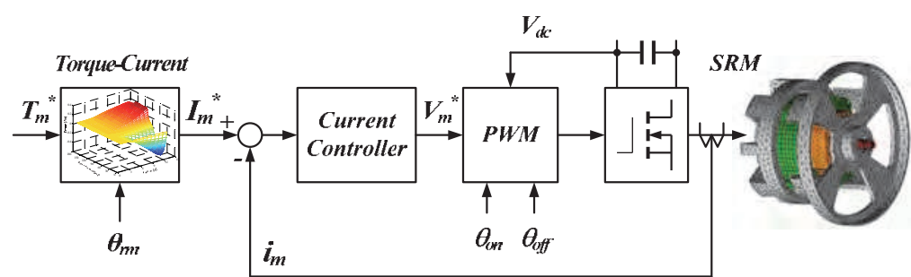
(a) Non-linear current control scheme
