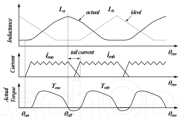
Fig. 9. Torque ripple from the tail current.
