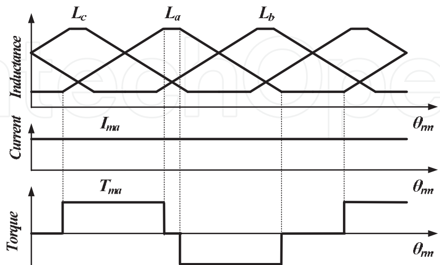
(b) Output torque vs phase current
