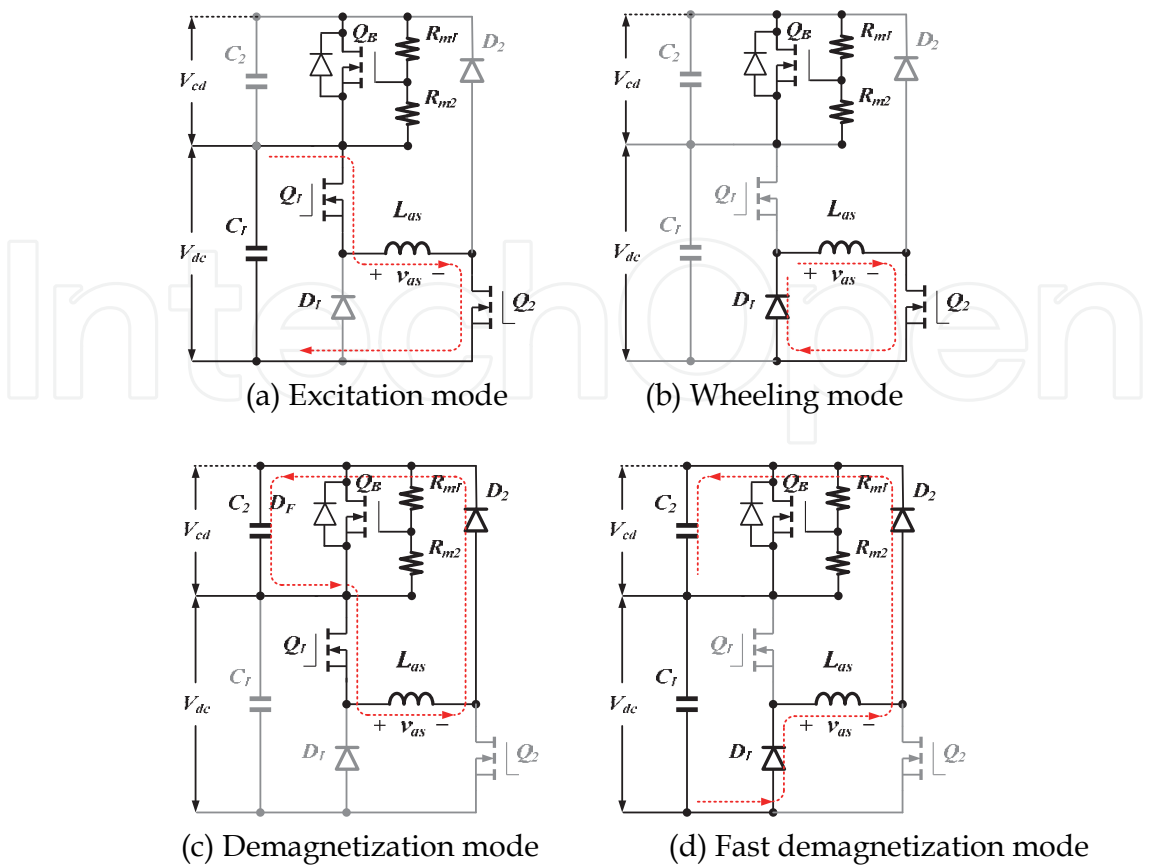
Fig. 20. Operating modes of the 4-level converter (type 2). With a PWM(Pulse Width Modulation) technology, two operating modes can be used in a sample time to control the phase current.
