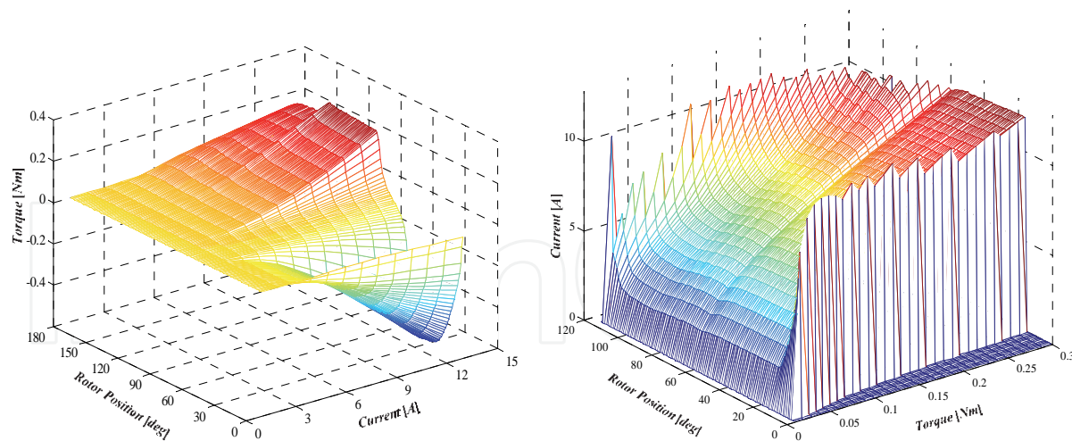
(a) Look-up table of the torque estimator (b) Look-up table of the current reference Fig. 28. The torque estimator and current reference of the proto-type SRM.
