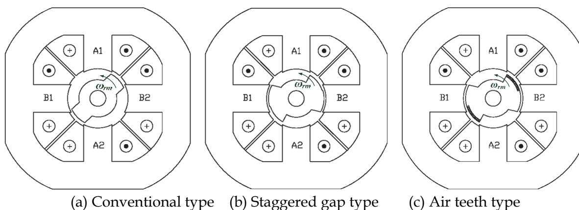
Fig. 3. Various type of 4/2 SRM.
