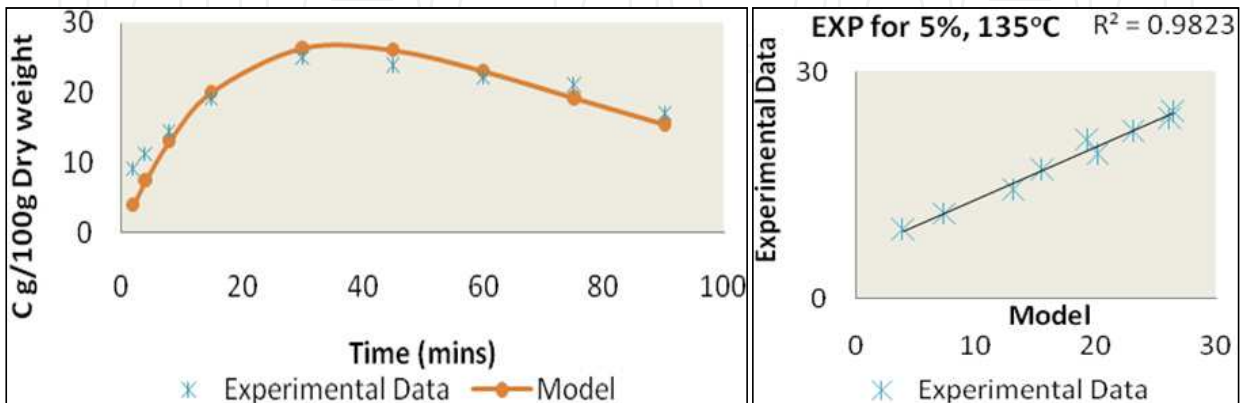
(a.1) Glucose model at 135°C, acid conc. 5.0%
