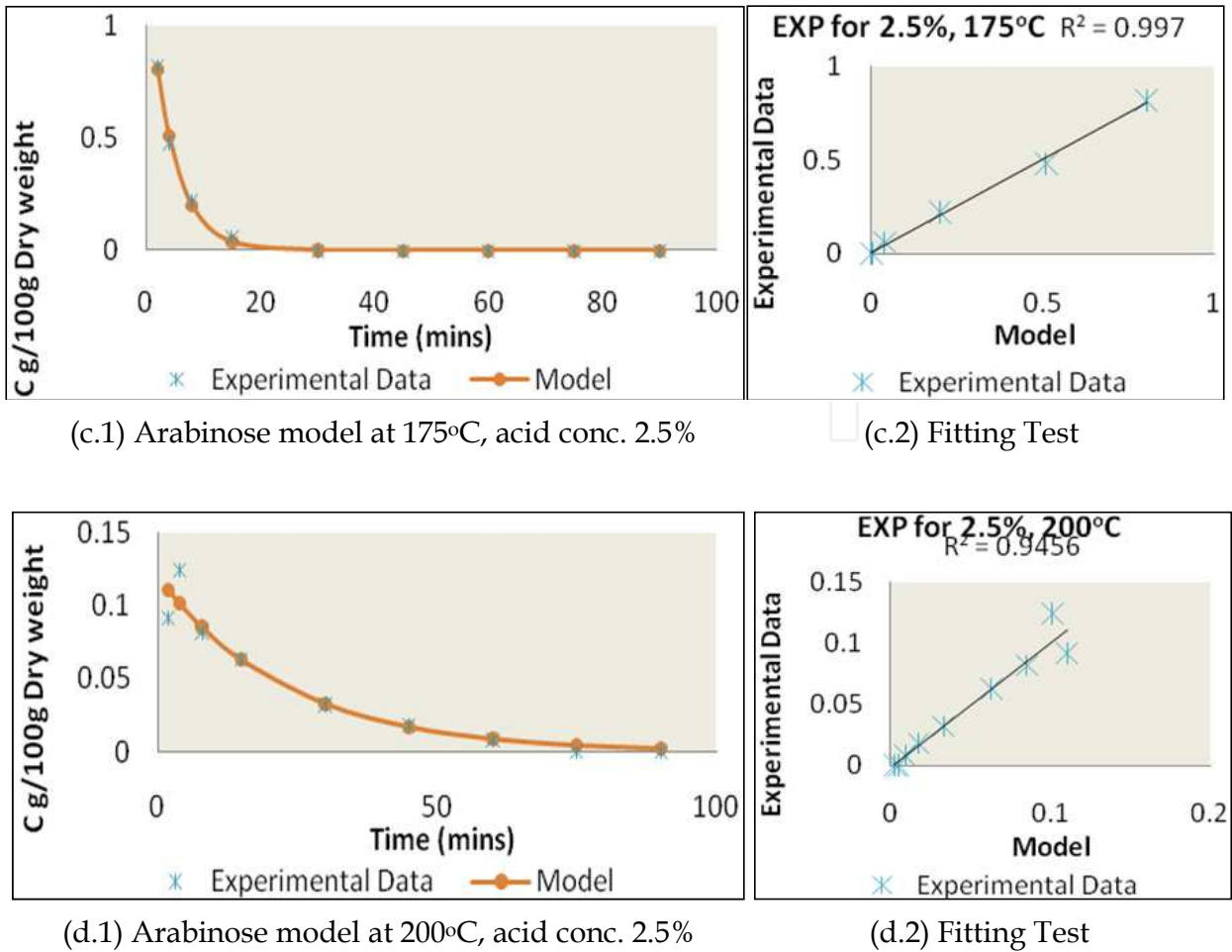
Fig. 3. Arabinose model with variation in reaction temperature
