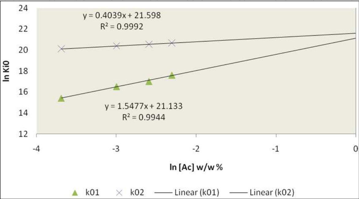
Fig. 5. The relationship between the calculated k_{i0} values and acid concentration for glucose The model for glucose was found to be more accurate than that of Arabinose due to issues with reliability of Arabinose experimental data obtained brought on by experimental/human error. The linear fit has a high accuracy level, indicated by the R^2 correlations obtained. This illustrates a strong agreement between acid concentration and the k_{i0} parameters. Table 3 shows the reaction constants obtained from Equation 12 for both sugars investigated.
