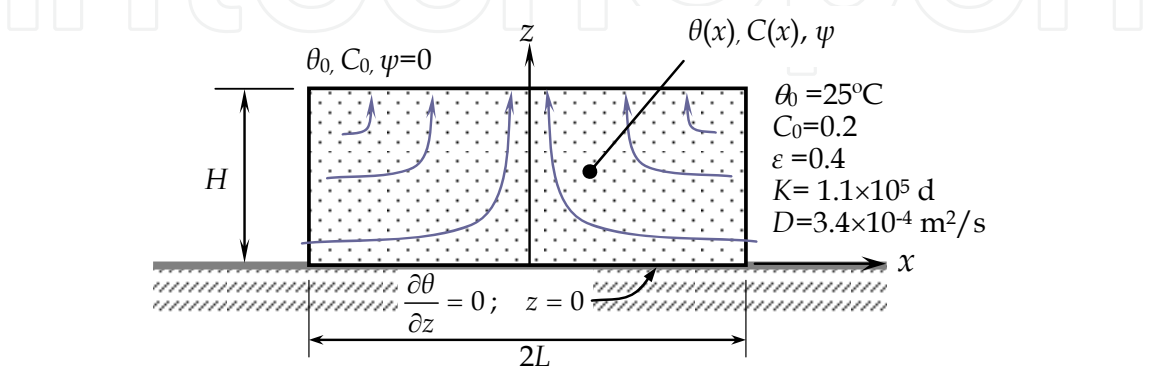
Fig. 14. Two-dimensional coal stockyard model with internal natural convection flow
