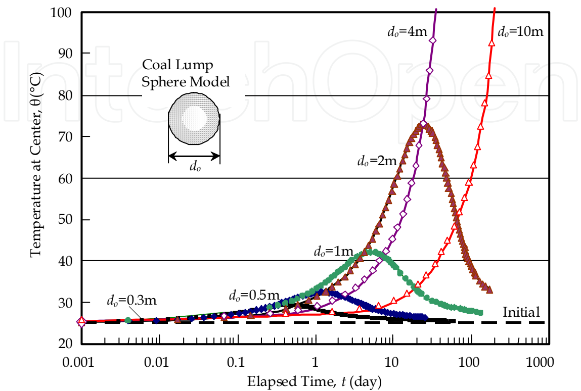
Fig. 7. Temperature at sphere center vs. elapsed time for different diameter
