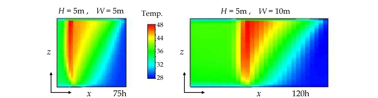
Fig. 18. Effect of aspect ratio, H/W , on temperature distribution in two-dimensional coal stock with internal natural convection flow ( 2W=10\text{m} , H=5\text{m} , K=1.1\times10^5\text{ d} , D=3.4\times10^{-4}\text{ m}^2/\text{s} )
