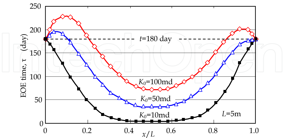
Fig. 12. Simulation results of EOE-time for different permeability of coal seam ( L=5\text{m} , \theta(0) = \theta(L) = 45^\circ\text{C} , t = 180\text{ days} , outer oxygen concentration, C(0) = C(L) = 0.20 )
