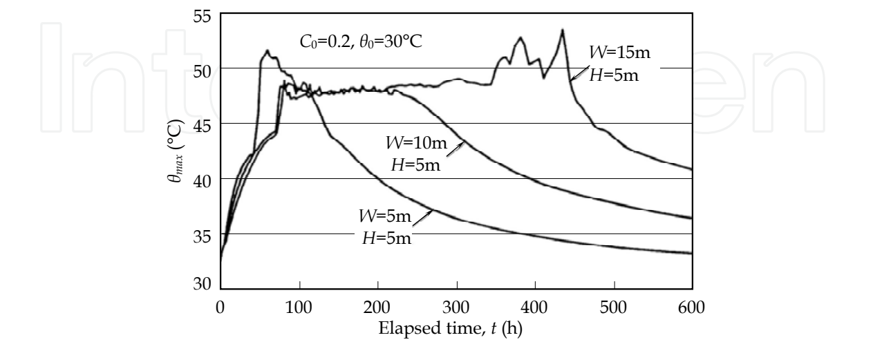
Fig. 19. Numerical simulation results of the maximum temperature transition in coal stock with three different aspect ratios
