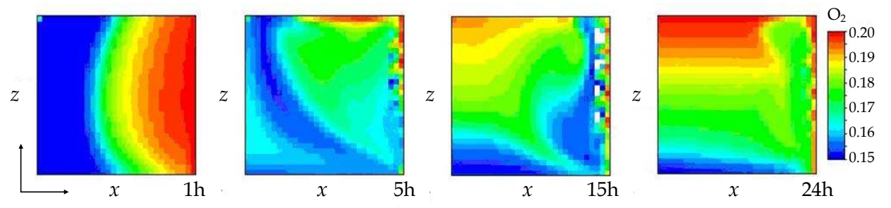
Fig. 17. Change of oxygen concentration distribution of two-dimensional coal stock (right half, 2W=10\text{m} , H=5\text{m} , K=1.1\times10^5\text{ d} , D=3.4\times10^{-4}\text{ m}^2/\text{s} ) with internal natural convection flow
