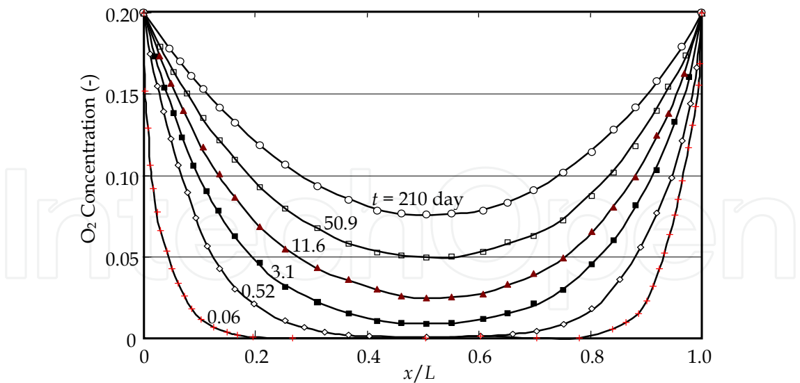
Fig. 13. Distributions of oxygen concentration in coal seam ( L=5\text{m} , \theta(0) = 45^{\circ}\text{C} , oxygen concentration, C(0) = C(L) = 0.20 , permeability K_0=50 \text{ md} = 4.9\times 10^{-14} \text{ m}^2 , D=7.1\times 10^{-6} \text{ m}^2/\text{s} )
