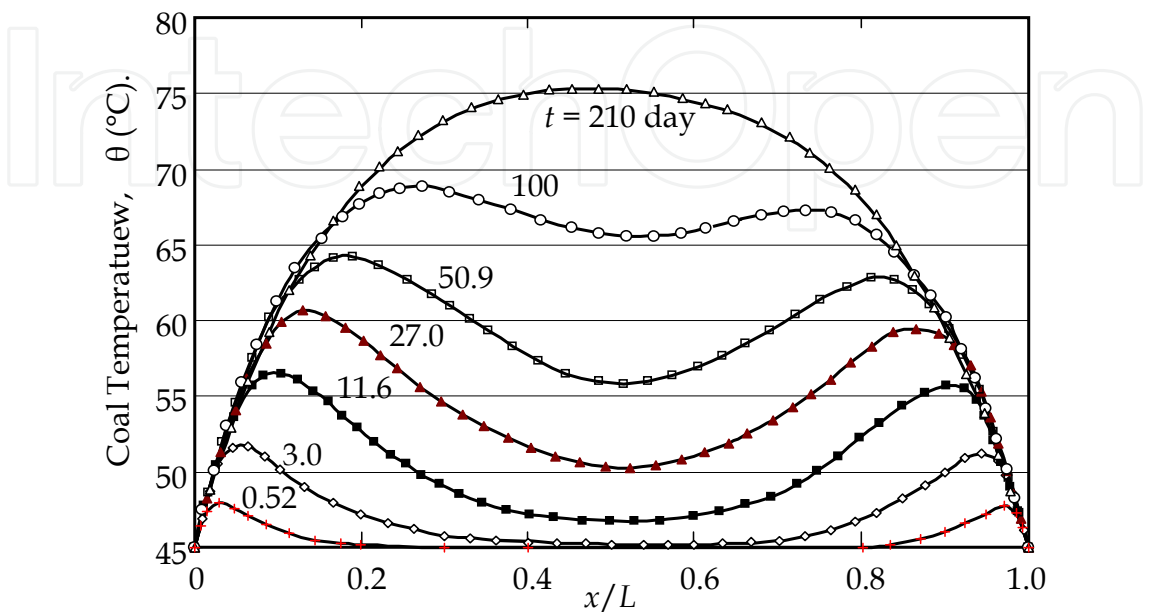
Fig. 11. Transition of temperature distribution of coal seam ( L=5\text{m} , Initial temperature, \theta(0) = \theta(L) = 45^\circ\text{C} , outer oxygen concentration, C(0) = C(L) = 0.20 , permeability K_0=50\text{ md} = 4.9\times 10^{-14}\text{ m}^2 , D=7.1\times 10^{-6}\text{ m}^2/\text{s} )
