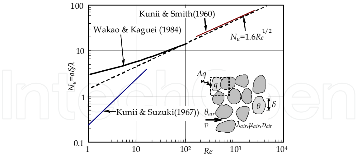
Fig. 15. Nusselt number, N_u vs. Reynolds number, Re=v\delta/v_{air} , in porous media consisting lump coals and air
