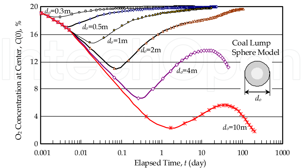
Fig. 8. Oxygen concentration at sphere center vs. elapsed time for different diameter
